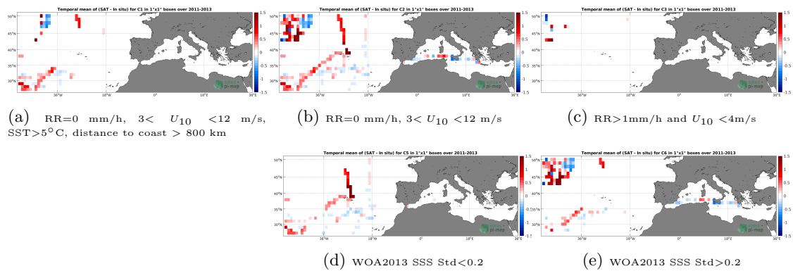
Figure 12: Temporal mean gridded over spatial boxes of size 1^\circ \times 1^\circ of \Delta SSS (SMOS SSS L3 MED-ATL-OA v2 - 9 Days (BEC) - TSG (SAMOS)) for 5 different subdatasets corresponding to: RR=0 mm/h, 3 < U_{10} < 12 m/s, SST > 5^\circ\text{C} , distance to coast > 800 km (a), RR=0 mm/h, 3 < U_{10} < 12 m/s (b), RR > 1 mm/h and U_{10} < 4 m/s (c), WOA2013 SSS Std < 0.2 (d), WOA2013 SSS Std > 0.2 (e).
