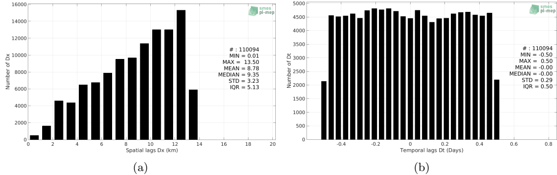
Figure 5: Histograms of the spatial (a) and temporal (b) lags between the time of the TSG (SAMOS) measurements and the date of the corresponding SMOS SSS L3 MED-ATL-OA v2 - 9 Days (BEC) SSS product.
