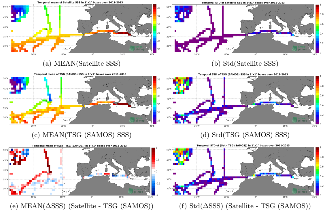
Figure 6: Temporal mean (left) and Std (right) of SSS from SMOS SSS L3 MED-ATL-OA v2 - 9 Days (BEC) (top), TSG (SAMOS) (middle), and of \Delta SSS (Satellite - TSG (SAMOS)). Only match-up pairs are used to generate these maps.
