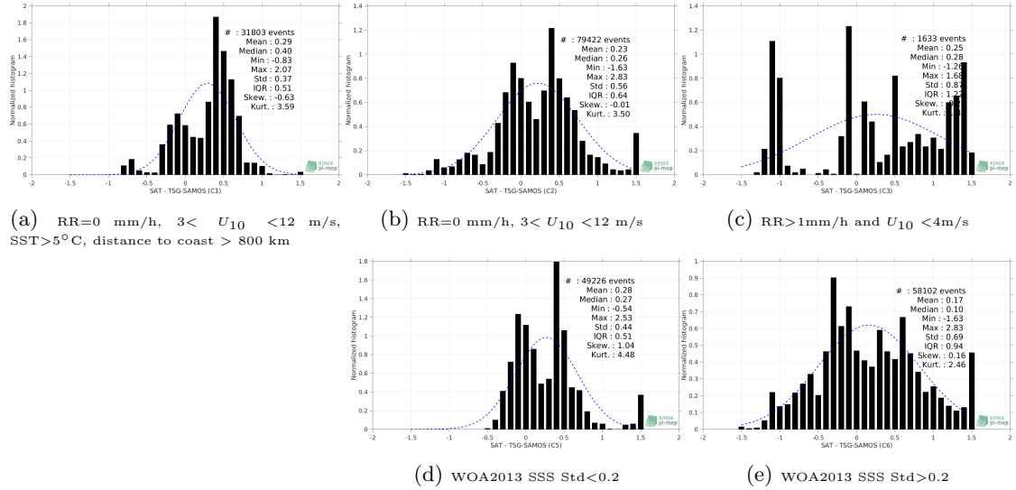
Figure 13: Normalized histogram of \Delta SSS (SMOS L3 MED-ATL-OA v2 - 9 Days (BEC) - TSG-SAMOS) for 5 different subdatasets corresponding to: RR=0 mm/h, 3 < U_{10} < 12 m/s, SST > 5°C, distance to coast > 800 km (a), RR=0 mm/h, 3 < U_{10} < 12 m/s (b), RR > 1mm/h and U_{10} < 4 m/s (c), WOA2013 SSS Std < 0.2 (d), WOA2013 SSS Std > 0.2 (e).
