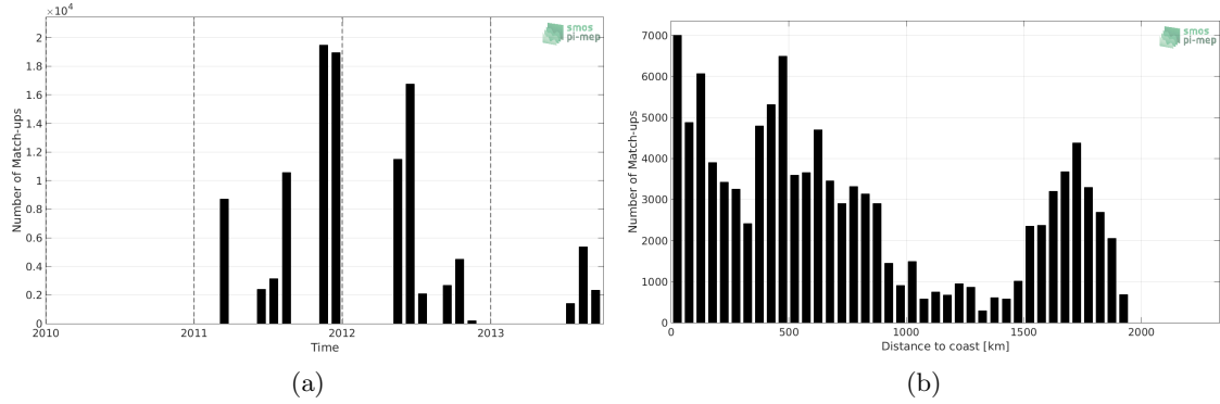
Figure 1: Number of match-ups between TSG-SAMOS and SMOS L3 MED-ATL-OA v2 - 9 Days (BEC) SSS as a function of time (a) and as function of the distance to coast (b) over the Global Ocean Pi-MEP region and for the full satellite product period.
