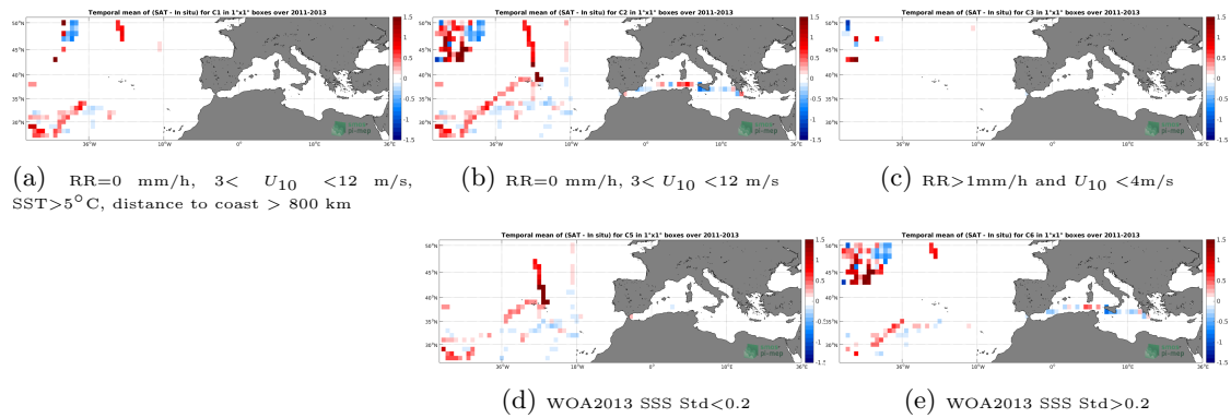
Figure 12: Temporal mean gridded over spatial boxes of size 1^\circ \times 1^\circ of \Delta SSS (SMOS L3 MED-ATL-OA v2 - 9 Days (BEC) - TSG-SAMOS) for 5 different subdatasets corresponding to:RR=0 mm/h, 3 < U_{10} < 12 m/s, SST >5^\circ\text{C} , distance to coast > 800 km (a), RR=0 mm/h, 3 < U_{10} < 12 m/s (b), RR >1 mm/h and U_{10} < 4 m/s (c), WOA2013 SSS Std <0.2 (d), WOA2013 SSS Std >0.2 (e).
