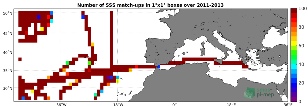
Figure 4: Number of SSS match-ups between TSG-SAMOS SSS and the SMOS L3 MED-ATL-OA v2 - 9 Days (BEC) SSS product for the Global Ocean Pi-MEP region over 1^\circ \times 1^\circ boxes and for the full satellite product period.
