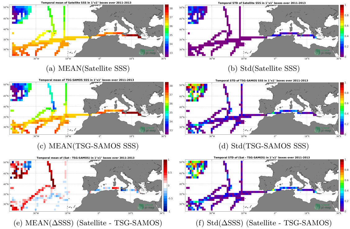
Figure 6: Temporal mean (left) and Std (right) of SSS from SMOS L3 MED-ATL-OA v2 - 9 Days (BEC) (top), TSG-SAMOS (middle), and of \Delta SSS (Satellite - TSG-SAMOS). Only match-up pairs are used to generate these maps.
