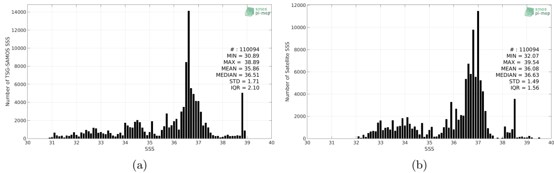
Figure 2: Histograms of SSS from TSG-SAMOS (a) and SMOS-L3-BEC-MED-ATL-OA-V2-9DAYS-0.25DEG (b) considering all match-up pairs per bins of 0.1 over the Global Ocean Pi-MEP region and for the full satellite product period.
