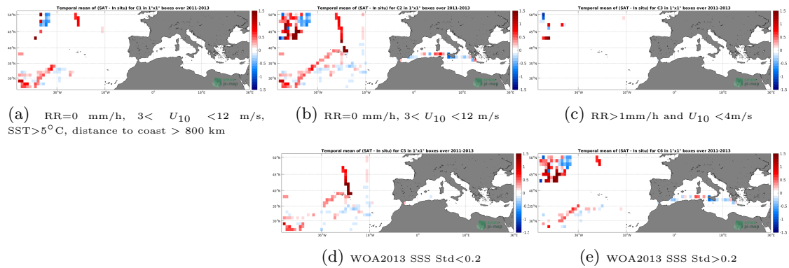
Figure 12: Temporal mean gridded over spatial boxes of size 1^\circ \times 1^\circ of \Delta SSS (SMOS-L3-BEC-MED-ATL-OA-V2-9DAYS-0.25DEG - TSG-SAMOS) for 5 different subdatasets corresponding to:RR=0 mm/h, 3 < U_{10} < 12 m/s, SST >5^\circ\text{C} , distance to coast > 800 km (a), RR=0 mm/h, 3 < U_{10} < 12 m/s (b), RR >1 mm/h and U_{10} < 4 m/s (c), WOA2013 SSS Std <0.2 (d), WOA2013 SSS Std >0.2 (e).
