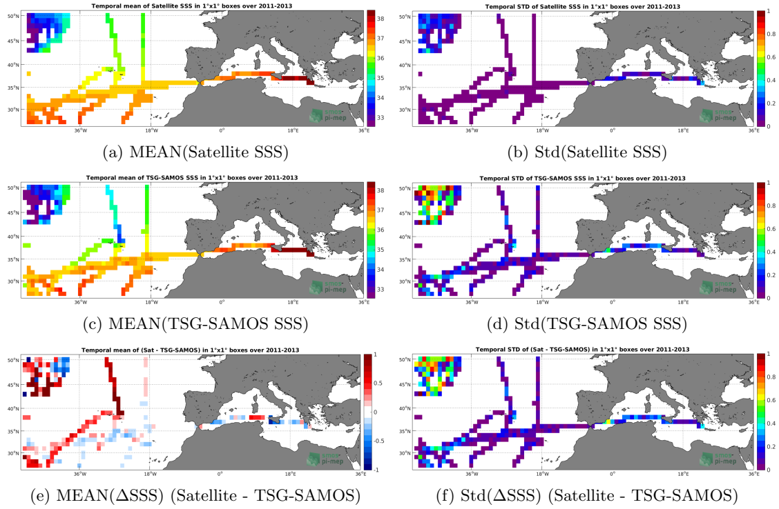
Figure 6: Temporal mean (left) and Std (right) of SSS from SMOS-L3-BEC-MED-ATL-OA-V2-9DAYS-0.25DEG (top), TSG-SAMOS (middle), and of \Delta SSS (Satellite - TSG-SAMOS). Only match-up pairs are used to generate these maps.
