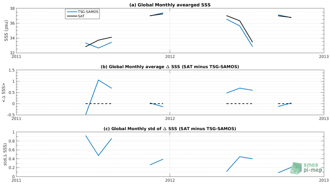
Figure 7: Time series of the monthly averaged mean SSS (top), mean \Delta \text{SSS} (Satellite - TSG-SAMOS) and Std of \Delta \text{SSS} (Satellite - TSG-SAMOS) over the Global Ocean Pi-MEP region considering all match-ups collected by the Pi-MEP platform.
