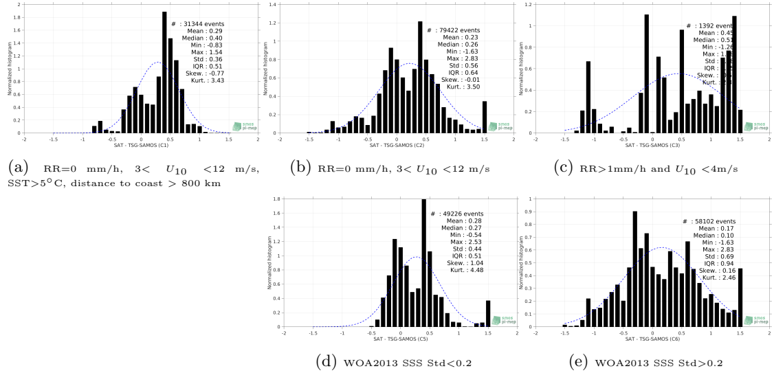
Figure 13: Normalized histogram of \Delta SSS (SMOS-L3-BEC-MED-ATL-OA-V2-9DAYS-0.25DEG - TSG-SAMOS) for 5 different subdatasets corresponding to: RR=0 mm/h, 3 < U_{10} < 12 m/s, SST>5°C, distance to coast > 800 km (a), RR=0 mm/h, 3 < U_{10} < 12 m/s (b), RR>1mm/h and U_{10} < 4 m/s (c), WOA2013 SSS Std<0.2 (d), WOA2013 SSS Std>0.2 (e).
