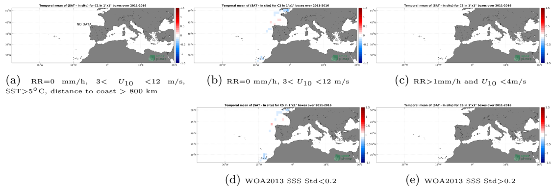
Figure 12: Temporal mean gridded over spatial boxes of size 1^\circ \times 1^\circ of \Delta SSS (SMOS SSS L3 MED-ATL-OA v2 - 9 Days (BEC) - TSG (Polarstern)) for 5 different subdatasets corresponding to:RR=0 mm/h, 3 < U_{10} < 12 m/s, SST >5^\circ C, distance to coast > 800 km (a), RR=0 mm/h, 3 < U_{10} < 12 m/s (b), RR >1 mm/h and U_{10} < 4 m/s (c), WOA2013 SSS Std <0.2 (d), WOA2013 SSS Std >0.2 (e).
