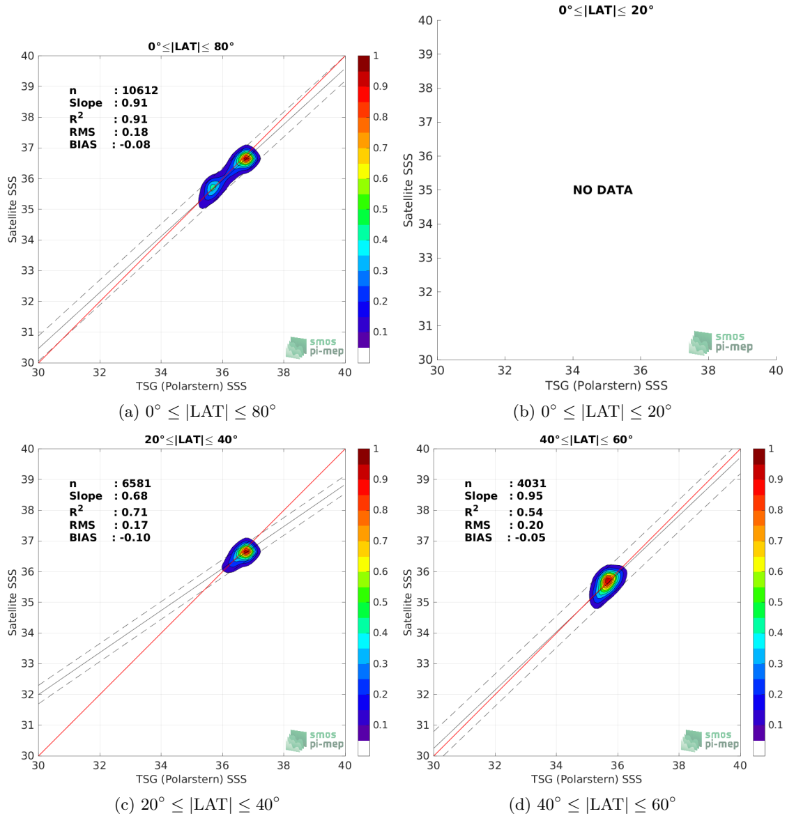
Figure 9: Contour maps of the concentration of SMOS SSS L3 MED-ATL-OA v2 - 9 Days (BEC) SSS (y-axis) versus TSG (Polarstern) SSS (x-axis) at match-up pairs for different latitude bands. For each plot, the red line shows x=y . The black thin and dashed lines indicate a linear fit through the data cloud and the \pm 95\% confidence levels, respectively. The number match-up pairs n , the slope and R^2 coefficient of the linear fit, the root mean square (RMS) and the mean bias between satellite and in situ data are indicated for each latitude band in each plots.
