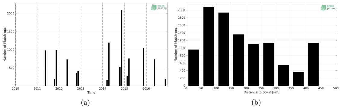
Figure 1: Number of match-ups between TSG (Polarstern) and SMOS SSS L3 MED-ATL-OA v2 - 9 Days (BEC) SSS as a function of time (a) and as function of the distance to coast (b) over the Global Ocean Pi-MEP region and for the full satellite product period.
