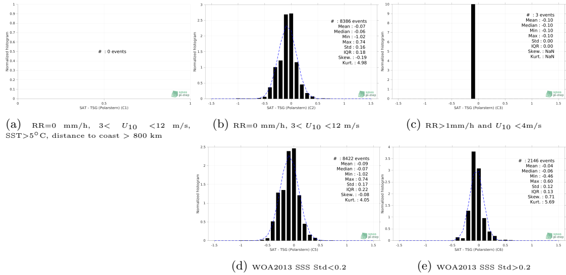
Figure 13: Normalized histogram of \Delta SSS (SMOS SSS L3 MED-ATL-OA v2 - 9 Days (BEC) - TSG (Polarstern)) for 5 different subdatasets corresponding to: RR=0 mm/h, 3 < U_{10} < 12 m/s, SST>5°C, distance to coast > 800 km (a), RR=0 mm/h, 3 < U_{10} < 12 m/s (b), RR>1mm/h and U_{10} < 4 m/s (c), WOA2013 SSS Std<0.2 (d), WOA2013 SSS Std>0.2 (e).
