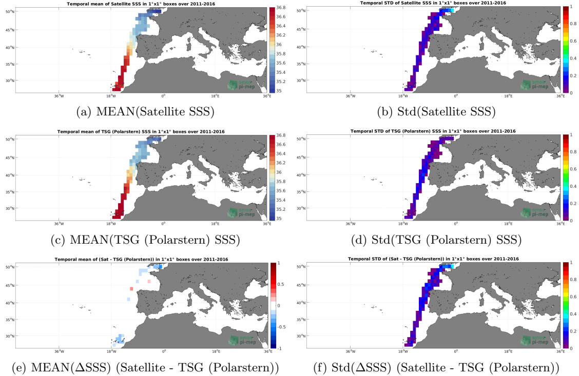
Figure 6: Temporal mean (left) and Std (right) of SSS from SMOS SSS L3 MED-ATL-OA v2 - 9 Days (BEC) (top), TSG (Polarstern) (middle), and of \Delta SSS (Satellite - TSG (Polarstern)). Only match-up pairs are used to generate these maps.
