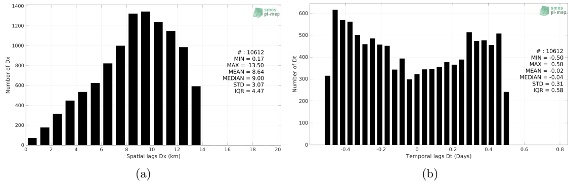
Figure 5: Histograms of the spatial (a) and temporal (b) lags between the location/time of the TSG (Polarstern) measurement and the date of the corresponding SMOS SSS L3 MED-ATL-OA v2 - 9 Days (BEC) SSS pixel.
