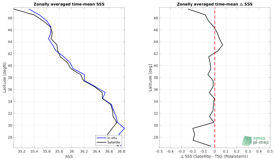
Figure 8: Left panel: Zonal mean SSS from SMOS SSS L3 MED-ATL-OA v2 - 9 Days (BEC) satellite product (black) and from TSG (Polarstern) (blue). Right panel: Zonal mean of \Delta SSS (Satellite - TSG (Polarstern)) for all the collected Pi-MEP match-up pairs estimated over the full satellite product period.
