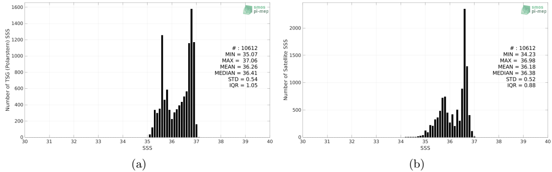
Figure 2: Histograms of SSS from TSG (Polarstern) (a) and SMOS SSS L3 MED-ATL-OA v2 - 9 Days (BEC) (b) considering all match-up pairs per bins of 0.1 over the Global Ocean Pi-MEP region and for the full satellite product period.
