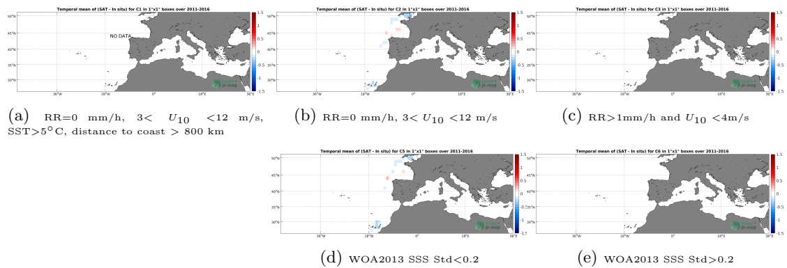
Figure 12: Temporal mean gridded over spatial boxes of size 1^\circ \times 1^\circ of \Delta SSS (SMOS SSS L3 MED-ATL-OA v2 - 9 Days (BEC) - TSG (Polarstern)) for 5 different subdatasets corresponding to:RR=0 mm/h, 3 < U_{10} < 12 m/s, SST >5^\circ C, distance to coast > 800 km (a), RR=0 mm/h, 3 < U_{10} < 12 m/s (b), RR >1 mm/h and U_{10} < 4 m/s (c), WOA2013 SSS Std <0.2 (d), WOA2013 SSS Std >0.2 (e).
