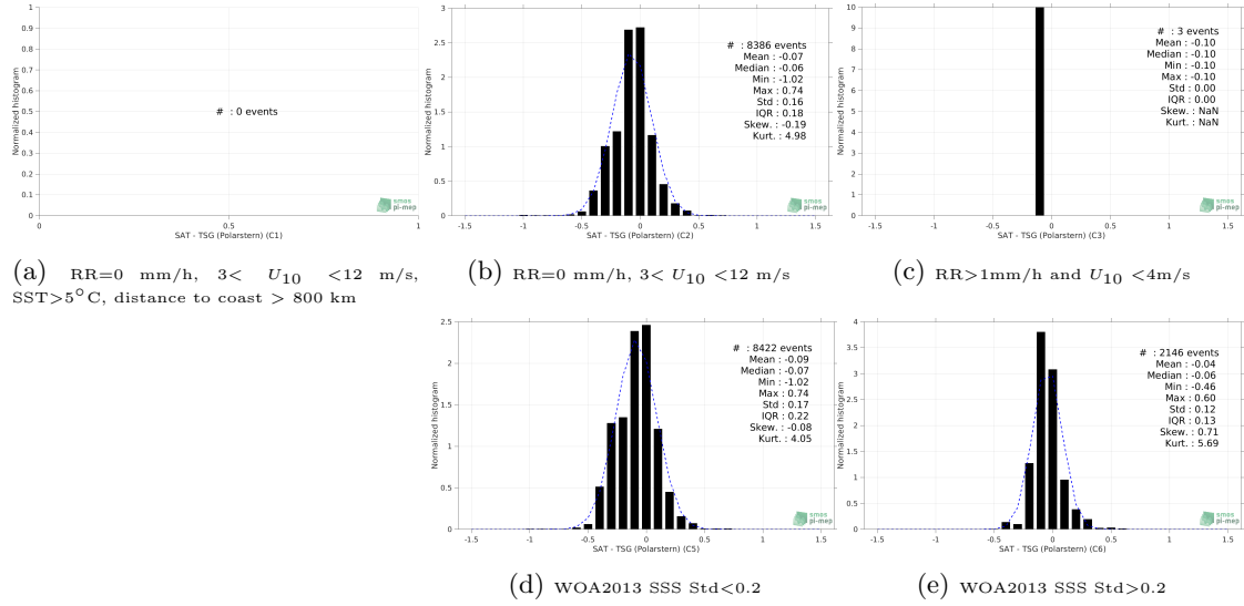
Figure 13: Normalized histogram of \Delta\text{SSS} (SMOS SSS L3 MED-ATL-OA v2 - 9 Days (BEC) - TSG (Polarstern)) for 5 different subdatasets corresponding to: RR=0 mm/h, 3 < U_{10} < 12 m/s, SST > 5^\circ\text{C} , distance to coast > 800 km (a), RR=0 mm/h, 3 < U_{10} < 12 m/s (b), RR > 1\text{mm/h} and U_{10} < 4\text{m/s} (c), WOA2013 SSS Std < 0.2 (d), WOA2013 SSS Std > 0.2 (e).
