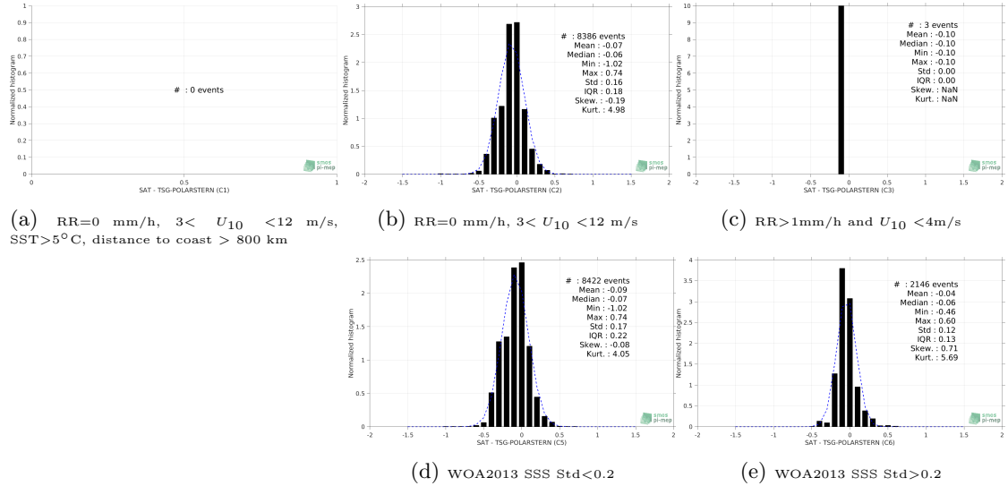
Figure 13: Normalized histogram of \Delta SSS (SMOS-L3-BEC-MED-ATL-OA-V2-9DAYS-0.25DEG - TSG-POLARSTERN) for 5 different subdatasets corresponding to: RR=0 mm/h, 3 < U_{10} < 12 m/s, SST > 5°C, distance to coast > 800 km (a), RR=0 mm/h, 3 < U_{10} < 12 m/s (b), RR > 1mm/h and U_{10} < 4 m/s (c), WOA2013 SSS Std < 0.2 (d), WOA2013 SSS Std > 0.2 (e).
