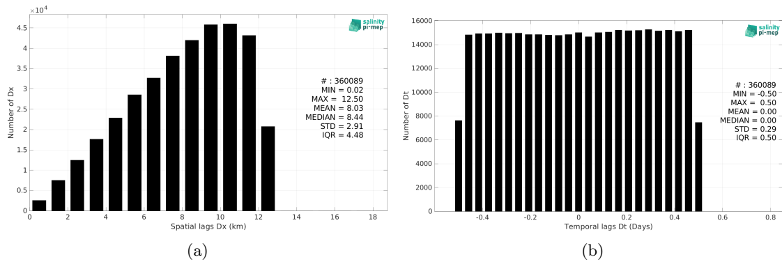
Figure 6: Histograms of the spatial (a) and temporal (b) lags between the location/time of the TSG (LEGOS-DM) measurement and the date of the corresponding SMOS SSS L3 MED-ATL-OA v2 - 9 Days (BEC) SSS pixel.
