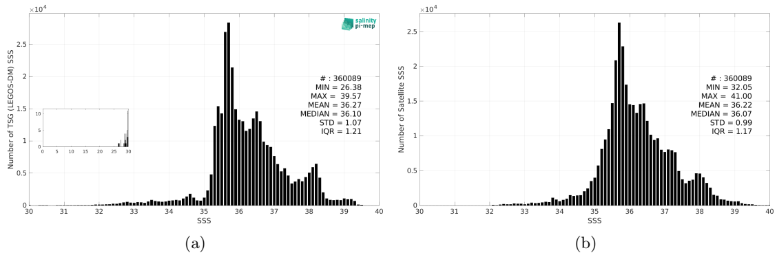
Figure 3: Histograms of SSS from TSG (LEGOS-DM) (a) and SMOS SSS L3 MED-ATL-OA v2 - 9 Days (BEC) (b) considering all match-up pairs per bins of 0.1 over the Global Ocean Pi-MEP region and for the full satellite product period.
