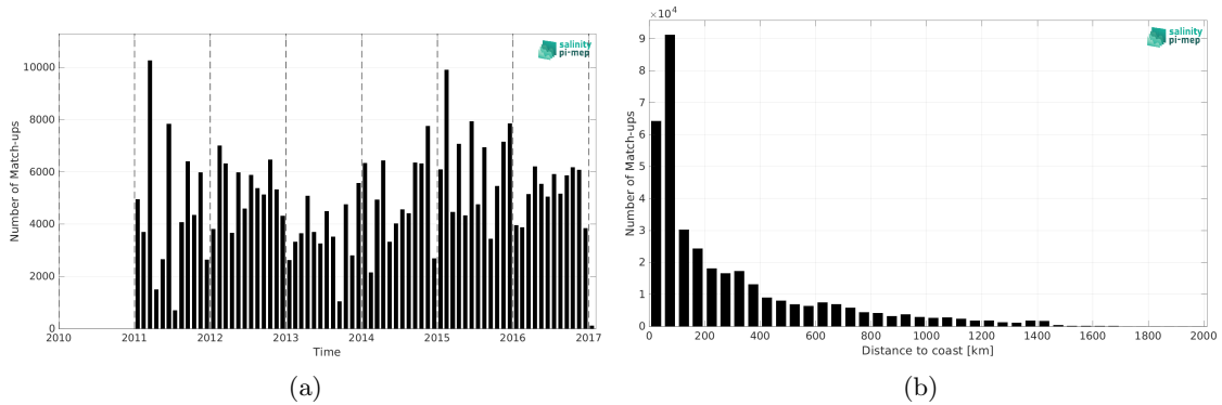
Figure 2: Number of match-ups between TSG (LEGOS-DM) and SMOS SSS L3 MED-ATL-OA v2 - 9 Days (BEC) SSS as a function of time (a) and as function of the distance to coast (b) over the Global Ocean Pi-MEP region and for the full satellite product period.
