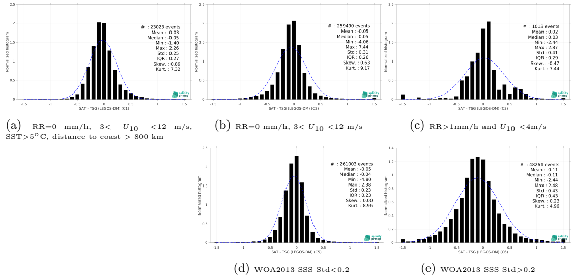
Figure 15: Normalized histogram of \Delta\text{SSS} (SMOS SSS L3 MED-ATL-OA v2 - 9 Days (BEC) - TSG (LEGOS-DM)) for 5 different subdatasets corresponding to: RR=0 mm/h, 3 < U_{10} < 12 m/s, SST>5°C, distance to coast > 800 km (a), RR=0 mm/h, 3 < U_{10} < 12 m/s (b), RR>1mm/h and U_{10} < 4 m/s (c), WOA2013 SSS Std<0.2 (d), WOA2013 SSS Std>0.2 (e).
