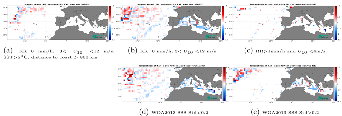
Figure 14: Temporal mean gridded over spatial boxes of size 1^\circ \times 1^\circ of \Delta SSS (SMOS SSS L3 MED-ATL-OA v2 - 9 Days (BEC) - TSG (LEGOS-DM)) for 5 different subdatasets corresponding to:RR=0 mm/h, 3 < U_{10} < 12 m/s, SST >5^\circ\text{C} , distance to coast > 800 km (a), RR=0 mm/h, 3 < U_{10} < 12 m/s (b), RR >1 mm/h and U_{10} < 4 m/s (c), WOA2013 SSS Std <0.2 (d), WOA2013 SSS Std >0.2 (e).
