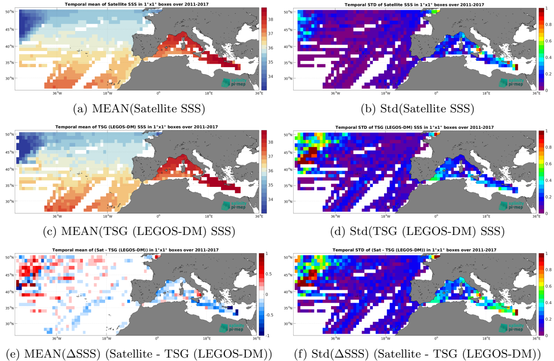
Figure 7: Temporal mean (left) and Std (right) of SSS from SMOS SSS L3 MED-ATL-OA v2 - 9 Days (BEC) (top), TSG (LEGOS-DM) (middle), and of \Delta SSS (Satellite - TSG (LEGOS-DM)). Only match-up pairs are used to generate these maps.
