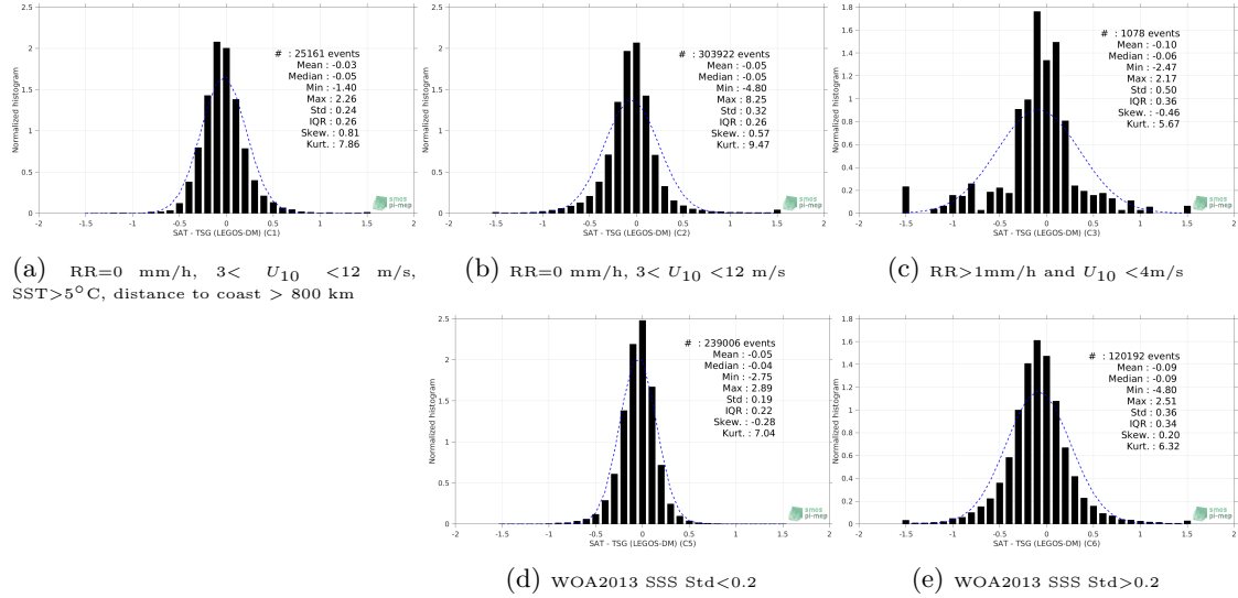
Figure 13: Normalized histogram of \Delta SSS (SMOS SSS L3 MED-ATL-OA v2 - 9 Days (BEC) - TSG (LEGOS-DM)) for 5 different subdatasets corresponding to: RR=0 mm/h, 3 < U_{10} < 12 m/s, SST>5°C, distance to coast > 800 km (a), RR=0 mm/h, 3 < U_{10} < 12 m/s, SST>5°C, distance to coast > 800 km (a), RR=0 mm/h, 3 < U_{10} < 12 m/s (b), RR>1mm/h and U_{10} < 4 m/s (c), WOA2013 SSS Std<0.2 (d), WOA2013 SSS Std>0.2 (e).
