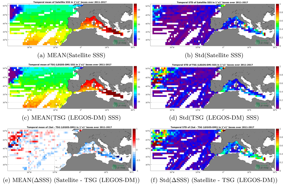
Figure 6: Temporal mean (left) and Std (right) of SSS from SMOS SSS L3 MED-ATL-OA v2 - 9 Days (BEC) (top), TSG (LEGOS-DM) (middle), and of \Delta SSS (Satellite - TSG (LEGOS-DM)). Only match-up pairs are used to generate these maps.
