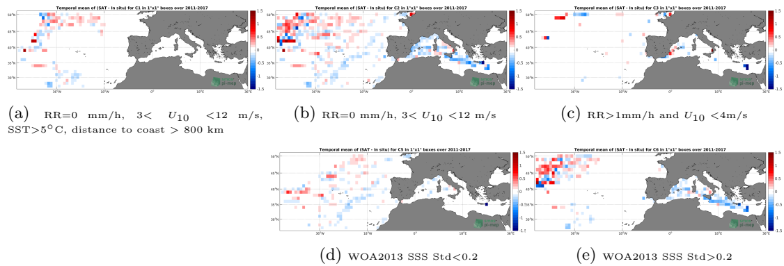
Figure 12: Temporal mean gridded over spatial boxes of size 1^\circ \times 1^\circ of \Delta\text{SSS} (SMOS SSS L3 MED-ATL-OA v2 - 9 Days (BEC) - TSG (LEGOS-DM)) for 5 different subdatasets corresponding to:RR=0 mm/h, 3 < U_{10} < 12 m/s, SST >5^\circ\text{C} , distance to coast > 800 km (a), RR=0 mm/h, 3 < U_{10} < 12 m/s (b), RR >1 mm/h and U_{10} < 4 m/s (c), WOA2013 SSS Std <0.2 (d), WOA2013 SSS Std >0.2 (e).
