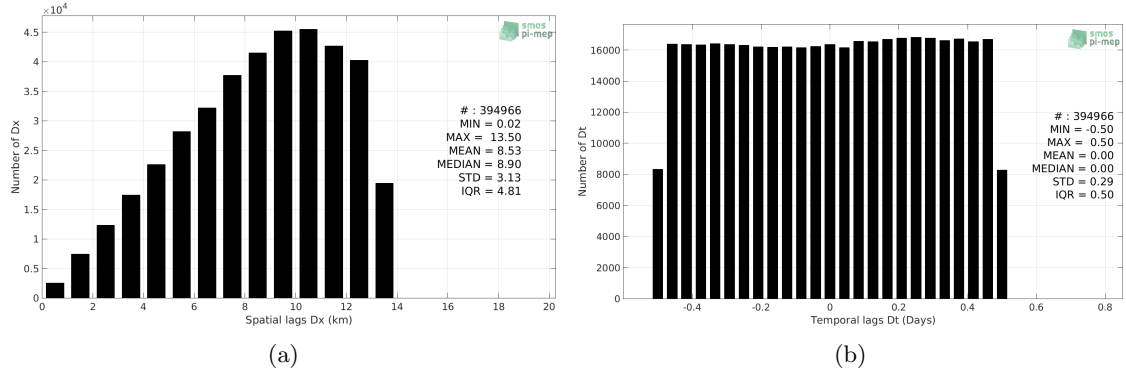
Figure 5: Histograms of the spatial (a) and temporal (b) lags between the location/time of the TSG (LEGOS-DM) measurement and the date of the corresponding SMOS SSS L3 MED-ATL-OA v2 - 9 Days (BEC) SSS pixel.
