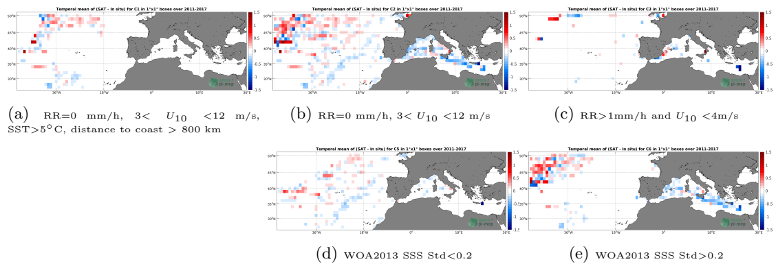
Figure 12: Temporal mean gridded over spatial boxes of size 1^\circ \times 1^\circ of \Delta SSS (SMOS SSS L3 MED-ATL-OA v2 - 9 Days (BEC) - TSG (LEGOS-DM)) for 5 different subdatasets corresponding to: RR=0 mm/h, 3 < U_{10} < 12 m/s, SST > 5°C, distance to coast > 800 km (a), RR=0 mm/h, 3 < U_{10} < 12 m/s (b), RR > 1mm/h and U_{10} < 4 m/s (c), WOA2013 SSS Std < 0.2 (d), WOA2013 SSS Std > 0.2 (e).
