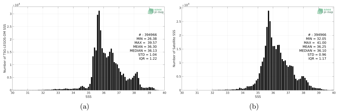
Figure 2: Histograms of SSS from TSG-LEGOS-DM (a) and SMOS L3 MED-ATL-OA v2 - 9 Days (BEC) (b) considering all match-up pairs per bins of 0.1 over the Global Ocean Pi-MEP region and for the full satellite product period.
