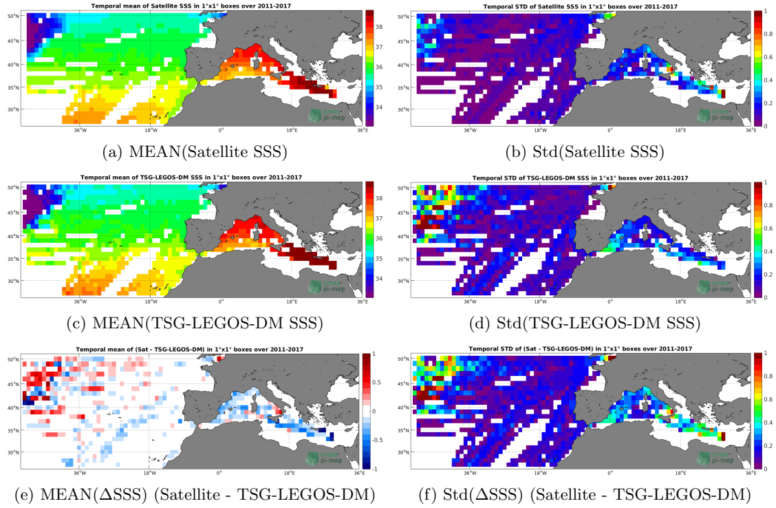
Figure 6: Temporal mean (left) and Std (right) of SSS from SMOS L3 MED-ATL-OA v2 - 9 Days (BEC) (top), TSG-LEGOS-DM (middle), and of \Delta SSS (Satellite - TSG-LEGOS-DM). Only match-up pairs are used to generate these maps.
