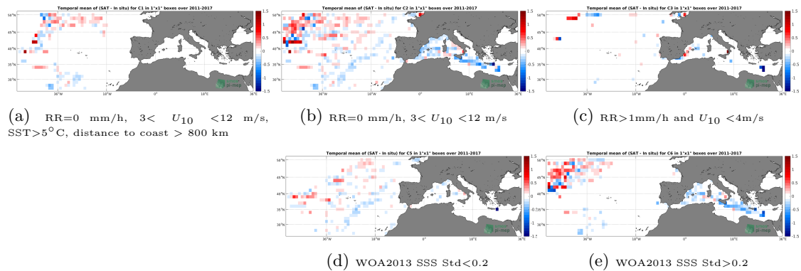
Figure 12: Temporal mean gridded over spatial boxes of size 1^\circ \times 1^\circ of \Delta SSS (SMOS L3 MED-ATL-OA v2 - 9 Days (BEC) - TSG-LEGOS-DM) for 5 different subdatasets corresponding to:RR=0 mm/h, 3 < U_{10} < 12 m/s, SST >5^\circ\text{C} , distance to coast > 800 km (a), RR=0 mm/h, 3 < U_{10} < 12 m/s (b), RR >1 mm/h and U_{10} < 4 m/s (c), WOA2013 SSS Std <0.2 (d), WOA2013 SSS Std >0.2 (e).
