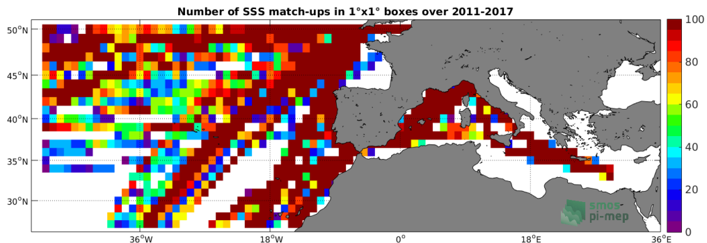
Figure 4: Number of SSS match-ups between TSG-LEGOS-DM SSS and the SMOS L3 MED-ATL-OA v2 - 9 Days (BEC) SSS product for the Global Ocean Pi-MEP region over 1^\circ \times 1^\circ boxes and for the full satellite product period.
