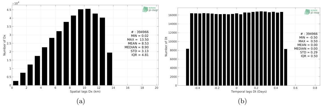
Figure 5: Histograms of the spatial (a) and temporal (b) lags between the time of the TSG-LEGOS-DM measurements and the date of the corresponding SMOS-L3-BEC-MED-ATL-OA-V2-9DAYS-0.25DEG SSS product.
