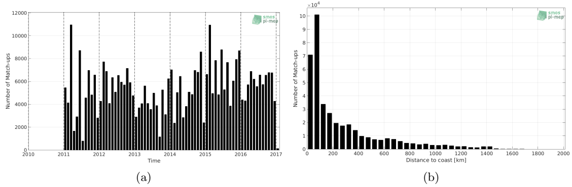
Figure 1: Number of match-ups between TSG-LEGOS-DM and SMOS-L3-BEC-MED-ATL-OA-V2-9DAYS-0.25DEG SSS as a function of time (a) and as function of the distance to coast (b) over the Global Ocean Pi-MEP region and for the full satellite product period.
