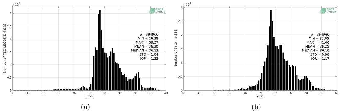
Figure 2: Histograms of SSS from TSG-LEGOS-DM (a) and SMOS-L3-BEC-MED-ATL-OA-V2-9DAYS-0.25DEG (b) considering all match-up pairs per bins of 0.1 over the Global Ocean Pi-MEP region and for the full satellite product period.
