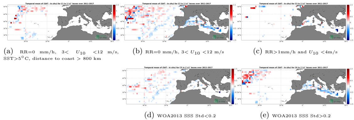
Figure 12: Temporal mean gridded over spatial boxes of size 1^\circ \times 1^\circ of \Delta SSS (SMOS-L3-BEC-MED-ATL-OA-V2-9DAYS-0.25DEG - TSG-LEGOS-DM) for 5 different subdatasets corresponding to:RR=0 mm/h, 3 < U_{10} < 12 m/s, SST >5^\circ\text{C} , distance to coast > 800 km (a), RR=0 mm/h, 3 < U_{10} < 12 m/s (b), RR >1 mm/h and U_{10} < 4 m/s (c), WOA2013 SSS Std <0.2 (d), WOA2013 SSS Std >0.2 (e).
