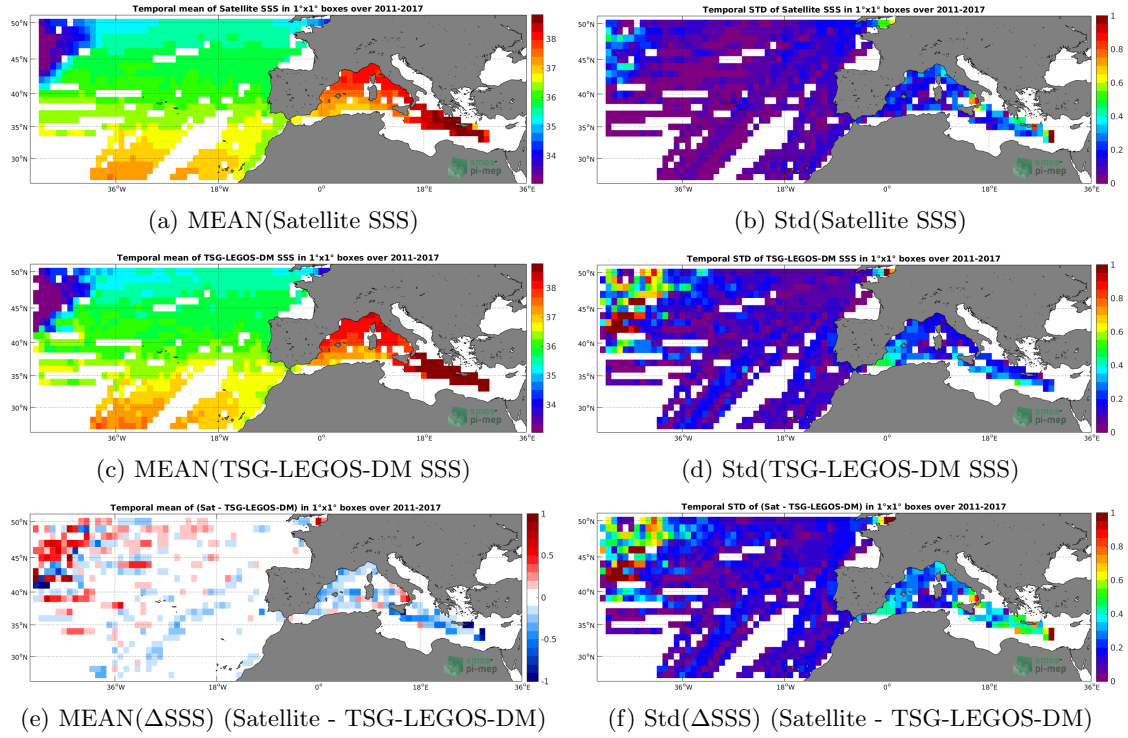
Figure 6: Temporal mean (left) and Std (right) of SSS from SMOS-L3-BEC-MED-ATL-OA-V2-9DAYS-0.25DEG (top), TSG-LEGOS-DM (middle), and of \Delta SSS (Satellite - TSG-LEGOS-DM). Only match-up pairs are used to generate these maps.
