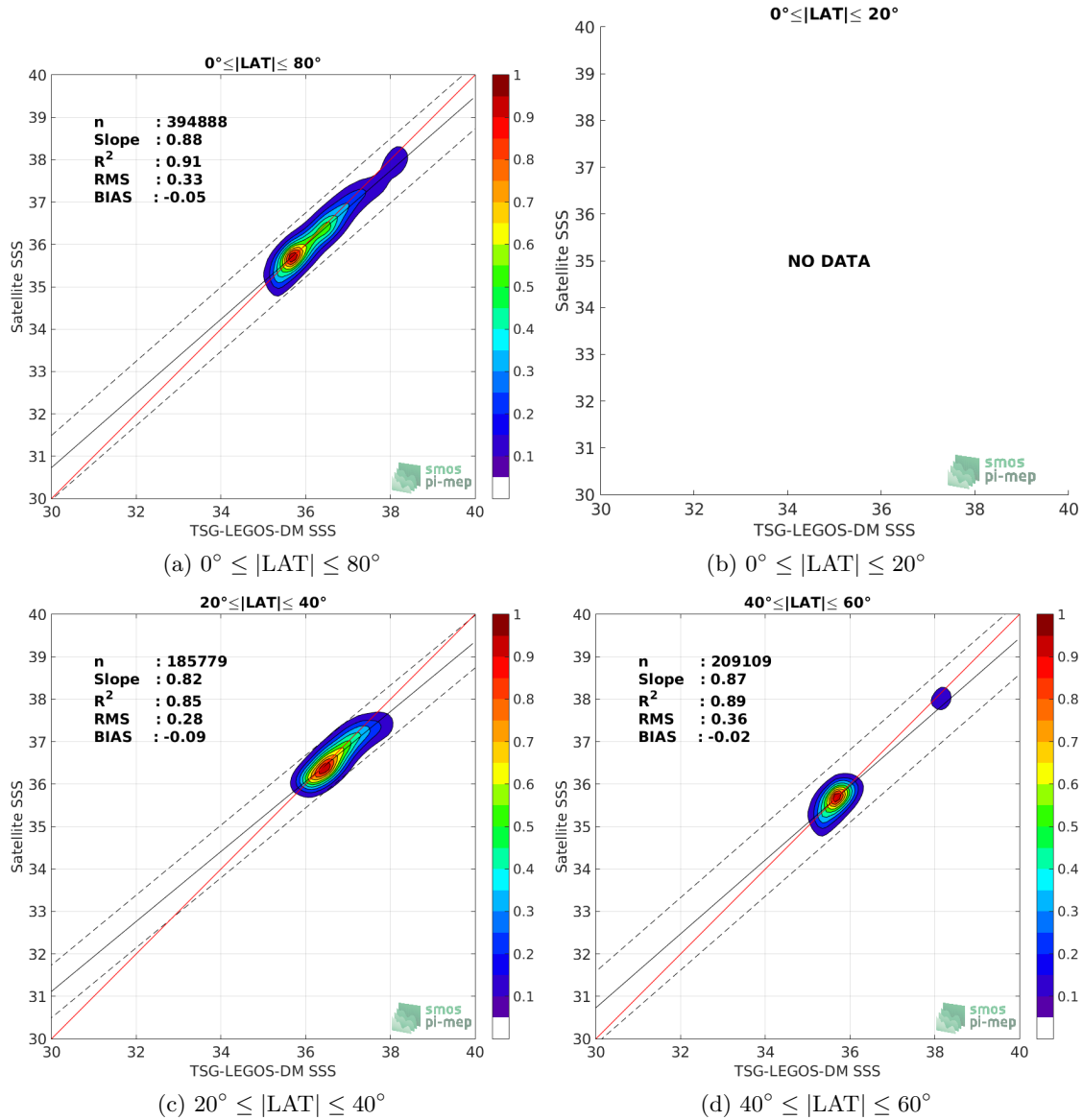
Figure 9: Contour maps of the concentration of SMOS-L3-BEC-MED-ATL-OA-V2-9DAYS-0.25DEG SSS (y-axis) versus TSG-LEGOS-DM SSS (x-axis) at match-up pairs for different latitude bands. For each plot, the red line shows x=y . The black thin and dashed lines indicate a linear fit through the data cloud and the \pm 95\% confidence levels, respectively. The number match-up pairs n , the slope and R^2 coefficient of the linear fit, the root mean square (RMS) and the mean bias between satellite and in situ data are indicated for each latitude band in each plots.
