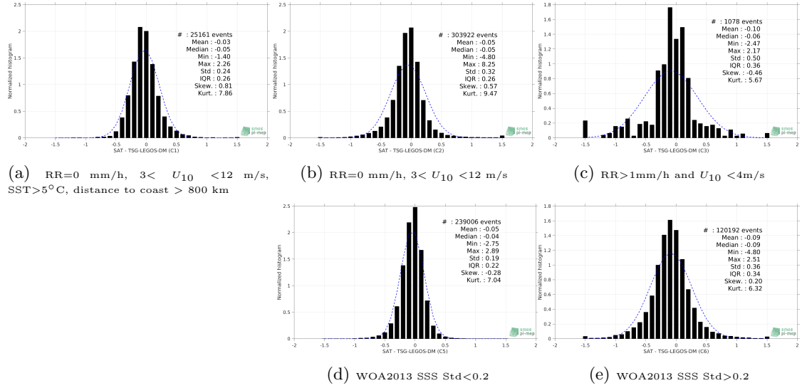
Figure 13: Normalized histogram of \Delta SSS (SMOS-L3-BEC-MED-ATL-OA-V2-9DAYS-0.25DEG - TSG-LEGOS-DM) for 5 different subdatasets corresponding to: RR=0 mm/h, 3 < U_{10} < 12 m/s, SST > 5°C, distance to coast > 800 km (a), RR=0 mm/h, 3 < U_{10} < 12 m/s (b), RR > 1mm/h and U_{10} < 4 m/s (c), WOA2013 SSS Std < 0.2 (d), WOA2013 SSS Std > 0.2 (e).
