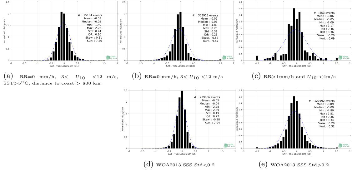
Figure 13: Normalized histogram of \Delta SSS (SMOS-L3-BEC-MED-ATL-OA-V2-9DAYS-0.25DEG - TSG-LEGOS-DM) for 5 different subdatasets corresponding to: RR=0 mm/h, 3 < U_{10} < 12 m/s, SST>5°C, distance to coast > 800 km (a), RR=0 mm/h, 3 < U_{10} < 12 m/s (b), RR>1mm/h and U_{10} < 4 m/s (c), WOA2013 SSS Std<0.2 (d), WOA2013 SSS Std>0.2 (e).
