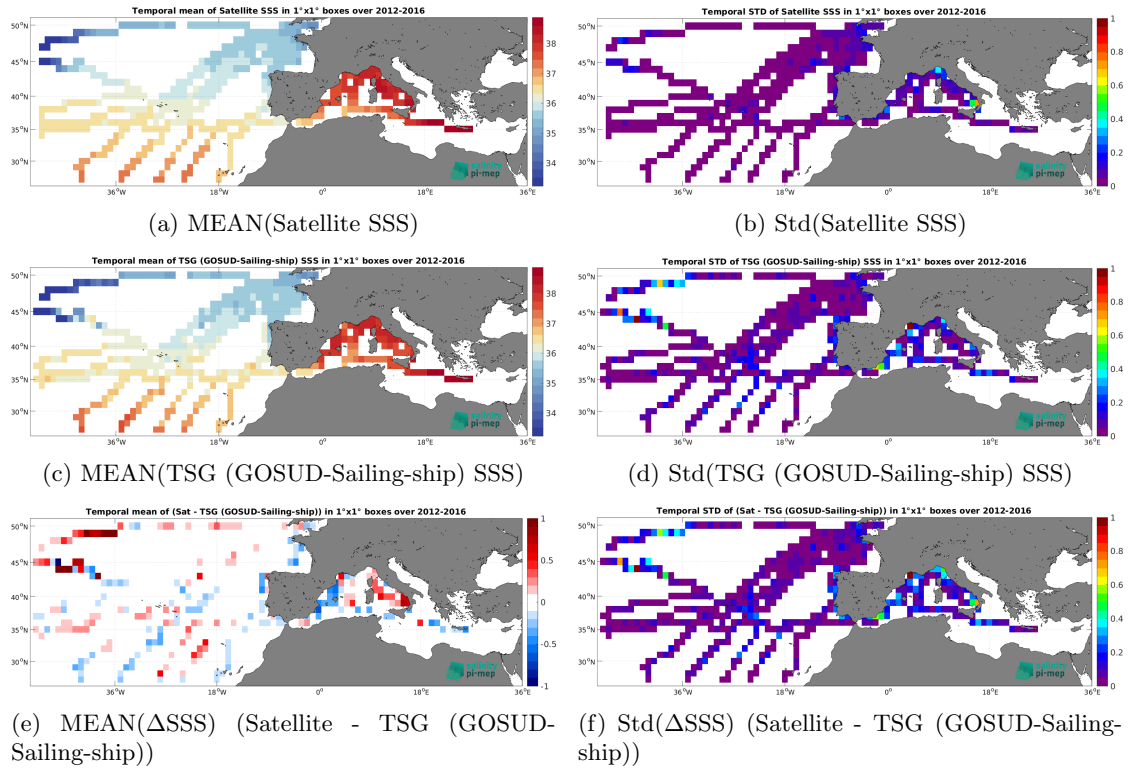
Figure 7: Temporal mean (left) and Std (right) of SSS from SMOS SSS L3 MED-ATL-OA v2 - 9 Days (BEC) (top), TSG (GOSUD-Sailing-ship) (middle), and of \Delta SSS (Satellite - TSG (GOSUD-Sailing-ship)). Only match-up pairs are used to generate these maps.
