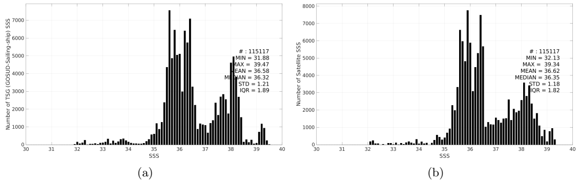
Figure 3: Histograms of SSS from TSG (GOSUD-Sailing-ship) (a) and SMOS SSS L3 MED-ATL-OA v2 - 9 Days (BEC) (b) considering all match-up pairs per bins of 0.1 over the Global Ocean Pi-MEP region and for the full satellite product period.
