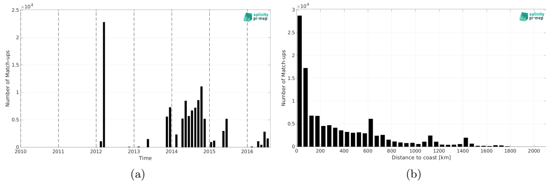
Figure 2: Number of match-ups between TSG (GOSUD-Sailing-ship) and SMOS SSS L3 MED-ATL-OA v2 - 9 Days (BEC) SSS as a function of time (a) and as function of the distance to coast (b) over the Global Ocean Pi-MEP region and for the full satellite product period.
