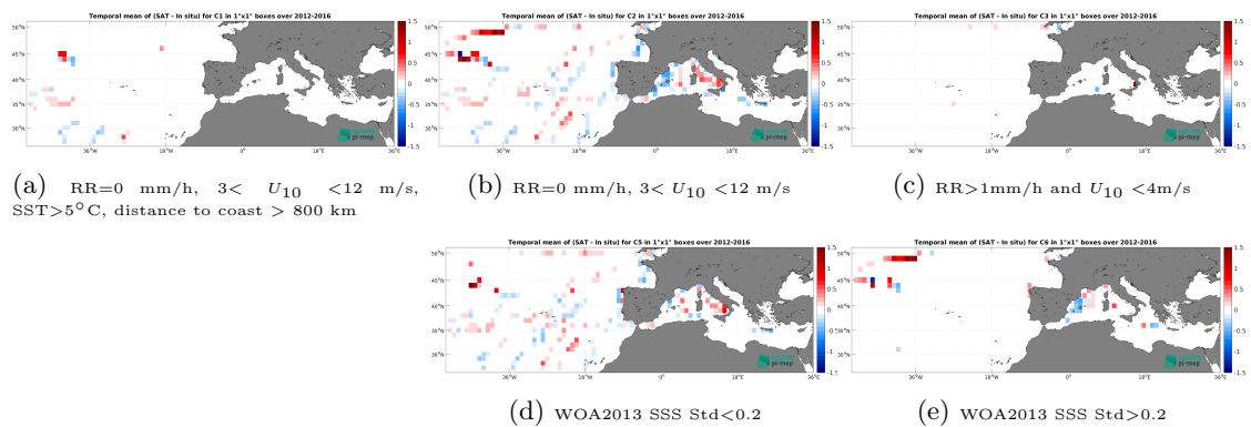
Figure 14: Temporal mean gridded over spatial boxes of size 1^\circ \times 1^\circ of \Delta SSS (SMOS SSS L3 MED-ATL-OA v2 - 9 Days (BEC) - TSG (GOSUD-Sailing-ship)) for 5 different subdatasets corresponding to:RR=0 mm/h, 3 < U_{10} < 12 m/s, SST >5^\circ\text{C} , distance to coast > 800 km (a), RR=0 mm/h, 3 < U_{10} < 12 m/s (b), RR >1 mm/h and U_{10} < 4 m/s (c), WOA2013 SSS Std <0.2 (d), WOA2013 SSS Std >0.2 (e).
