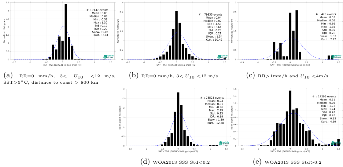
Figure 15: Normalized histogram of \Delta SSS (SMOS SSS L3 MED-ATL-OA v2 - 9 Days (BEC) - TSG (GOSUD-Sailing-ship)) for 5 different subdatasets corresponding to: RR=0 mm/h, 3 < U_{10} < 12 m/s, SST>5°C, distance to coast > 800 km (a), RR=0 mm/h, 3 < U_{10} < 12 m/s (b), RR>1mm/h and U_{10} < 4 m/s (c), WOA2013 SSS Std<0.2 (d), WOA2013 SSS Std>0.2 (e).
