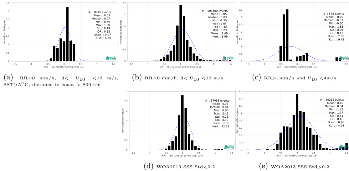
Figure 13: Normalized histogram of \Delta SSS (SMOS SSS L3 MED-ATL-OA v2 - 9 Days (BEC) - TSG (GOSUD-Sailing-ship)) for 5 different subdatasets corresponding to: RR=0 mm/h, 3 < U_{10} < 12 m/s, SST>5°C, distance to coast > 800 km (a), RR=0 mm/h, 3 < U_{10} < 12 m/s (b), RR>1mm/h and U_{10} < 4 m/s (c), WOA2013 SSS Std<0.2 (d), WOA2013 SSS Std>0.2 (e).
