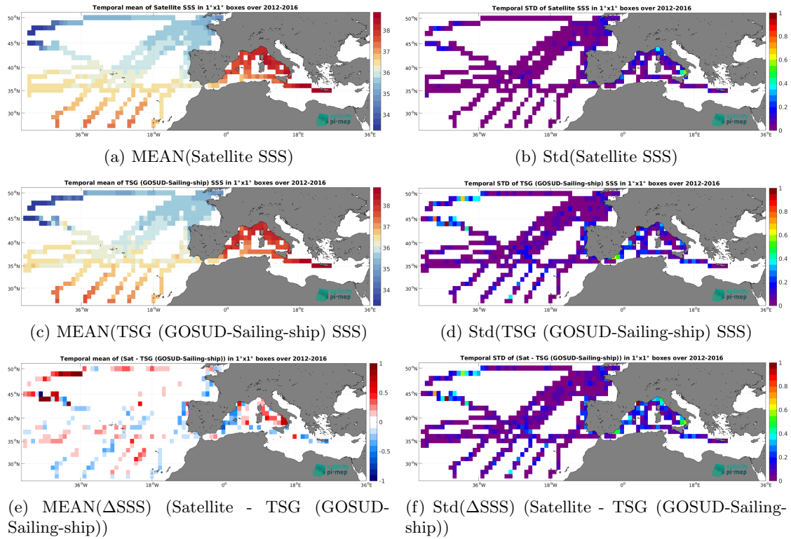
Figure 6: Temporal mean (left) and Std (right) of SSS from SMOS SSS L3 MED-ATL-OA v2 - 9 Days (BEC) (top), TSG (GOSUD-Sailing-ship) (middle), and of \Delta SSS (Satellite - TSG (GOSUD-Sailing-ship)). Only match-up pairs are used to generate these maps.
