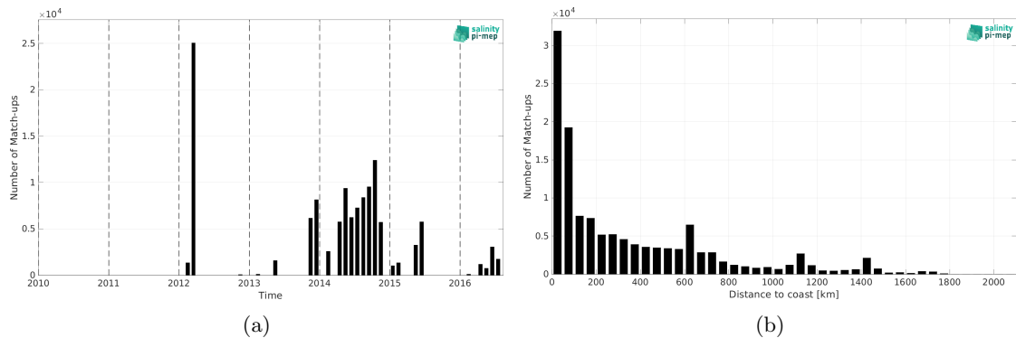
Figure 1: Number of match-ups between TSG (GOSUD-Sailing-ship) and SMOS SSS L3 MED-ATL-OA v2 - 9 Days (BEC) SSS as a function of time (a) and as function of the distance to coast (b) over the Global Ocean Pi-MEP region and for the full satellite product period.
