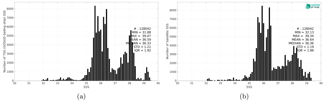
Figure 2: Histograms of SSS from TSG (GOSUD-Sailing-ship) (a) and SMOS SSS L3 MED-ATL-OA v2 - 9 Days (BEC) (b) considering all match-up pairs per bins of 0.1 over the Global Ocean Pi-MEP region and for the full satellite product period.
