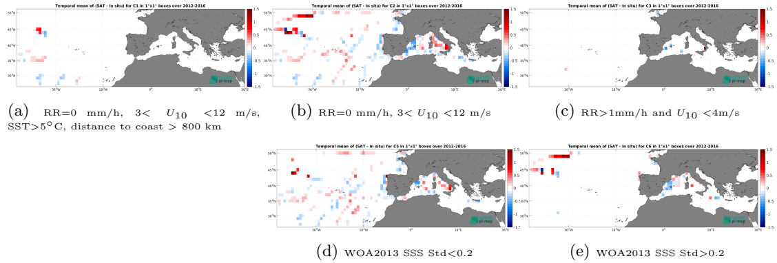
Figure 12: Temporal mean gridded over spatial boxes of size 1^{\circ}\times 1^{\circ} of \Delta SSS (SMOS SSS L3 MED-ATL-OA v2 - 9 Days (BEC) - TSG (GOSUD-Sailing-ship)) for 5 different subdatasets corresponding to:RR=0 mm/h, 3 < U_{10} < 12 m/s, SST >5^{\circ}\text{C} , distance to coast > 800 km (a), RR=0 mm/h, 3 < U_{10} < 12 m/s (b), RR >1 mm/h and U_{10} < 4 m/s (c), WOA2013 SSS Std <0.2 (d), WOA2013 SSS Std >0.2 (e).
