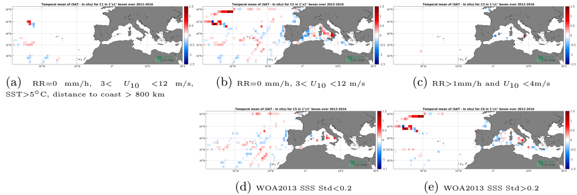
Figure 12: Temporal mean gridded over spatial boxes of size 1^\circ \times 1^\circ of \Delta SSS (SMOS SSS L3 MED-ATL-OA v2 - 9 Days (BEC) - TSG (GOSUD-Sailing-ship)) for 5 different subdatasets corresponding to:RR=0 mm/h, 3 < U_{10} < 12 m/s, SST >5^\circ\text{C} , distance to coast > 800 km (a), RR=0 mm/h, 3 < U_{10} < 12 m/s (b), RR >1 mm/h and U_{10} < 4 m/s (c), WOA2013 SSS Std <0.2 (d), WOA2013 SSS Std >0.2 (e).
