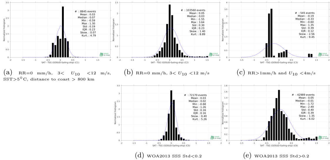
Figure 13: Normalized histogram of \Delta SSS (SMOS SSS L3 MED-ATL-OA v2 - 9 Days (BEC) - TSG (GOSUD-Sailing-ship)) for 5 different subdatasets corresponding to: RR=0 mm/h, 3 < U_{10} < 12 m/s, SST > 5°C, distance to coast > 800 km (a), RR=0 mm/h, 3 < U_{10} < 12 m/s (b), RR > 1mm/h and U_{10} < 4 m/s (c), WOA2013 SSS Std < 0.2 (d), WOA2013 SSS Std > 0.2 (e).
