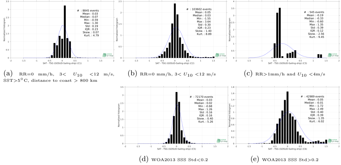
Figure 13: Normalized histogram of \Delta SSS (SMOS SSS L3 MED-ATL-OA v2 - 9 Days (BEC) - TSG (GOSUD-Sailing-ship)) for 5 different subdatasets corresponding to: RR=0 mm/h, 3 < U_{10} < 12 m/s, SST > 5°C, distance to coast > 800 km (a), RR=0 mm/h, 3 < U_{10} < 12 m/s (b), RR > 1mm/h and U_{10} < 4 m/s (c), WOA2013 SSS Std < 0.2 (d), WOA2013 SSS Std > 0.2 (e).
