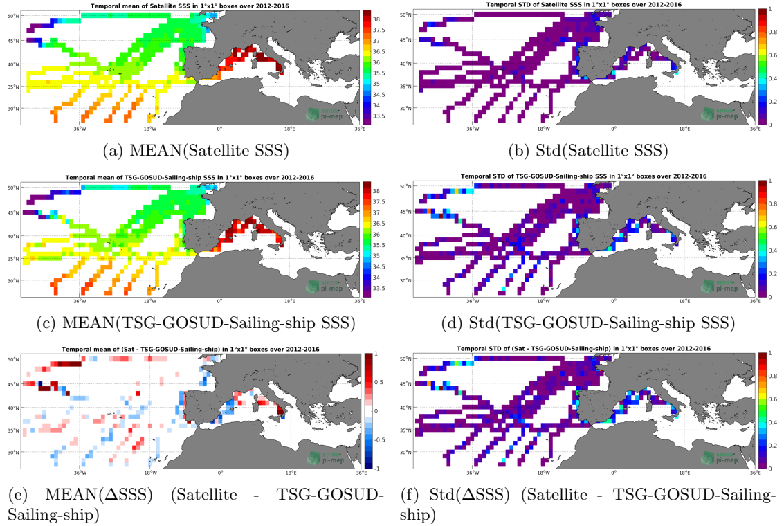
Figure 6: Temporal mean (left) and Std (right) of SSS from SMOS L3 MED-ATL-OA v2 - 9 Days (BEC) (top), TSG-GOSUD-Sailing-ship (middle), and of \Delta SSS (Satellite - TSG-GOSUD-Sailing-ship). Only match-up pairs are used to generate these maps.
