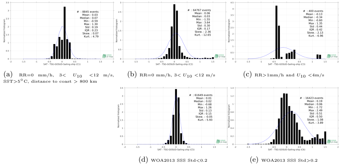
Figure 13: Normalized histogram of \Delta SSS (SMOS L3 MED-ATL-OA v2 - 9 Days (BEC) - TSG-GOSUD-Sailing-ship) for 5 different subdatasets corresponding to: RR=0 mm/h, 3 < U_{10} < 12 m/s, SST > 5°C, distance to coast > 800 km (a), RR=0 mm/h, 3 < U_{10} < 12 m/s (b), RR > 1mm/h and U_{10} < 4 m/s (c), WOA2013 SSS Std < 0.2 (d), WOA2013 SSS Std > 0.2 (e).
