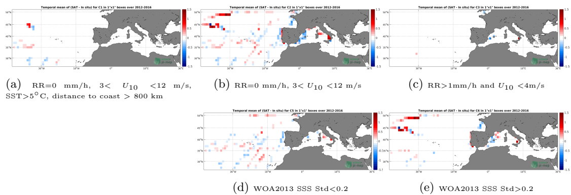
Figure 12: Temporal mean gridded over spatial boxes of size 1^\circ \times 1^\circ of \Delta SSS (SMOS L3 MED-ATL-OA v2 - 9 Days (BEC) - TSG-GOSUD-Sailing-ship) for 5 different subdatasets corresponding to:RR=0 mm/h, 3 < U_{10} < 12 m/s, SST>5°C, distance to coast > 800 km (a), RR=0 mm/h, 3 < U_{10} < 12 m/s (b), RR>1mm/h and U_{10} < 4 m/s (c), WOA2013 SSS Std<0.2 (d), WOA2013 SSS Std>0.2 (e).
