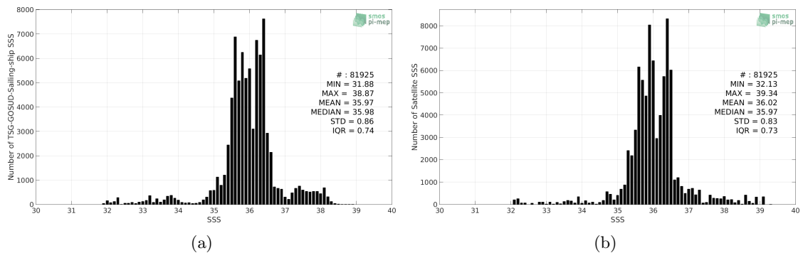
Figure 2: Histograms of SSS from TSG-GOSUD-Sailing-ship (a) and SMOS L3 MED-ATL-OA v2 - 9 Days (BEC) (b) considering all match-up pairs per bins of 0.1 over the Global Ocean Pi-MEP region and for the full satellite product period.
