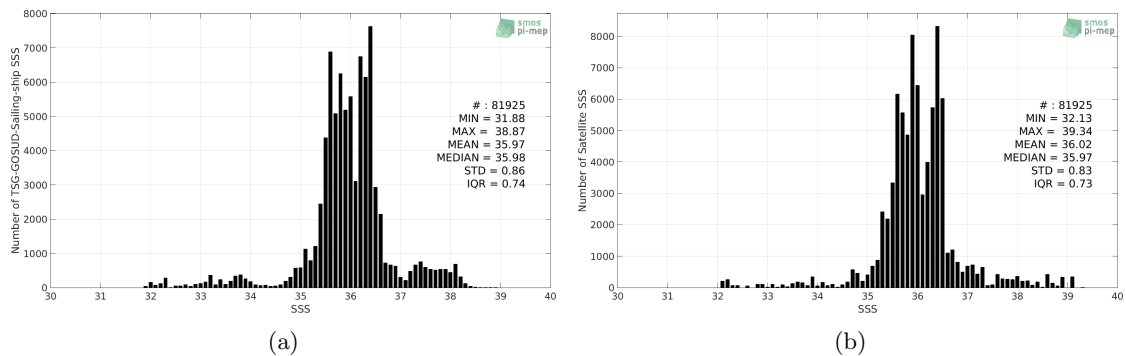
Figure 2: Histograms of SSS from TSG-GOSUD-Sailing-ship (a) and SMOS-L3-BEC-MED-ATL-OA-V2-9DAYS-0.25DEG (b) considering all match-up pairs per bins of 0.1 over the Global Ocean Pi-MEP region and for the full satellite product period.
