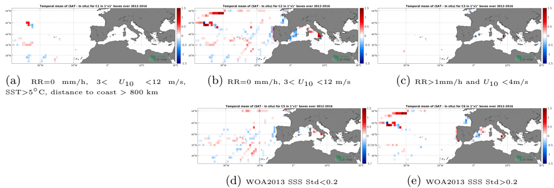
Figure 12: Temporal mean gridded over spatial boxes of size 1^\circ \times 1^\circ of \Delta SSS (SMOS-L3-BEC-MED-ATL-OA-V2-9DAYS-0.25DEG - TSG-GOSUD-Sailing-ship) for 5 different subdatasets corresponding to:RR=0 mm/h, 3 < U_{10} < 12 m/s, SST>5°C, distance to coast > 800 km (a), RR=0 mm/h, 3 < U_{10} < 12 m/s (b), RR>1mm/h and U_{10} < 4 m/s (c), WOA2013 SSS Std<0.2 (d), WOA2013 SSS Std>0.2 (e).
