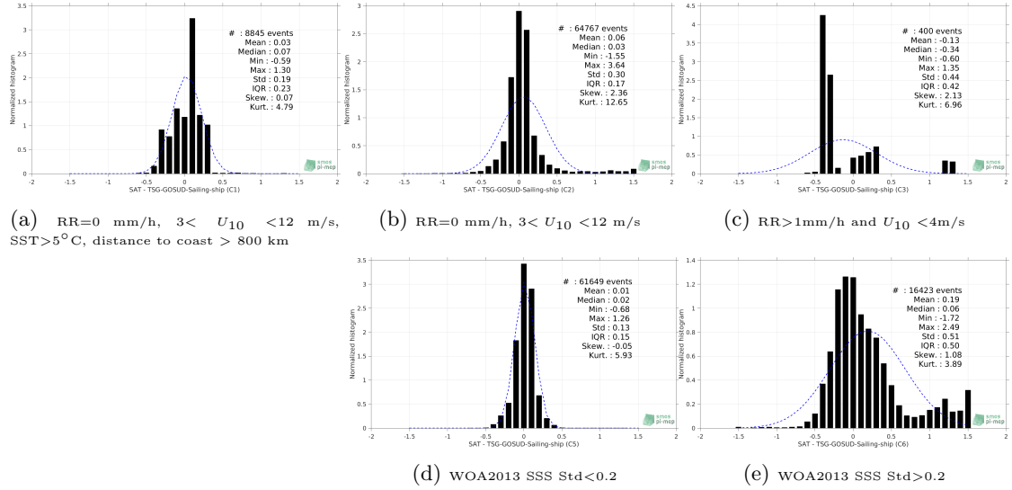
Figure 13: Normalized histogram of \Delta SSS (SMOS-L3-BEC-MED-ATL-OA-V2-9DAYS-0.25DEG - TSG-GOSUD-Sailing-ship) for 5 different subdatasets corresponding to: RR=0 mm/h, 3 < U_{10} < 12 m/s, SST>5°C, distance to coast > 800 km (a), RR=0 mm/h, 3 < U_{10} < 12 m/s (b), RR>1mm/h and U_{10} < 4 m/s (c), WOA2013 SSS Std<0.2 (d), WOA2013 SSS Std>0.2 (e).
