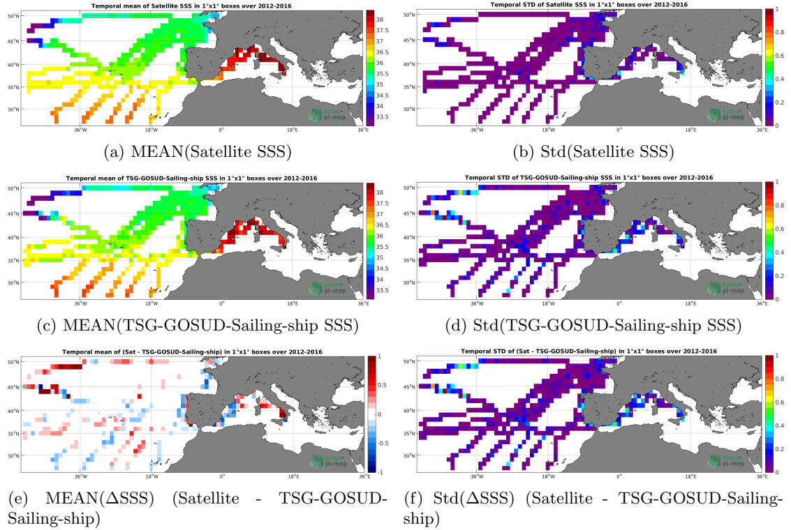
Figure 6: Temporal mean (left) and Std (right) of SSS from SMOS-L3-BEC-MED-ATL-OA-V2-9DAYS-0.25DEG (top), TSG-GOSUD-Sailing-ship (middle), and of \Delta SSS (Satellite - TSG-GOSUD-Sailing-ship). Only match-up pairs are used to generate these maps.
