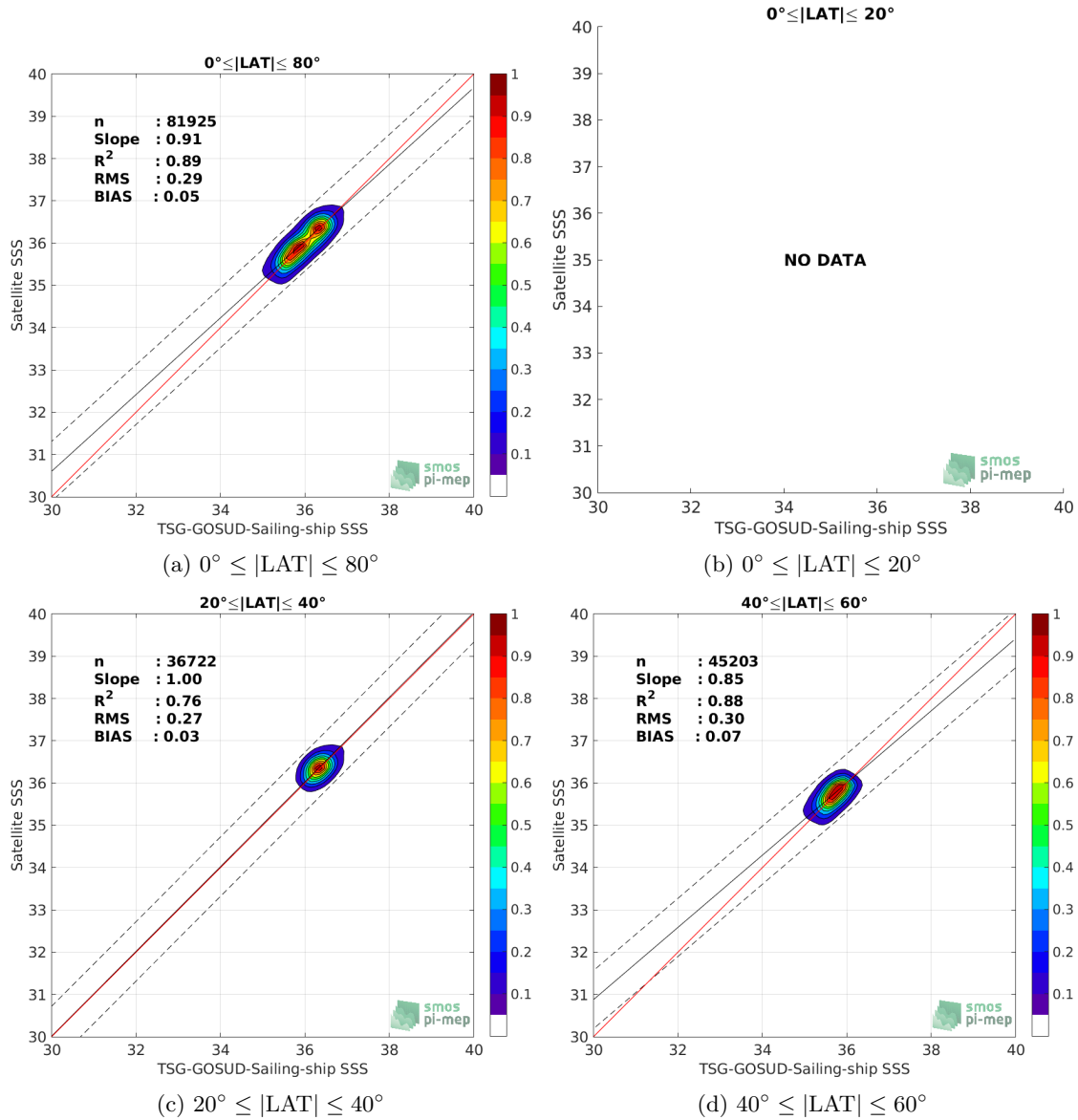
Figure 9: Contour maps of the concentration of SMOS-L3-BEC-MED-ATL-OA-V2-9DAYS-0.25DEG SSS (y-axis) versus TSG-GOSUD-Sailing-ship SSS (x-axis) at match-up pairs for different latitude bands. For each plot, the red line shows x=y . The black thin and dashed lines indicate a linear fit through the data cloud and the \pm 95\% confidence levels, respectively. The number of match-up pairs n , the slope and R^2 coefficient of the linear fit, the root mean square (RMS) and the mean bias between satellite and in situ data are indicated for each latitude band in each plot.
