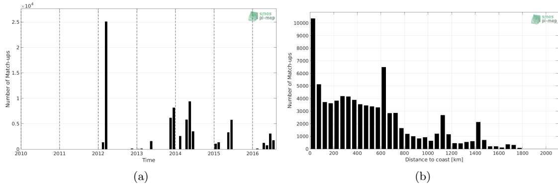
Figure 1: Number of match-ups between TSG-GOSUD-Sailing-ship and SMOS-L3-BEC-MED-ATL-OA-V2-9DAYS-0.25DEG SSS as a function of time (a) and as function of the distance to coast (b) over the Global Ocean Pi-MEP region and for the full satellite product period.
