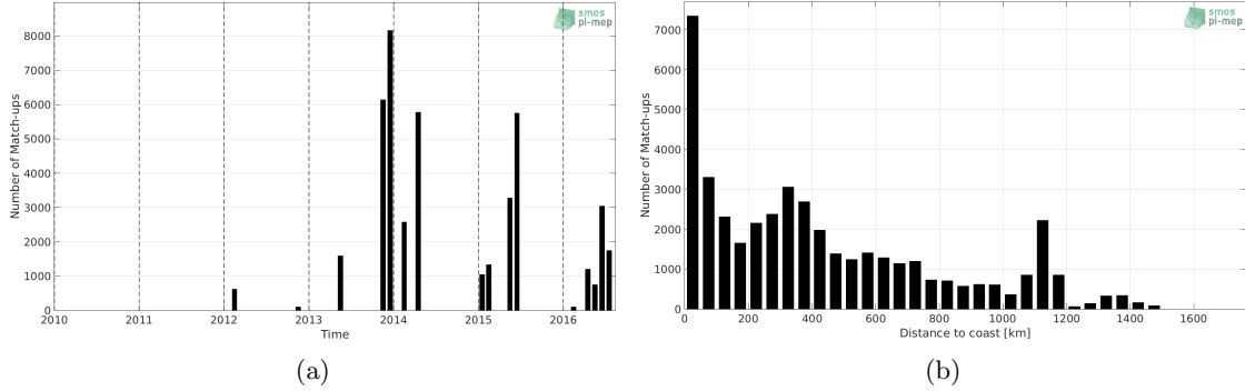
Figure 1: Number of match-ups between TSG-GOSUD-Sailing-ship and SMOS-L3-BEC-MED-ATL-OA-V2-9DAYS-0.25DEG SSS as a function of time (a) and as function of the distance to coast (b) over the Global Ocean Pi-MEP region and for the full satellite product period.
