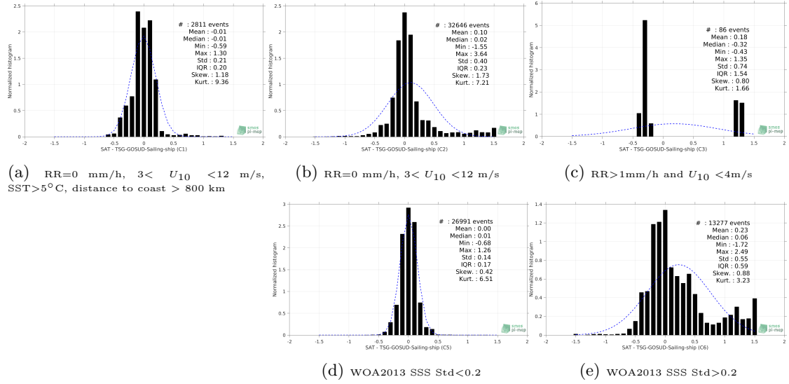
Figure 13: Normalized histogram of \Delta SSS (SMOS-L3-BEC-MED-ATL-OA-V2-9DAYS-0.25DEG - TSG-GOSUD-Sailing-ship) for 5 different subdatasets corresponding to: RR=0 mm/h, 3 < U_{10} < 12 m/s, SST>5°C, distance to coast > 800 km (a), RR=0 mm/h, 3 < U_{10} < 12 m/s (b), RR>1mm/h and U_{10} < 4 m/s (c), WOA2013 SSS Std<0.2 (d), WOA2013 SSS Std>0.2 (e).
