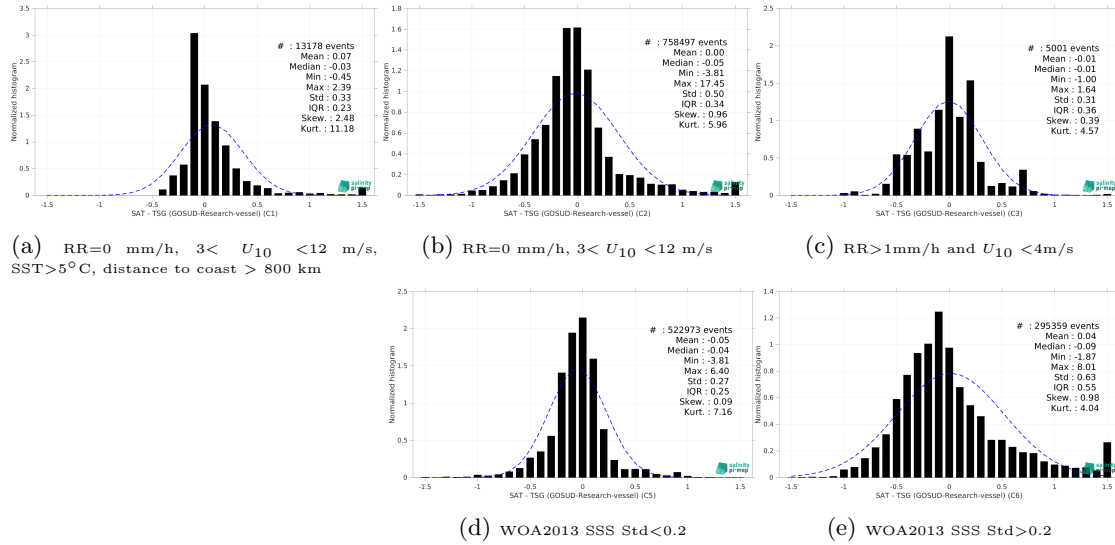
Figure 13: Normalized histogram of \Delta\text{SSS} (SMOS SSS L3 MED-ATL-OA v2 - 9 Days (BEC) - TSG (GOSUD-Research-vessel)) for 5 different subdatasets corresponding to: RR=0 mm/h, 3 < U_{10} < 12 m/s, SST>5°C, distance to coast > 800 km (a), RR=0 mm/h, 3 < U_{10} < 12 m/s (b), RR>1mm/h and U_{10} < 4 m/s (c), WOA2013 SSS Std<0.2 (d), WOA2013 SSS Std>0.2 (e).
