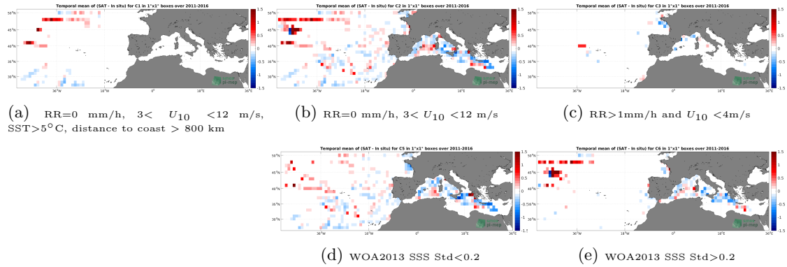
Figure 12: Temporal mean gridded over spatial boxes of size 1^{\circ}\times 1^{\circ} of \Delta SSS (SMOS SSS L3 MED-ATL-OA v2 - 9 Days (BEC) - TSG (GOSUD-Research-vessel)) for 5 different subdatasets corresponding to:RR=0 mm/h, 3 < U_{10} < 12 m/s, SST >5^{\circ}\text{C} , distance to coast > 800 km (a), RR=0 mm/h, 3 < U_{10} < 12 m/s (b), RR >1 mm/h and U_{10} < 4 m/s (c), WOA2013 SSS Std <0.2 (d), WOA2013 SSS Std >0.2 (e).
