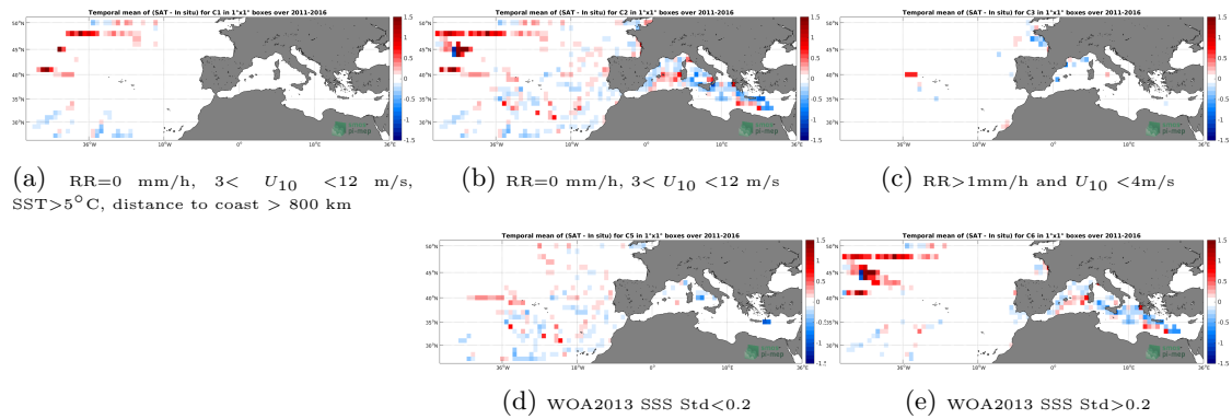
Figure 12: Temporal mean gridded over spatial boxes of size 1^\circ \times 1^\circ of \Delta SSS (SMOS-L3-BEC-MED-ATL-OA-V2-9DAYS-0.25DEG - TSG-GOSUD-Research-vessel) for 5 different subdatasets corresponding to:RR=0 mm/h, 3 < U_{10} < 12 m/s, SST >5^\circ C, distance to coast > 800 km (a), RR=0 mm/h, 3 < U_{10} < 12 m/s (b), RR >1 mm/h and U_{10} < 4 m/s (c), WOA2013 SSS Std <0.2 (d), WOA2013 SSS Std >0.2 (e).
