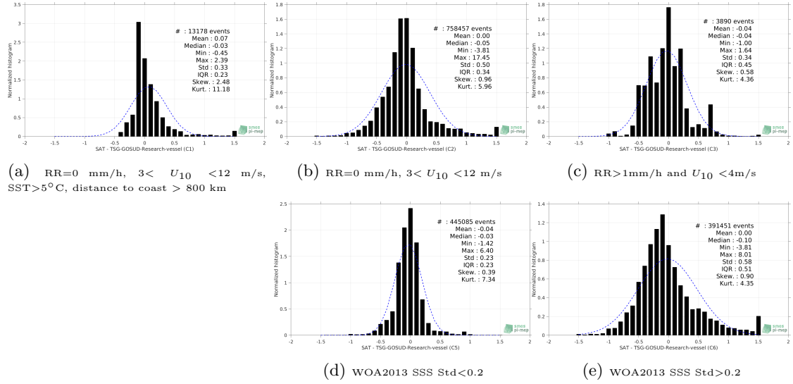
Figure 13: Normalized histogram of \Delta SSS (SMOS-L3-BEC-MED-ATL-OA-V2-9DAYS-0.25DEG - TSG-GOSUD-Research-vessel) for 5 different subdatasets corresponding to: RR=0 mm/h, 3 < U_{10} < 12 m/s, SST>5°C, distance to coast > 800 km (a), RR=0 mm/h, 3 < U_{10} < 12 m/s (b), RR>1mm/h and U_{10} < 4 m/s (c), WOA2013 SSS Std<0.2 (d), WOA2013 SSS Std>0.2 (e).
