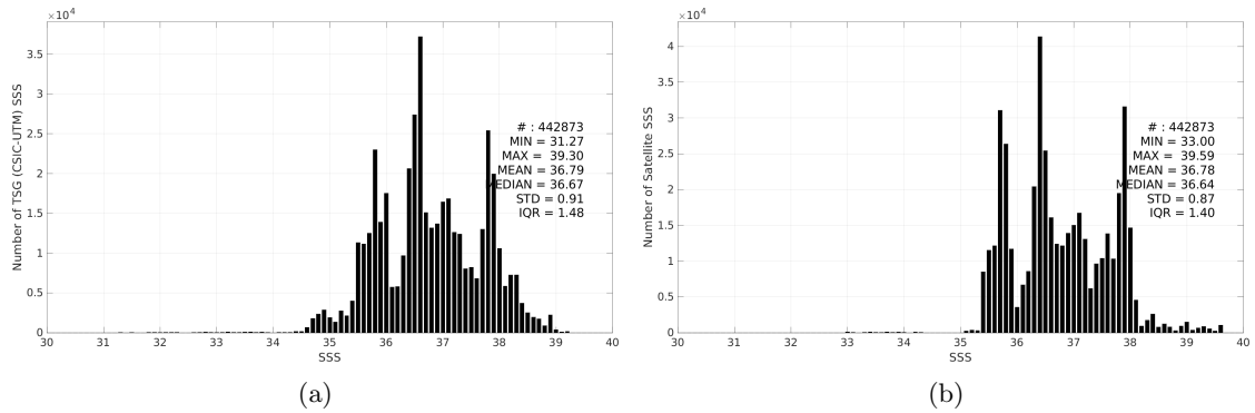
Figure 3: Histograms of SSS from TSG (CSIC-UTM) (a) and SMOS SSS L3 MED-ATL-OA v2 - 9 Days (BEC) (b) considering all match-up pairs per bins of 0.1 over the Global Ocean Pi-MEP region and for the full satellite product period.
