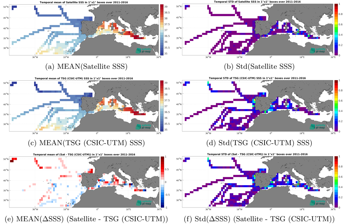
Figure 7: Temporal mean (left) and Std (right) of SSS from SMOS SSS L3 MED-ATL-OA v2 - 9 Days (BEC) (top), TSG (CSIC-UTM) (middle), and of \Delta SSS (Satellite - TSG (CSIC-UTM)). Only match-up pairs are used to generate these maps.
