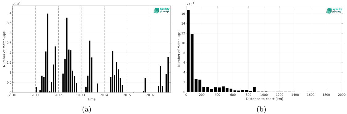
Figure 2: Number of match-ups between TSG (CSIC-UTM) and SMOS SSS L3 MED-ATL-OA v2 - 9 Days (BEC) SSS as a function of time (a) and as function of the distance to coast (b) over the Global Ocean Pi-MEP region and for the full satellite product period.
