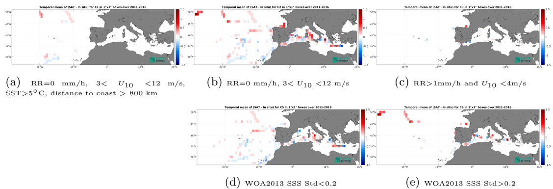
Figure 14: Temporal mean gridded over spatial boxes of size 1^\circ \times 1^\circ of \Delta\text{SSS} (SMOS SSS L3 MED-ATL-OA v2 - 9 Days (BEC) - TSG (CSIC-UTM)) for 5 different subdatasets corresponding to:RR=0 mm/h, 3 < U_{10} < 12 m/s, SST >5^\circ\text{C} , distance to coast > 800 km (a), RR=0 mm/h, 3 < U_{10} < 12 m/s (b), RR >1 mm/h and U_{10} < 4 m/s (c), WOA2013 SSS Std <0.2 (d), WOA2013 SSS Std >0.2 (e).
