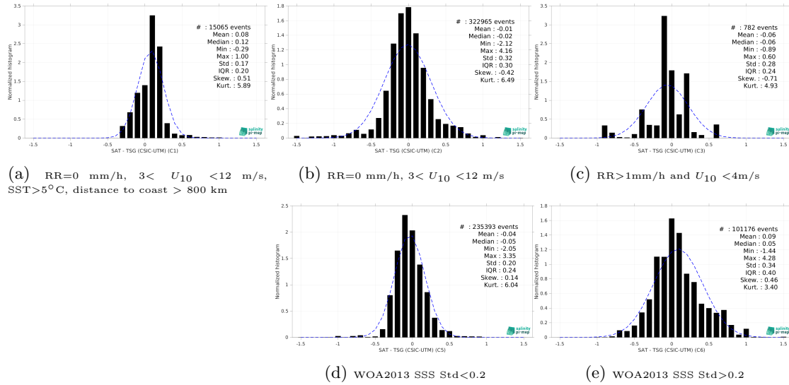
Figure 15: Normalized histogram of \Delta SSS (SMOS SSS L3 MED-ATL-OA v2 - 9 Days (BEC) - TSG (CSIC-UTM)) for 5 different subdatasets corresponding to: RR=0 mm/h, 3 < U_{10} < 12 m/s, SST>5°C, distance to coast > 800 km (a), RR=0 mm/h, 3 < U_{10} < 12 m/s (b), RR>1mm/h and U_{10} < 4 m/s (c), WOA2013 SSS Std<0.2 (d), WOA2013 SSS Std>0.2 (e).
