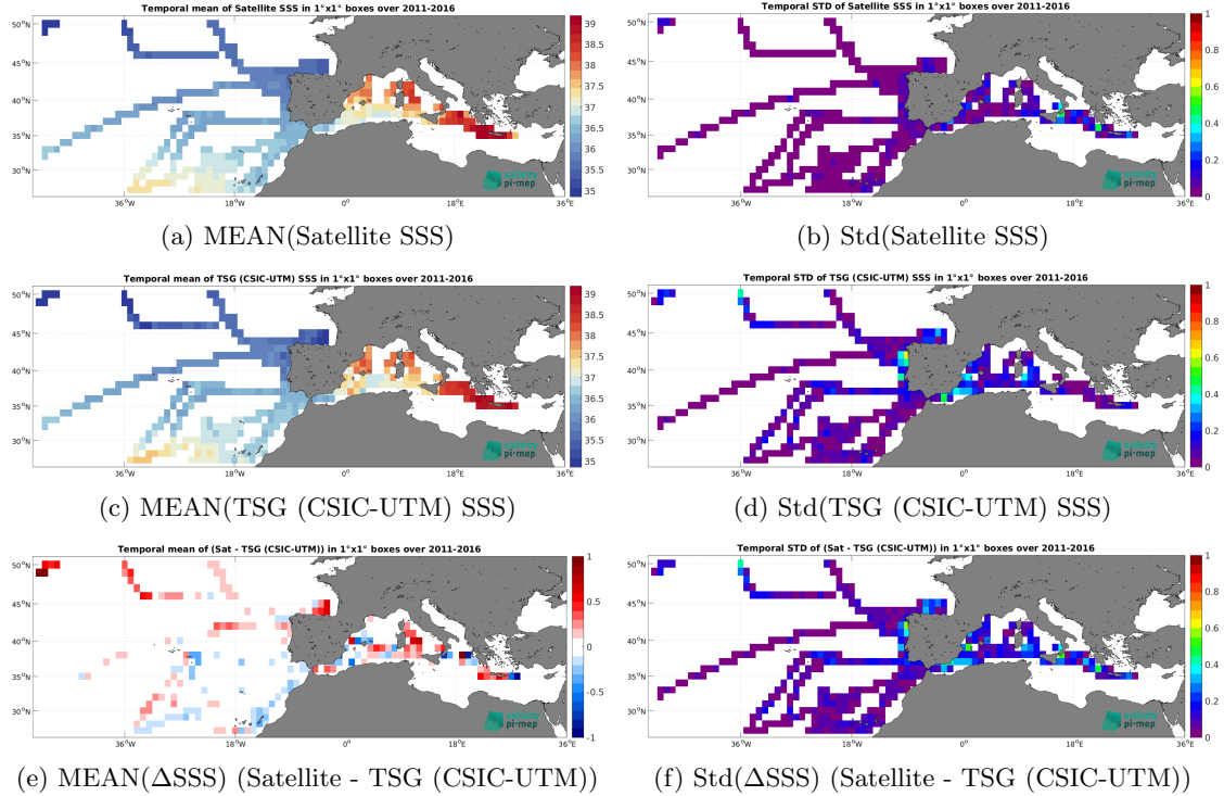
Figure 6: Temporal mean (left) and Std (right) of SSS from SMOS SSS L3 MED-ATL-OA v2 - 9 Days (BEC) (top), TSG (CSIC-UTM) (middle), and of \Delta SSS (Satellite - TSG (CSIC-UTM)). Only match-up pairs are used to generate these maps.
