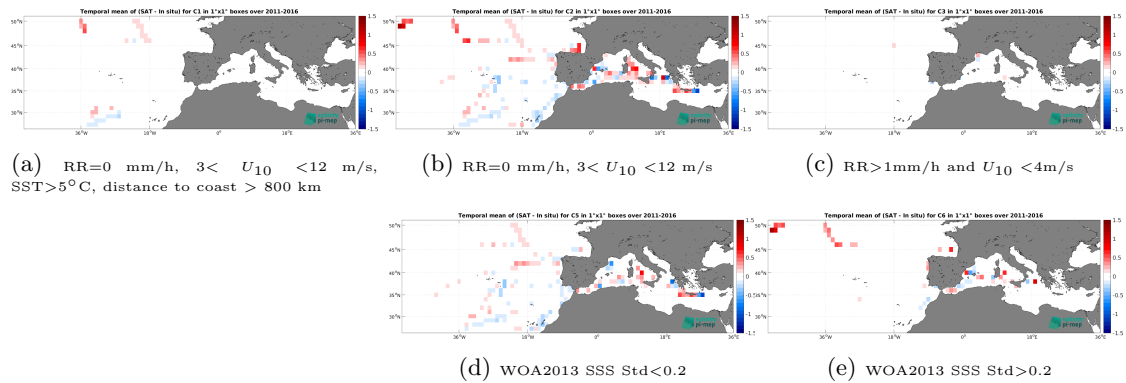
Figure 12: Temporal mean gridded over spatial boxes of size 1^\circ \times 1^\circ of \Delta SSS (SMOS SSS L3 MED-ATL-OA v2 - 9 Days (BEC) - TSG (CSIC-UTM)) for 5 different subdatasets corresponding to:RR=0 mm/h, 3 < U_{10} < 12 m/s, SST >5^\circ C, distance to coast > 800 km (a), RR=0 mm/h, 3 < U_{10} < 12 m/s (b), RR >1 mm/h and U_{10} < 4 m/s (c), WOA2013 SSS Std <0.2 (d), WOA2013 SSS Std >0.2 (e).
