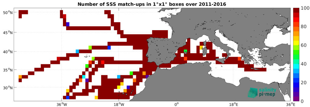
Figure 4: Number of SSS match-ups between TSG (CSIC-UTM) SSS and the SMOS SSS L3 MED-ATL-OA v2 - 9 Days (BEC) SSS product for the Global Ocean Pi-MEP region over 1^\circ \times 1^\circ boxes and for the full satellite product period.
