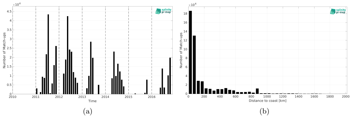
Figure 1: Number of match-ups between TSG (CSIC-UTM) and SMOS SSS L3 MED-ATL-OA v2 - 9 Days (BEC) SSS as a function of time (a) and as function of the distance to coast (b) over the Global Ocean Pi-MEP region and for the full satellite product period.
