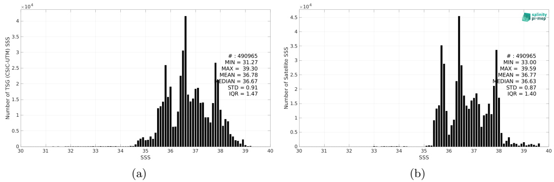
Figure 2: Histograms of SSS from TSG (CSIC-UTM) (a) and SMOS SSS L3 MED-ATL-OA v2 - 9 Days (BEC) (b) considering all match-up pairs per bins of 0.1 over the Global Ocean Pi-MEP region and for the full satellite product period.
