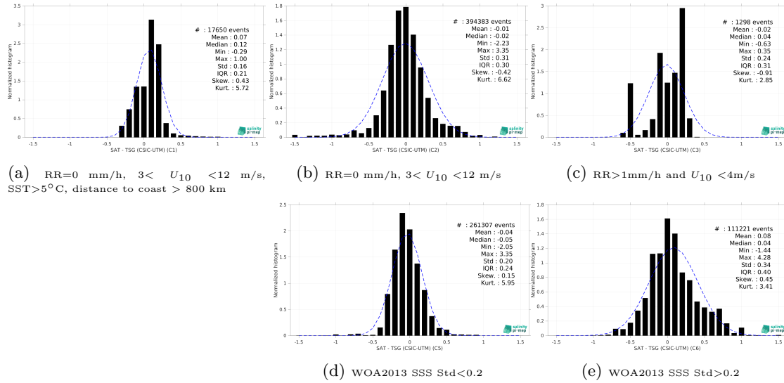
Figure 13: Normalized histogram of \Delta SSS (SMOS SSS L3 MED-ATL-OA v2 - 9 Days (BEC) - TSG (CSIC-UTM)) for 5 different subdatasets corresponding to: RR=0 mm/h, 3 < U_{10} < 12 m/s, SST>5°C, distance to coast > 800 km (a), RR=0 mm/h, 3 < U_{10} < 12 m/s (b), RR>1mm/h and U_{10} < 4 m/s (c), WOA2013 SSS Std<0.2 (d), WOA2013 SSS Std>0.2 (e).
