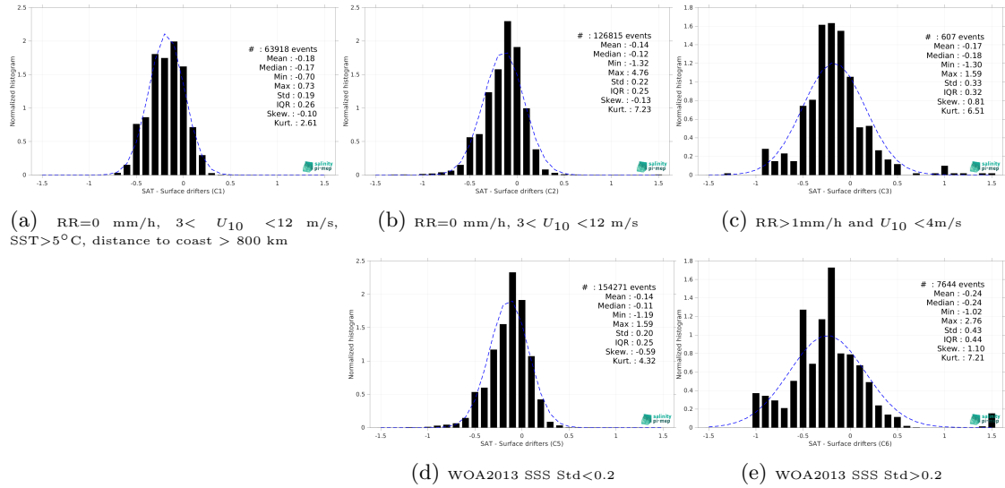
Figure 14: Normalized histogram of \Delta SSS (SMOS SSS L3 MED-ATL-OA v2 - 9 Days (BEC) - Surface drifters) for 5 different subdatasets corresponding to: RR=0 mm/h, 3 < U_{10} < 12 m/s, SST > 5°C, distance to coast > 800 km (a), RR=0 mm/h, 3 < U_{10} < 12 m/s (b), RR > 1mm/h and U_{10} < 4 m/s (c), WOA2013 SSS Std < 0.2 (d), WOA2013 SSS Std > 0.2 (e).
