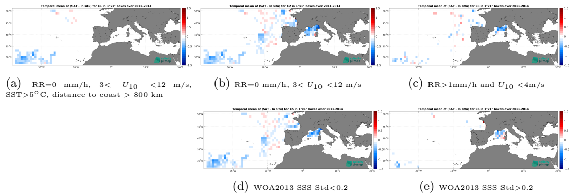
Figure 13: Temporal mean gridded over spatial boxes of size 1^\circ \times 1^\circ of \Delta SSS (SMOS SSS L3 MED-ATL-OA v2 - 9 Days (BEC) - Surface drifters) for 5 different subdatasets corresponding to:RR=0 mm/h, 3 < U_{10} < 12 m/s, SST >5^\circ C, distance to coast > 800 km (a), RR=0 mm/h, 3 < U_{10} < 12 m/s (b), RR >1 mm/h and U_{10} < 4 m/s (c), WOA2013 SSS Std <0.2 (d), WOA2013 SSS Std >0.2 (e).
