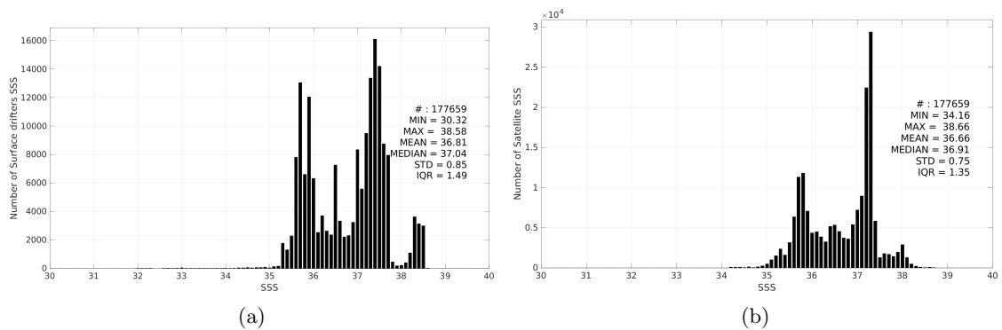
Figure 3: Histograms of SSS from Surface drifters (a) and SMOS SSS L3 MED-ATL-OA v2 - 9 Days (BEC) (b) considering all match-up pairs per bins of 0.1 over the Global Ocean Pi-MEP region and for the full satellite product period.
