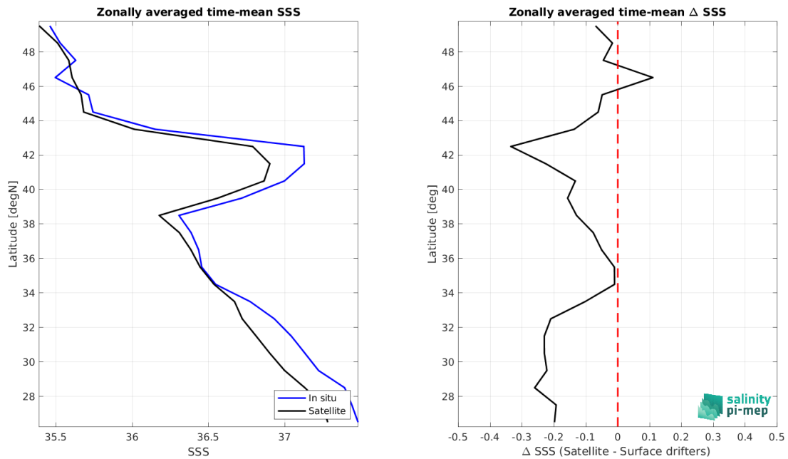
Figure 8: Left panel: Zonal mean SSS from SMOS SSS L3 MED-ATL-OA v2 - 9 Days (BEC) satellite product (black) and from Surface drifters (blue). Right panel: Zonal mean of \Delta SSS (Satellite - Surface drifters) for all the collected Pi-MEP match-up pairs estimated over the full satellite product period.
