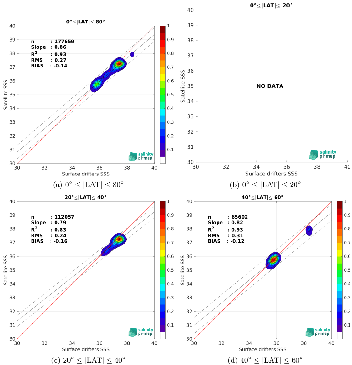
Figure 9: Contour maps of the concentration of SMOS SSS L3 MED-ATL-OA v2 - 9 Days (BEC) SSS (y-axis) versus Surface drifters SSS (x-axis) at match-up pairs for different latitude bands. For each plot, the red line shows x=y . The black thin and dashed lines indicate a linear fit through the data cloud and the \pm 95\% confidence levels, respectively. The number match-up pairs n , the slope and R^2 coefficient of the linear fit, the root mean square (RMS) and the mean bias between satellite and in situ data are indicated for each latitude band in each plots.
