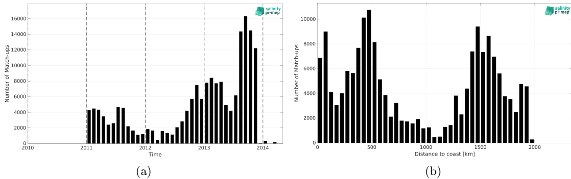
Figure 2: Number of match-ups between Surface drifters and SMOS SSS L3 MED-ATL-OA v2 - 9 Days (BEC) SSS as a function of time (a) and as function of the distance to coast (b) over the Global Ocean Pi-MEP region and for the full satellite product period.
