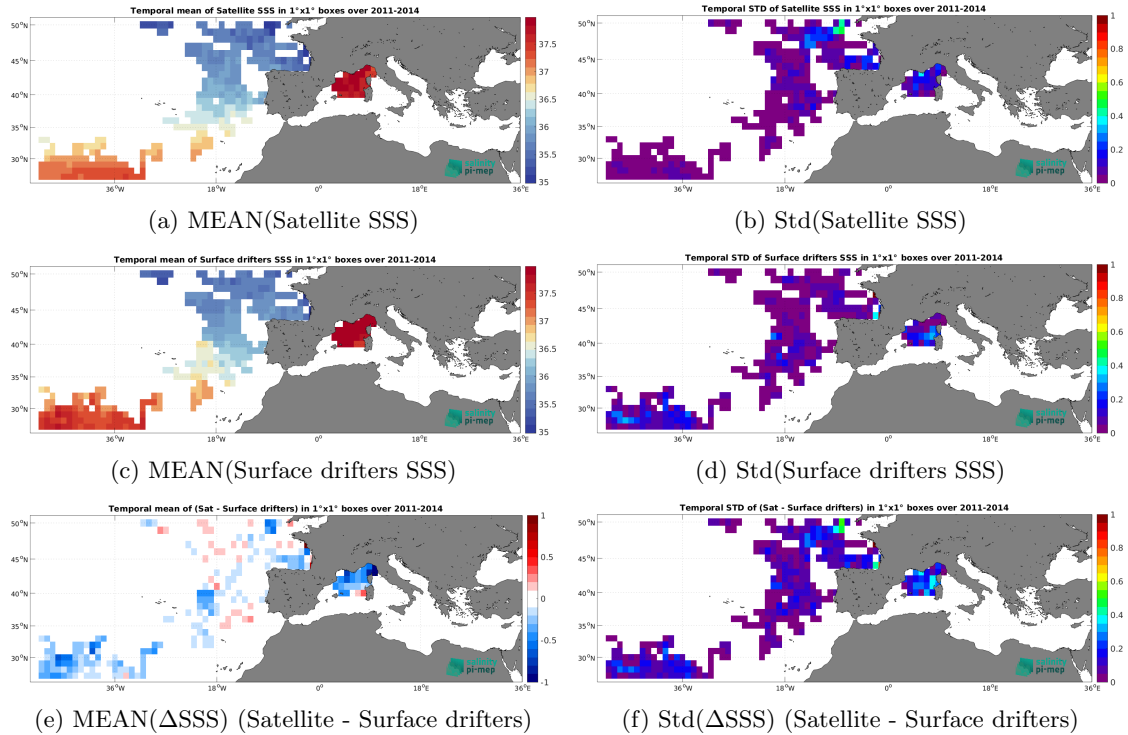
Figure 6: Temporal mean (left) and Std (right) of SSS from SMOS SSS L3 MED-ATL-OA v2 - 9 Days (BEC) (top), Surface drifters (middle), and of \Delta SSS (Satellite - Surface drifters). Only match-up pairs are used to generate these maps.
