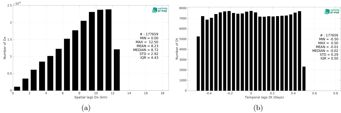
Figure 5: Histograms of the spatial (a) and temporal (b) lags between the location/time of the Surface drifters measurement and the date of the corresponding SMOS SSS L3 MED-ATL-OA v2 - 9 Days (BEC) SSS pixel.
