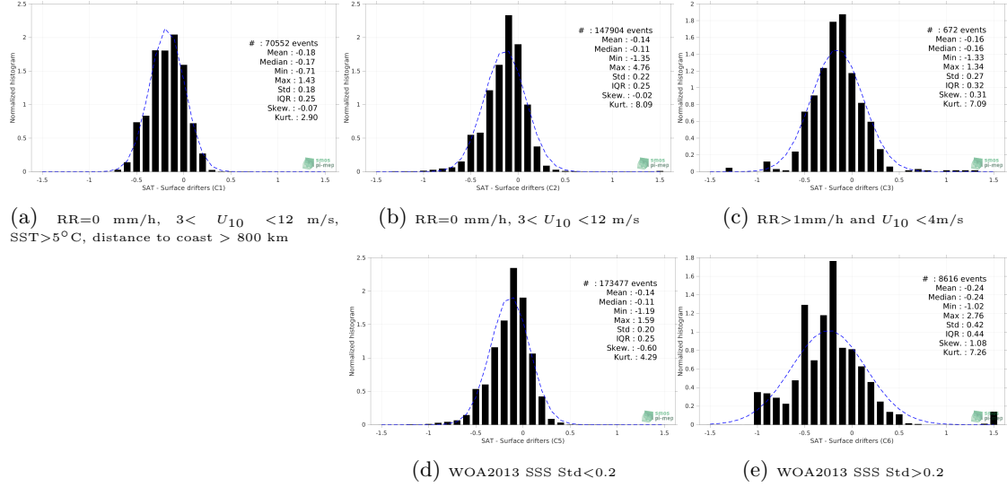
Figure 12: Normalized histogram of \Delta SSS (SMOS SSS L3 MED-ATL-OA v2 - 9 Days (BEC) - Surface drifters) for 5 different subdatasets corresponding to: RR=0 mm/h, 3 < U_{10} < 12 m/s, SST > 5°C, distance to coast > 800 km (a), RR=0 mm/h, 3 < U_{10} < 12 m/s (b), RR > 1mm/h and U_{10} < 4 m/s (c), WOA2013 SSS Std < 0.2 (d), WOA2013 SSS Std > 0.2 (e).
