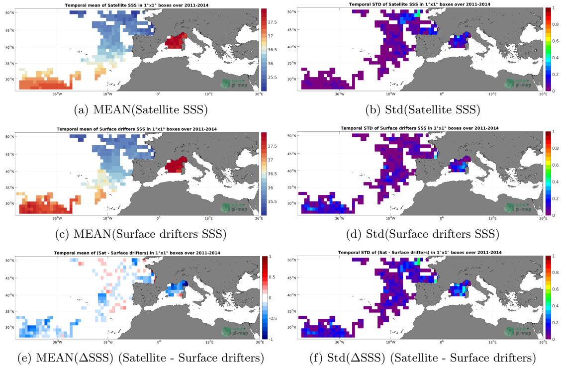
Figure 5: Temporal mean (left) and Std (right) of SSS from SMOS SSS L3 MED-ATL-OA v2 - 9 Days (BEC) (top), Surface drifters (middle), and of \Delta SSS (Satellite - Surface drifters). Only match-up pairs are used to generate these maps.
