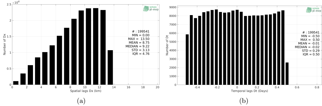
Figure 4: Histograms of the spatial (a) and temporal (b) lags between the location/time of the Surface drifters measurement and the date of the corresponding SMOS SSS L3 MED-ATL-OA v2 - 9 Days (BEC) SSS pixel.
