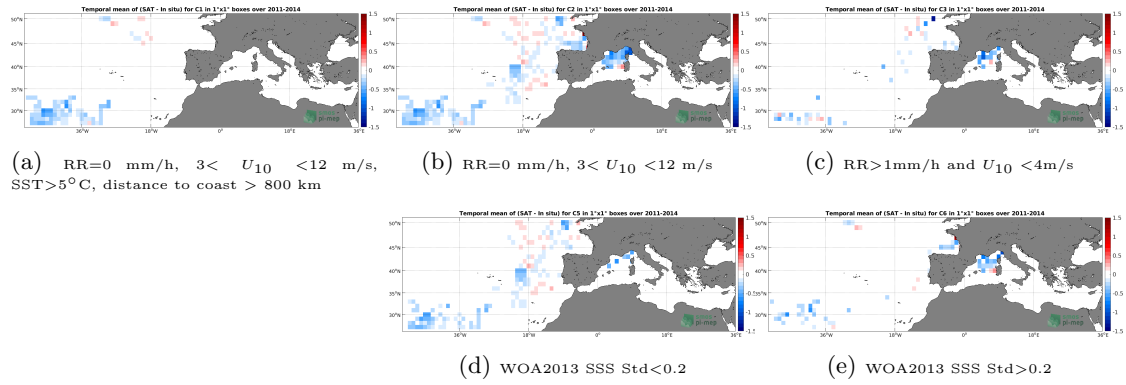
Figure 11: Temporal mean gridded over spatial boxes of size 1^\circ \times 1^\circ of \Delta SSS (SMOS SSS L3 MED-ATL-OA v2 - 9 Days (BEC) - Surface drifters) for 5 different subdatasets corresponding to: RR=0 mm/h, 3 < U_{10} < 12 m/s, SST > 5^\circ C , distance to coast > 800 km (a), RR=0 mm/h, 3 < U_{10} < 12 m/s (b), RR > 1 mm/h and U_{10} < 4 m/s (c), WOA2013 SSS Std < 0.2 (d), WOA2013 SSS Std > 0.2 (e).
