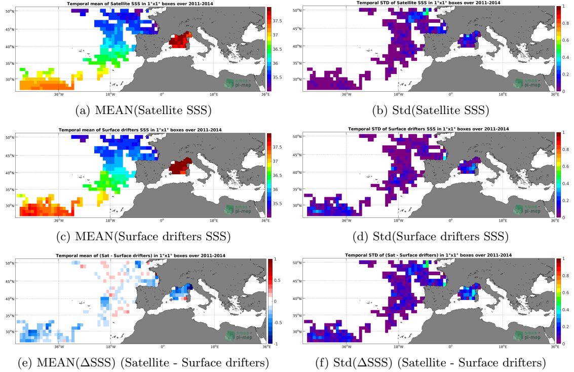
Figure 5: Temporal mean (left) and Std (right) of SSS from SMOS SSS L3 MED-ATL-OA v2 - 9 Days (BEC) (top), Surface drifters (middle), and of \Delta\text{SSS} (Satellite - Surface drifters). Only match-up pairs are used to generate these maps.
