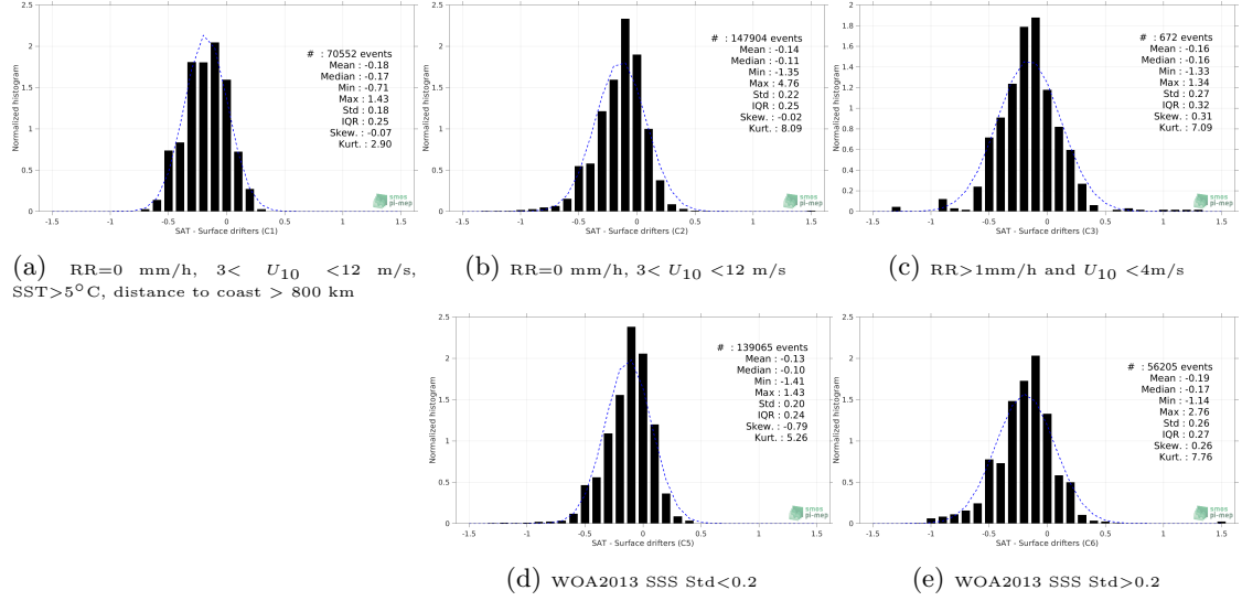
Figure 12: Normalized histogram of \Delta SSS (SMOS SSS L3 MED-ATL-OA v2 - 9 Days (BEC) - Surface drifters) for 5 different subdatasets corresponding to: RR=0 mm/h, 3 < U_{10} < 12 m/s, SST > 5^\circ\text{C} , distance to coast > 800 km (a), RR=0 mm/h, 3 < U_{10} < 12 m/s (b), RR > 1 mm/h and U_{10} < 4 m/s (c), WOA2013 SSS Std < 0.2 (d), WOA2013 SSS Std > 0.2 (e).
