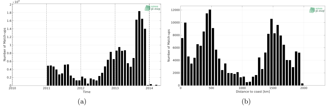
Figure 1: Number of match-ups between Surface drifters and SMOS SSS L3 MED-ATL-OA v2 - 9 Days (BEC) SSS as a function of time (a) and as function of the distance to coast (b) over the Global Ocean Pi-MEP region and for the full satellite product period.
