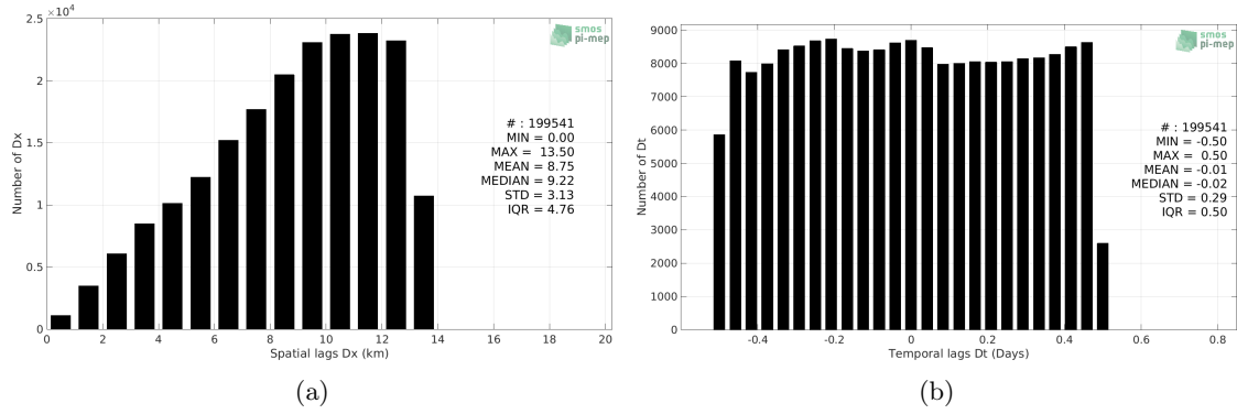
Figure 4: Histograms of the spatial (a) and temporal (b) lags between the time of the Surface drifters measurements and the date of the corresponding SMOS SSS L3 MED-ATL-OA v2 - 9 Days (BEC) SSS product.
