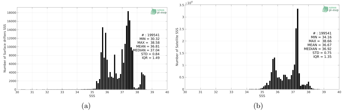
Figure 2: Histograms of SSS from Surface drifters (a) and SMOS SSS L3 MED-ATL-OA v2 - 9 Days (BEC) (b) considering all match-up pairs per bins of 0.1 over the Global Ocean Pi-MEP region and for the full satellite product period.
