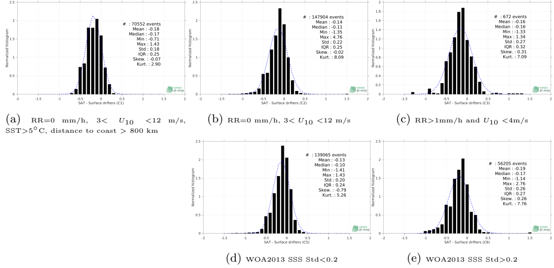
Figure 12: Normalized histogram of \Delta SSS (SMOS SSS L3 MED-ATL-OA v2 - 9 Days (BEC) - Surface drifters) for 5 different subdatasets corresponding to: RR=0 mm/h, 3 < U_{10} < 12 m/s, SST>5°C, distance to coast > 800 km (a), RR=0 mm/h, 3 < U_{10} < 12 m/s (b), RR>1mm/h and U_{10} < 4 m/s (c), WOA2013 SSS Std<0.2 (d), WOA2013 SSS Std>0.2 (e).
