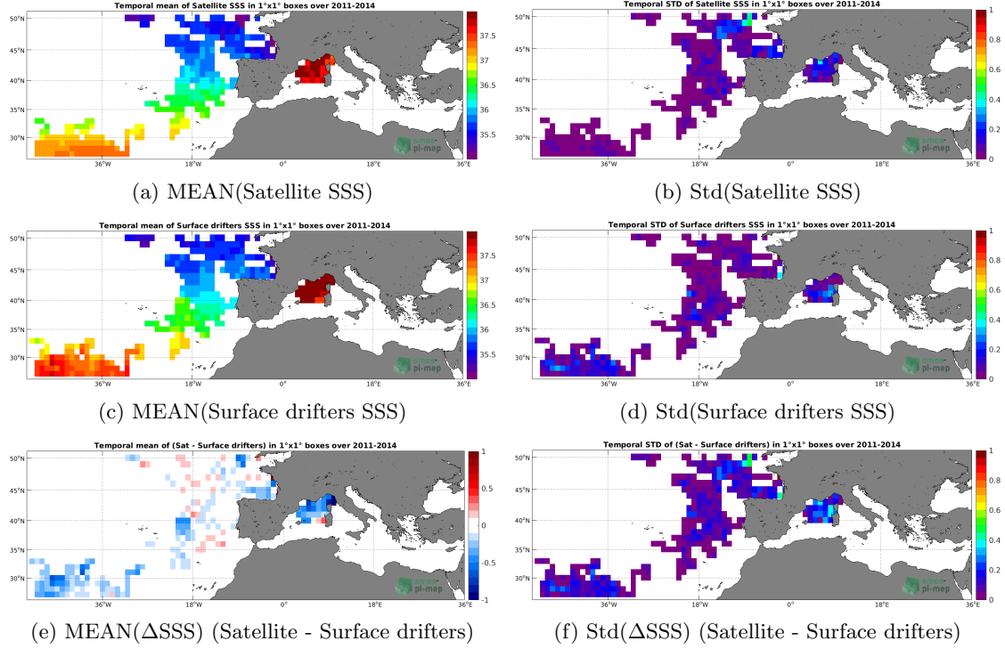
Figure 5: Temporal mean (left) and Std (right) of SSS from SMOS SSS L3 MED-ATL-OA v2 - 9 Days (BEC) (top), Surface drifters (middle), and of \Delta SSS (Satellite - Surface drifters). Only match-up pairs are used to generate these maps.
