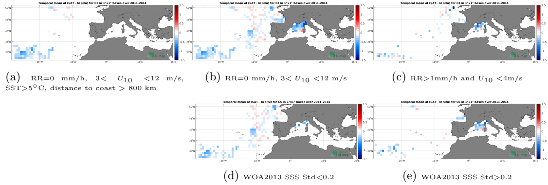
Figure 11: Temporal mean gridded over spatial boxes of size 1^\circ \times 1^\circ of \Delta SSS (SMOS SSS L3 MED-ATL-OA v2 - 9 Days (BEC) - Surface drifters) for 5 different subdatasets corresponding to: RR=0 mm/h, 3 < U_{10} < 12 m/s, SST > 5^\circ C , distance to coast > 800 km (a), RR=0 mm/h, 3 < U_{10} < 12 m/s (b), RR > 1 mm/h and U_{10} < 4 m/s (c), WOA2013 SSS Std < 0.2 (d), WOA2013 SSS Std > 0.2 (e).
