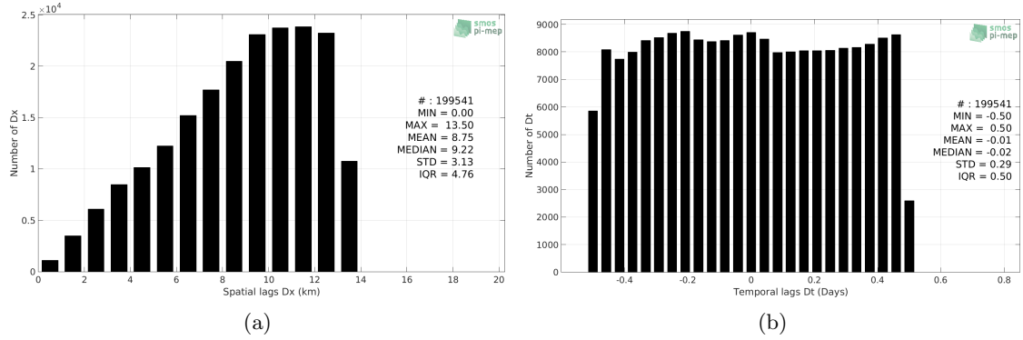
Figure 4: Histograms of the spatial (a) and temporal (b) lags between the time of the Surface drifters measurements and the date of the corresponding SMOS L3 MED-ATL-OA v2 - 9 Days (BEC) SSS product.
