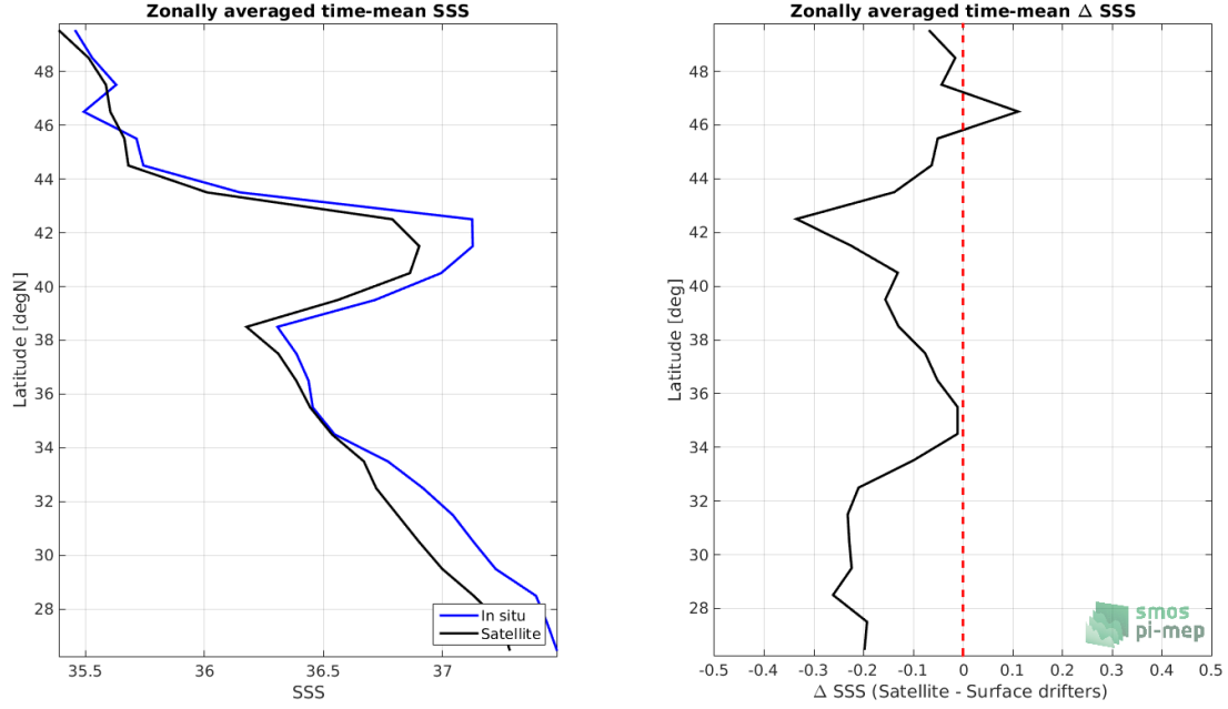
Figure 7: Left panel: Zonal mean SSS from SMOS L3 MED-ATL-OA v2 - 9 Days (BEC) satellite product (black) and from Surface drifters (blue). Right panel: Zonal mean of \Delta SSS (Satellite - Surface drifters) for all the collected Pi-MEP match-up pairs estimated over the full satellite product period.
