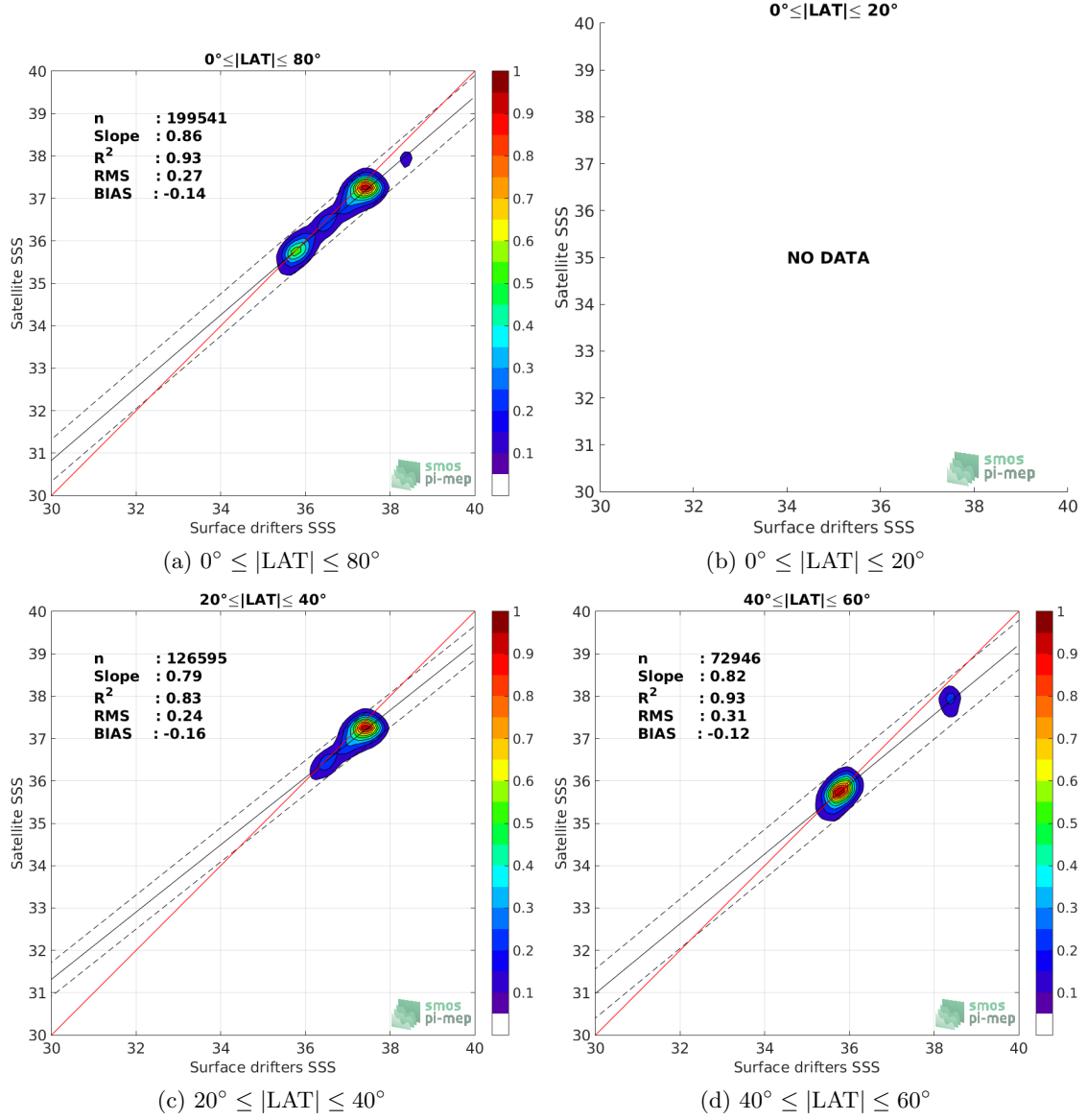
Figure 8: Contour maps of the concentration of SMOS L3 MED-ATL-OA v2 - 9 Days (BEC) SSS (y-axis) versus Surface drifters SSS (x-axis) at match-up pairs for different latitude bands. For each plot, the red line shows x=y . The black thin and dashed lines indicate a linear fit through the data cloud and the \pm 95\% confidence levels, respectively. The number match-up pairs n , the slope and R^2 coefficient of the linear fit, the root mean square (RMS) and the mean bias between satellite and in situ data are indicated for each latitude band in each plots.
