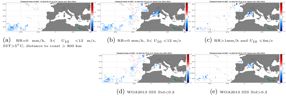
Figure 11: Temporal mean gridded over spatial boxes of size 1^\circ \times 1^\circ of \Delta SSS (SMOS L3 MED-ATL-OA v2 - 9 Days (BEC) - Surface drifters) for 5 different subdatasets corresponding to: RR=0 mm/h, 3 < U_{10} < 12 m/s, SST > 5^\circ\text{C} , distance to coast > 800 km (a), RR=0 mm/h, 3 < U_{10} < 12 m/s (b), RR > 1 mm/h and U_{10} < 4 m/s (c), WOA2013 SSS Std < 0.2 (d), WOA2013 SSS Std > 0.2 (e).
