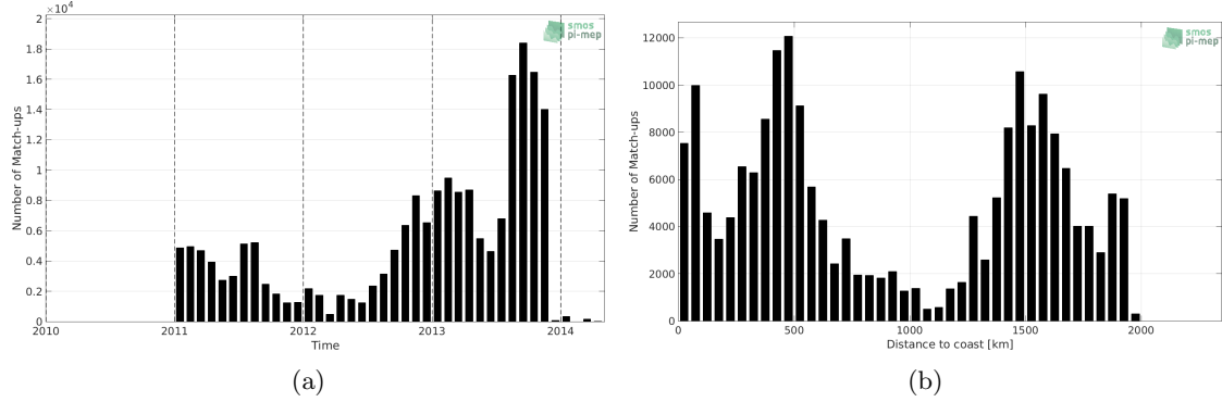
Figure 1: Number of match-ups between Surface drifters and SMOS L3 MED-ATL-OA v2 - 9 Days (BEC) SSS as a function of time (a) and as function of the distance to coast (b) over the Global Ocean Pi-MEP region and for the full satellite product period.
