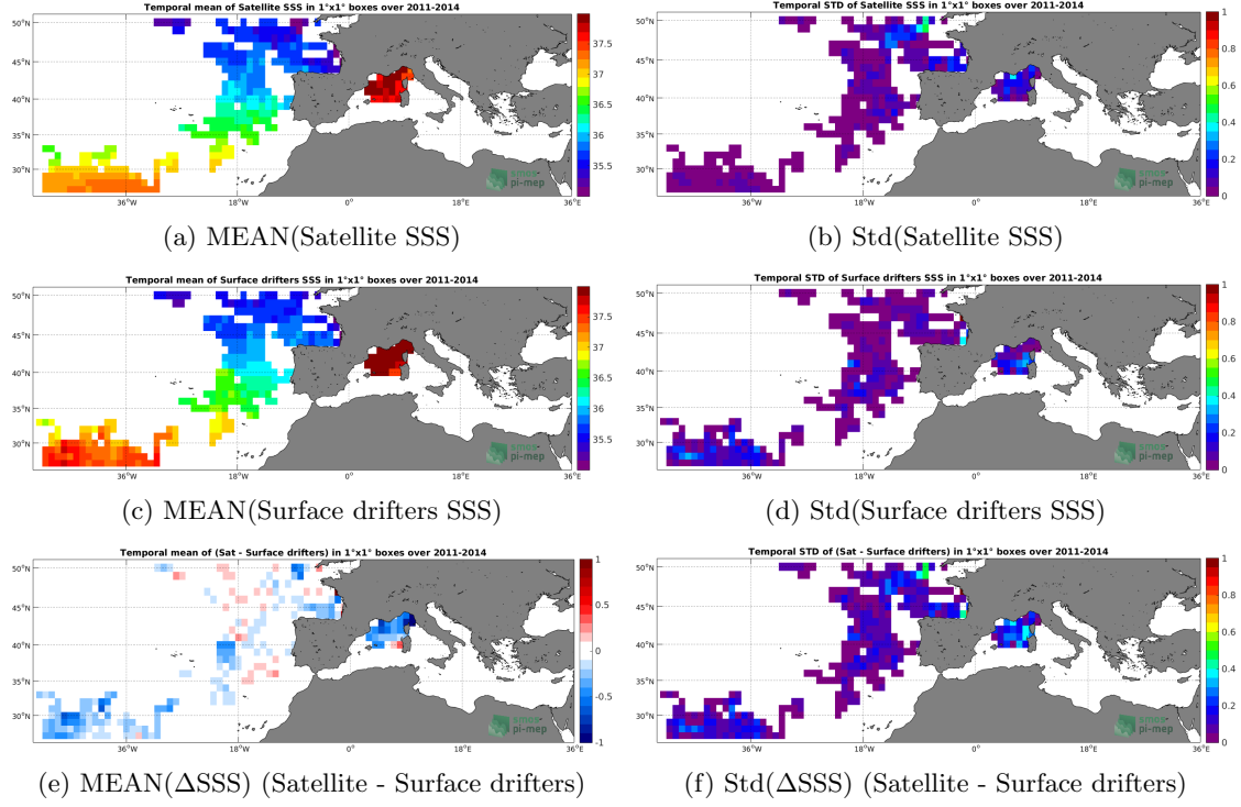
Figure 5: Temporal mean (left) and Std (right) of SSS from SMOS L3 MED-ATL-OA v2 - 9 Days (BEC) (top), Surface drifters (middle), and of \Delta SSS (Satellite - Surface drifters). Only match-up pairs are used to generate these maps.
