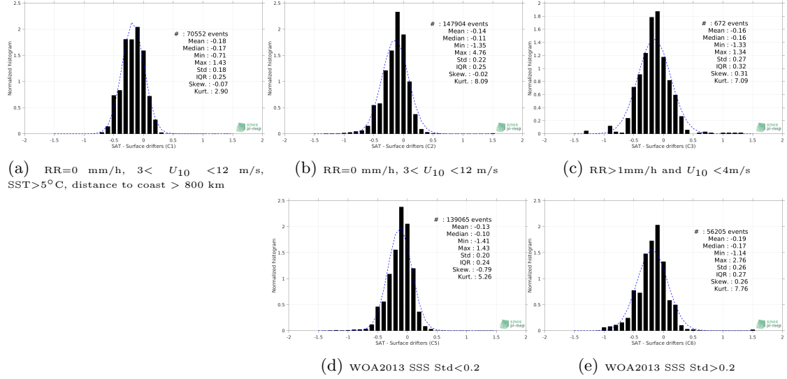
Figure 12: Normalized histogram of \Delta SSS (SMOS L3 MED-ATL-OA v2 - 9 Days (BEC) - Surface drifters) for 5 different subdatasets corresponding to: RR=0 mm/h, 3 < U_{10} < 12 m/s, SST > 5°C, distance to coast > 800 km (a), RR=0 mm/h, 3 < U_{10} < 12 m/s (b), RR > 1mm/h and U_{10} < 4 m/s (c), WOA2013 SSS Std < 0.2 (d), WOA2013 SSS Std > 0.2 (e).
