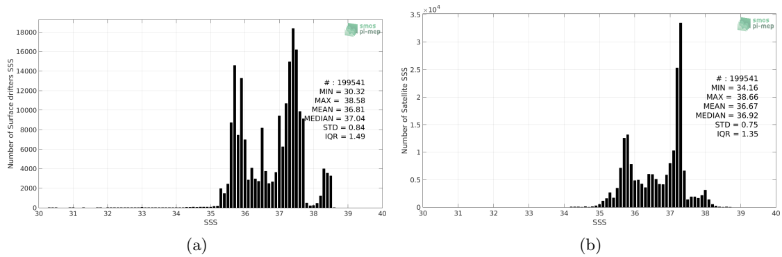
Figure 2: Histograms of SSS from Surface drifters (a) and SMOS L3 MED-ATL-OA v2 - 9 Days (BEC) (b) considering all match-up pairs per bins of 0.1 over the Global Ocean Pi-MEP region and for the full satellite product period.
