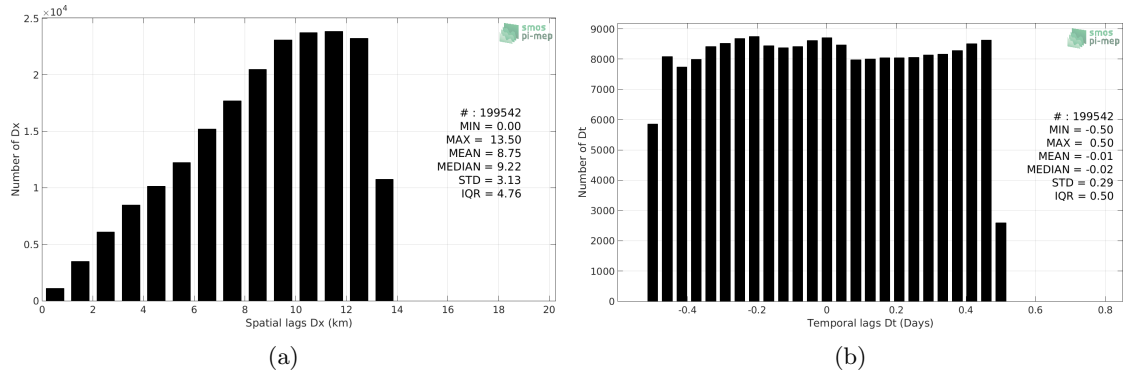
Figure 4: Histograms of the spatial (a) and temporal (b) lags between the time of the Surface drifters measurements and the date of the corresponding SMOS-L3-BEC-MED-ATL-OA-V2-9DAYS-0.25DEG SSS product.
