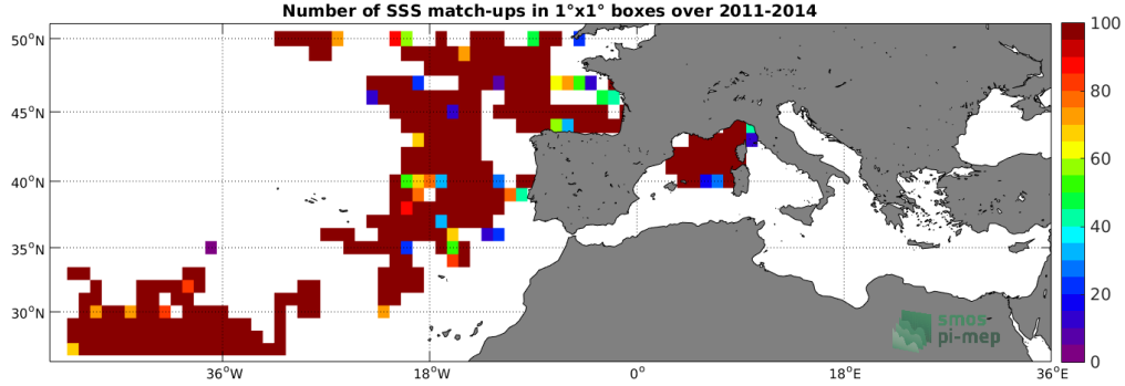
Figure 3: Number of SSS match-ups between Surface drifters SSS and the SMOS-L3-BEC-MED-ATL-OA-V2-9DAYS-0.25DEG SSS product for the Global Ocean Pi-MEP region over 1^\circ \times 1^\circ boxes and for the full satellite product period.
