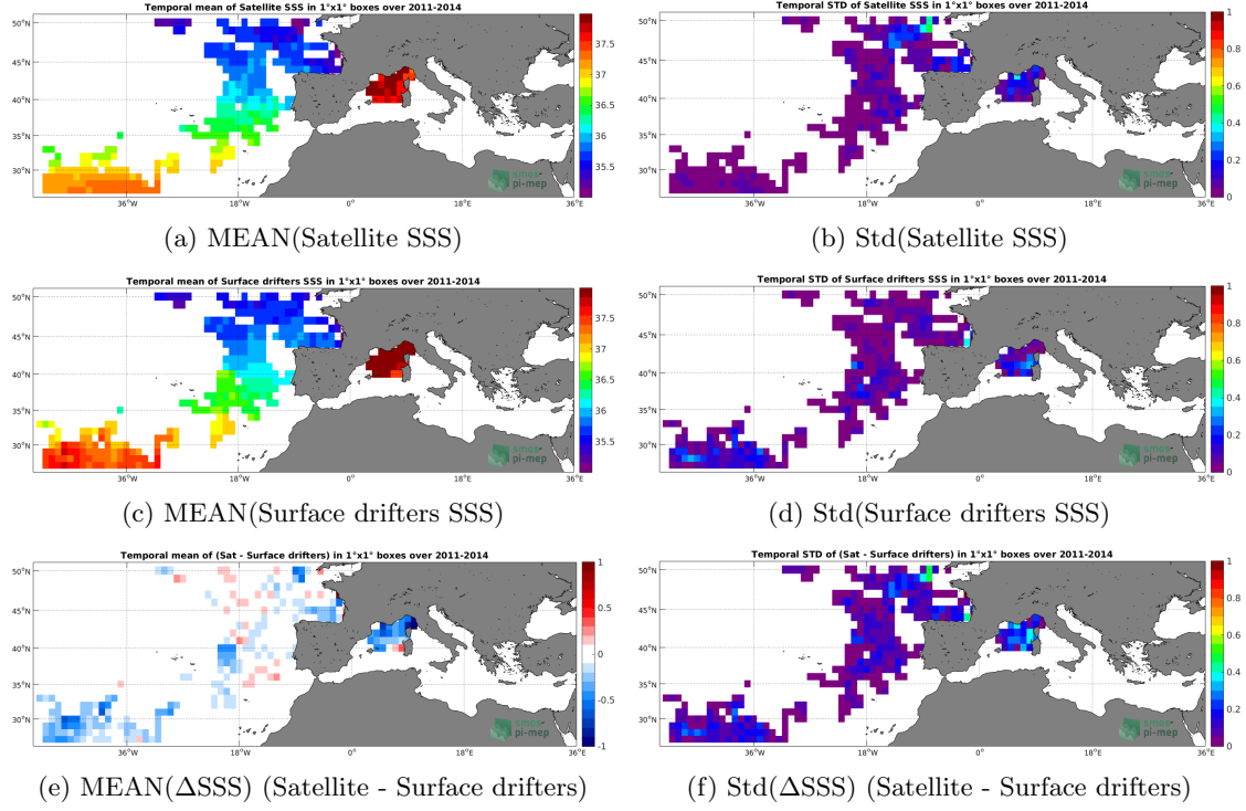
Figure 5: Temporal mean (left) and Std (right) of SSS from SMOS-L3-BEC-MED-ATL-OA-V2-9DAYS-0.25DEG (top), Surface drifters (middle), and of \Delta SSS (Satellite - Surface drifters). Only match-up pairs are used to generate these maps.
