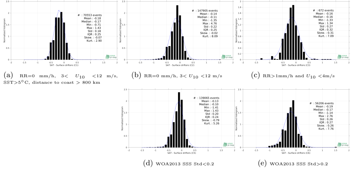
Figure 12: Normalized histogram of \Delta SSS (SMOS-L3-BEC-MED-ATL-OA-V2-9DAYS-0.25DEG - Surface drifters) for 5 different subdatasets corresponding to: RR=0 mm/h, 3 < U_{10} < 12 m/s, SST>5°C, distance to coast > 800 km (a), RR=0 mm/h, 3 < U_{10} < 12 m/s (b), RR>1mm/h and U_{10} < 4 m/s (c), WOA2013 SSS Std<0.2 (d), WOA2013 SSS Std>0.2 (e).
