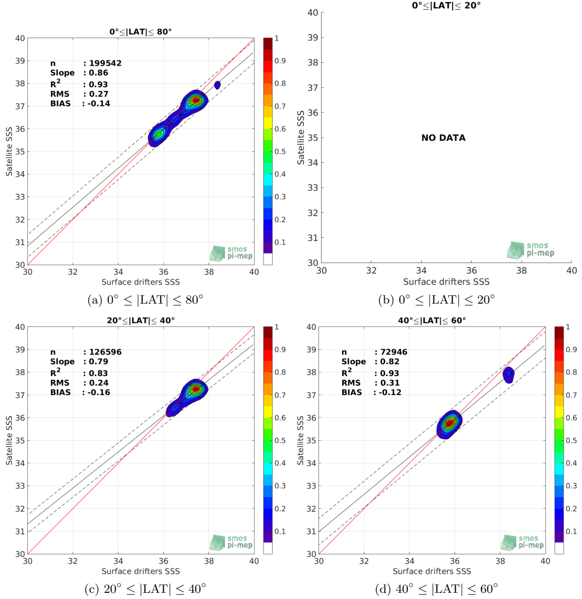
Figure 8: Contour maps of the concentration of SMOS-L3-BEC-MED-ATL-OA-V2-9DAYS-0.25DEG SSS (y-axis) versus Surface drifters SSS (x-axis) at match-up pairs for different latitude bands. For each plot, the red line shows x=y . The black thin and dashed lines indicate a linear fit through the data cloud and the \pm 95\% confidence levels, respectively. The number match-up pairs n , the slope and R^2 coefficient of the linear fit, the root mean square (RMS) and the mean bias between satellite and in situ data are indicated for each latitude band in each plots.
