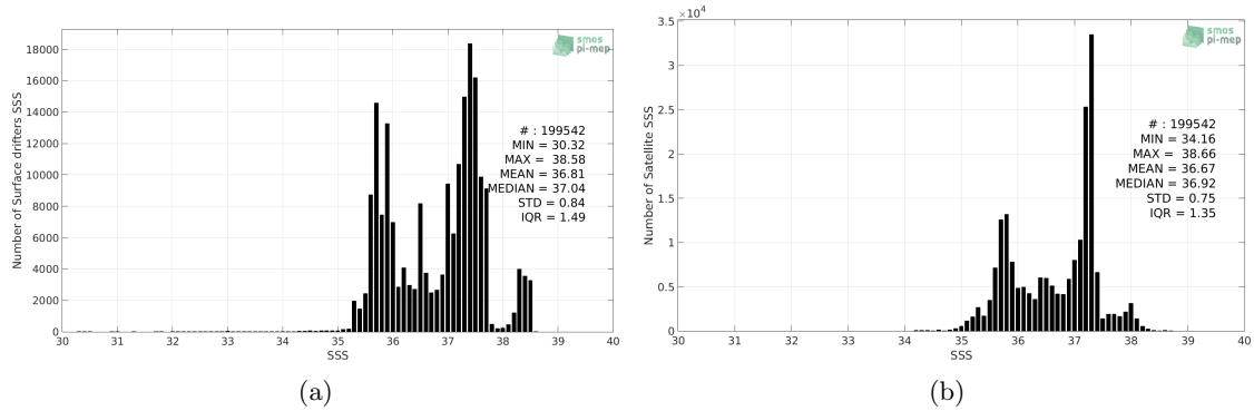
Figure 2: Histograms of SSS from Surface drifters (a) and SMOS-L3-BEC-MED-ATL-OA-V2-9DAYS-0.25DEG (b) considering all match-up pairs per bins of 0.1 over the Global Ocean Pi-MEP region and for the full satellite product period.
