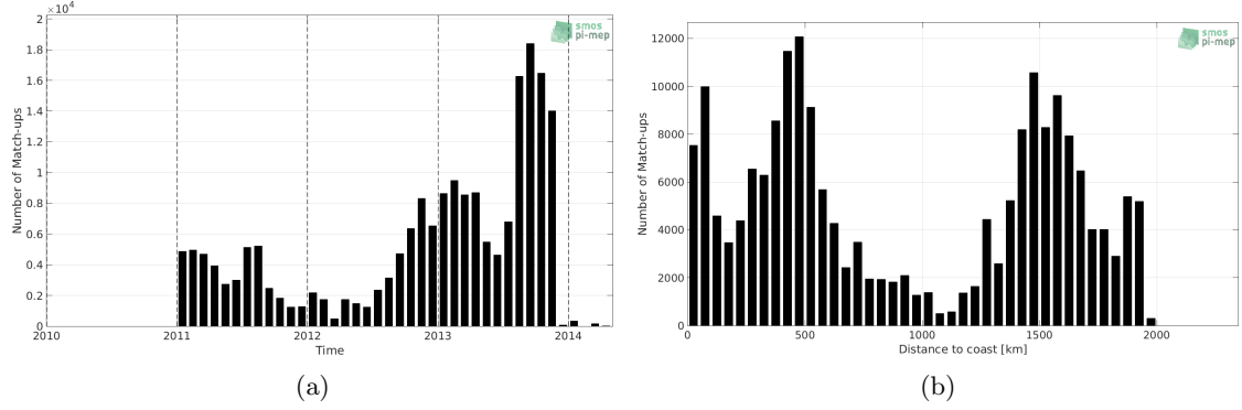
Figure 1: Number of match-ups between Surface drifters and SMOS-L3-BEC-MED-ATL-OA-V2-9DAYS-0.25DEG SSS as a function of time (a) and as function of the distance to coast (b) over the Global Ocean Pi-MEP region and for the full satellite product period.
