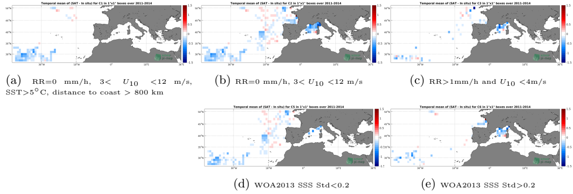
Figure 11: Temporal mean gridded over spatial boxes of size 1^\circ \times 1^\circ of \Delta SSS (SMOS-L3-BEC-MED-ATL-OA-V2-9DAYS-0.25DEG - Surface drifters) for 5 different subdatasets corresponding to: RR=0 mm/h, 3 < U_{10} < 12 m/s, SST > 5^\circ C , distance to coast > 800 km (a), RR=0 mm/h, 3 < U_{10} < 12 m/s (b), RR > 1 mm/h and U_{10} < 4 m/s (c), WOA2013 SSS Std < 0.2 (d), WOA2013 SSS Std > 0.2 (e).
