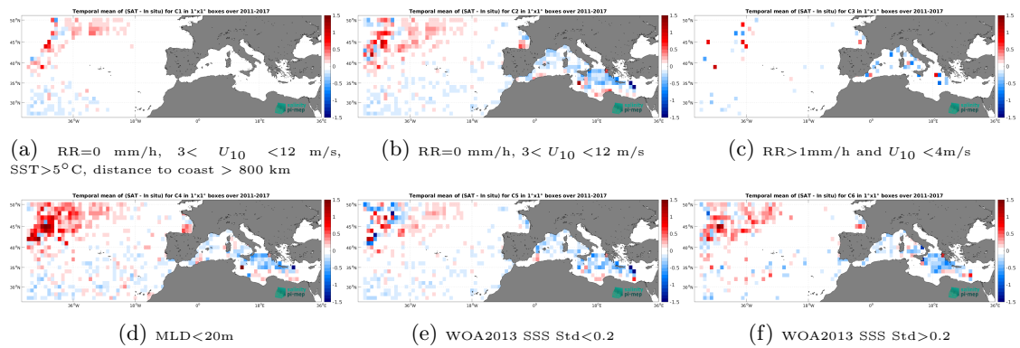
Figure 14: Temporal mean gridded over spatial boxes of size 1^\circ \times 1^\circ of \Delta SSS (SMOS SSS L3 MED-ATL-OA v2 - 9 Days (BEC) - Argo) for 6 different subdatasets corresponding to:RR=0 mm/h, 3 < U_{10} < 12 m/s, SST >5^\circ C, distance to coast > 800 km (a), RR=0 mm/h, 3 < U_{10} < 12 m/s (b), RR >1 mm/h and U_{10} < 4 m/s (c),MLD <20 m (d),WOA2013 SSS Std <0.2 (e),WOA2013 SSS Std >0.2 (f).
