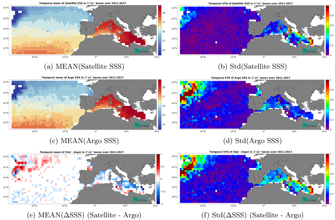
Figure 7: Temporal mean (left) and Std (right) of SSS from SMOS SSS L3 MED-ATL-OA v2 - 9 Days (BEC) (top), Argo (middle), and of \Delta SSS (Satellite - Argo). Only match-up pairs are used to generate these maps.
