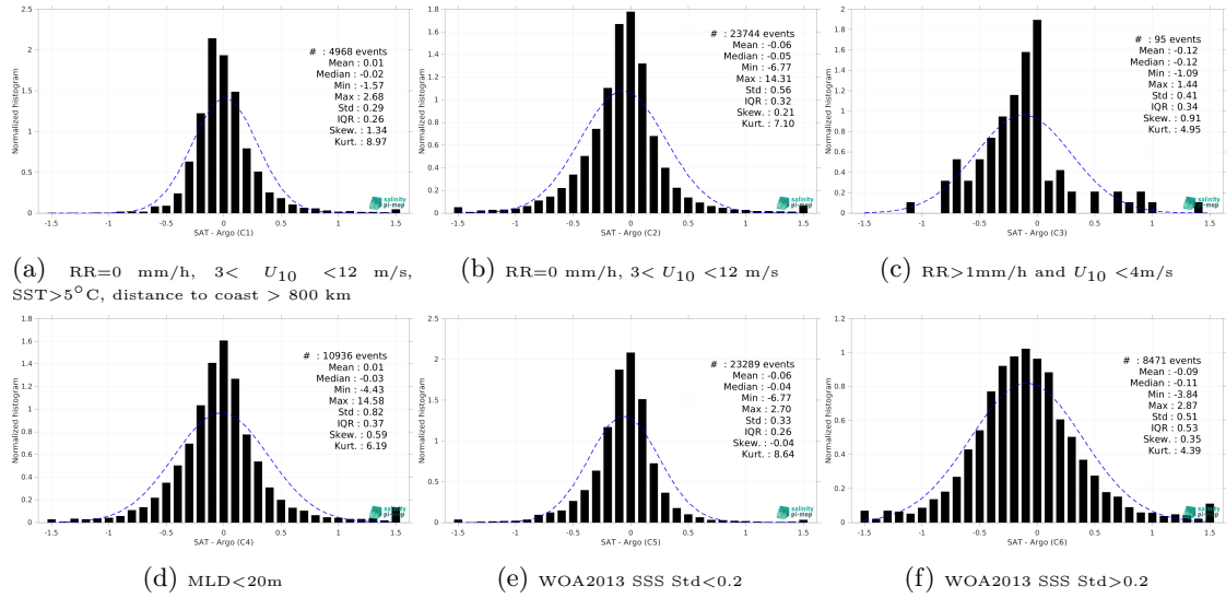
Figure 15: Normalized histogram of \Delta SSS (SMOS SSS L3 MED-ATL-OA v2 - 9 Days (BEC) - Argo) for 6 different subdatasets corresponding to: RR=0 mm/h, 3 < U_{10} < 12 m/s, SST>5°C, distance to coast > 800 km (a), RR=0 mm/h, 3 < U_{10} < 12 m/s (b), RR>1mm/h and U_{10} < 4 m/s (c), MLD<20m (d), WOA2013 SSS Std<0.2 (e), WOA2013 SSS Std>0.2 (f).
