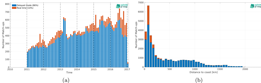
Figure 2: Number of match-ups between Argo and SMOS SSS L3 MED-ATL-OA v2 - 9 Days (BEC) SSS as a function of time (a) and as function of the distance to coast (b) over the Global Ocean Pi-MEP region and for the full satellite product period.
