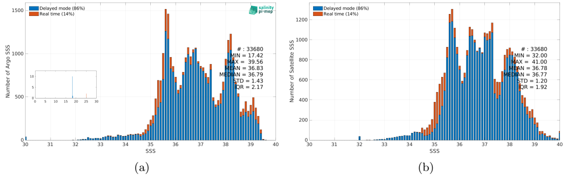
Figure 3: Histograms of SSS from Argo (a) and SMOS SSS L3 MED-ATL-OA v2 - 9 Days (BEC) (b) considering all match-up pairs per bins of 0.1 over the Global Ocean Pi-MEP region and for the full satellite product period.
