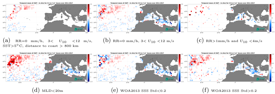
Figure 12: Temporal mean gridded over spatial boxes of size 1^\circ \times 1^\circ of \Delta SSS (SMOS SSS L3 MED-ATL-OA v2 - 9 Days (BEC) - Argo) for 6 different subdatasets corresponding to:RR=0 mm/h, 3 < U_{10} < 12 m/s, SST >5^\circ C, distance to coast > 800 km (a), RR=0 mm/h, 3 < U_{10} < 12 m/s (b), RR >1 mm/h and U_{10} < 4 m/s (c),MLD <20 m (d),WOA2013 SSS Std <0.2 (e),WOA2013 SSS Std >0.2 (f).
