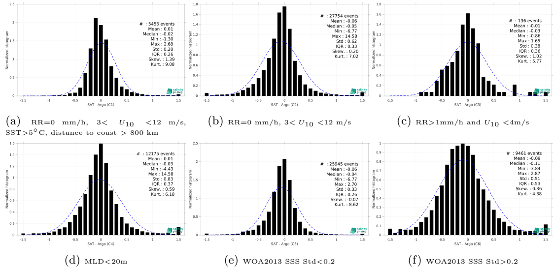
Figure 13: Normalized histogram of \Delta SSS (SMOS SSS L3 MED-ATL-OA v2 - 9 Days (BEC) - Argo) for 6 different subdatasets corresponding to: RR=0 mm/h, 3 < U_{10} < 12 m/s, SST > 5°C, distance to coast > 800 km (a), RR=0 mm/h, 3 < U_{10} < 12 m/s (b), RR > 1mm/h and U_{10} < 4 m/s (c), MLD < 20m (d), WOA2013 SSS Std < 0.2 (e), WOA2013 SSS Std > 0.2 (f).
