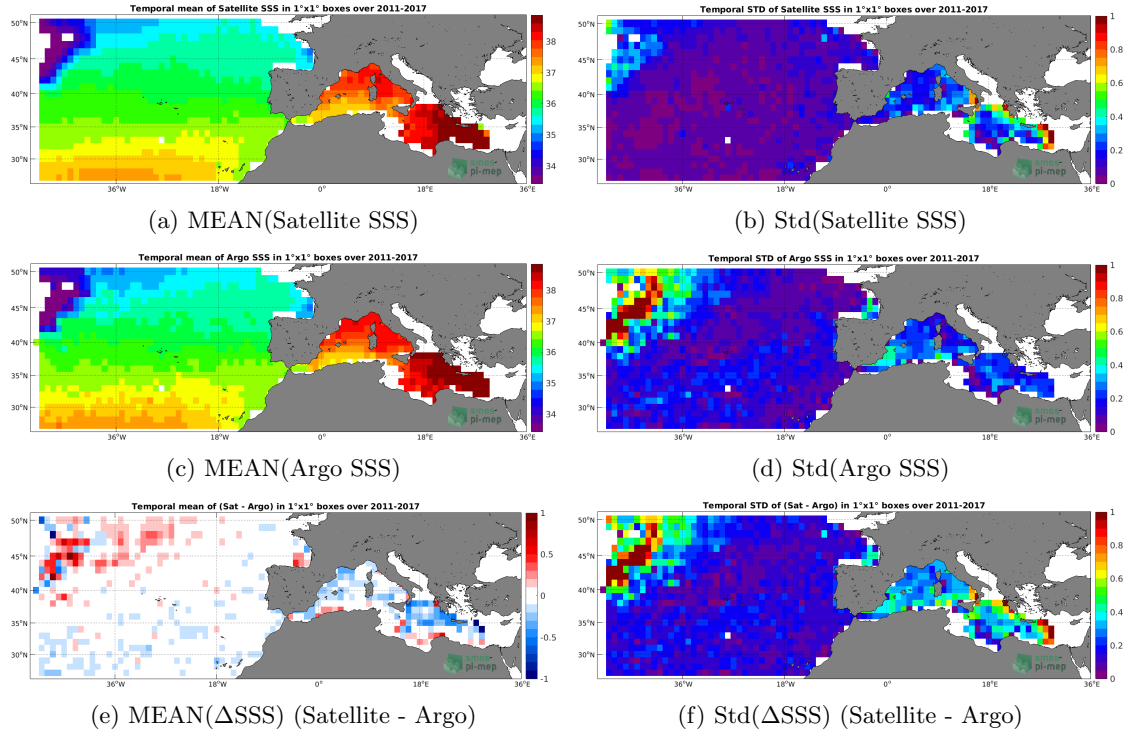
Figure 6: Temporal mean (left) and Std (right) of SSS from SMOS SSS L3 MED-ATL-OA v2 - 9 Days (BEC) (top), Argo (middle), and of \Delta SSS (Satellite - Argo). Only match-up pairs are used to generate these maps.
