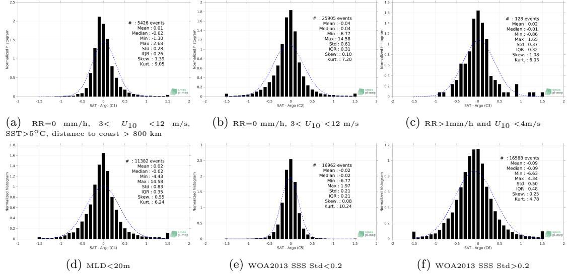
Figure 13: Normalized histogram of \Delta SSS (SMOS SSS L3 MED-ATL-OA v2 - 9 Days (BEC) - Argo) for 6 different subdatasets corresponding to: RR=0 mm/h, 3 < U_{10} < 12 m/s, SST>5°C, distance to coast > 800 km (a), RR=0 mm/h, 3 < U_{10} < 12 m/s (b), RR>1mm/h and U_{10} < 4 m/s (c), MLD<20m (d), WOA2013 SSS Std<0.2 (e), WOA2013 SSS Std>0.2 (f).
