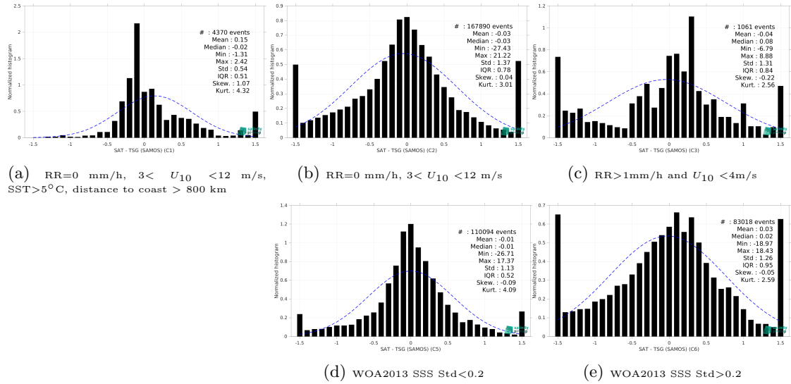
Figure 15: Normalized histogram of \Delta SSS (SMOS SSS L3 Arctic v4 - 9 Days (BEC) - TSG (SAMOS)) for 5 different subdatasets corresponding to: RR=0 mm/h, 3 < U_{10} < 12 m/s, SST>5°C, distance to coast > 800 km (a), RR=0 mm/h, 3 < U_{10} < 12 m/s (b), RR>1mm/h and U_{10} < 4 m/s (c), WOA2013 SSS Std<0.2 (d), WOA2013 SSS Std>0.2 (e).
