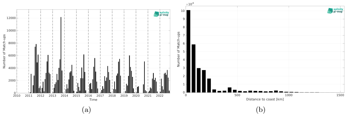
Figure 2: Number of match-ups between TSG (SAMOS) and SMOS SSS L3 Arctic v4 - 9 Days (BEC) SSS as a function of time (a) and as function of the distance to coast (b) over the Global Ocean Pi-MEP region and for the full satellite product period.
