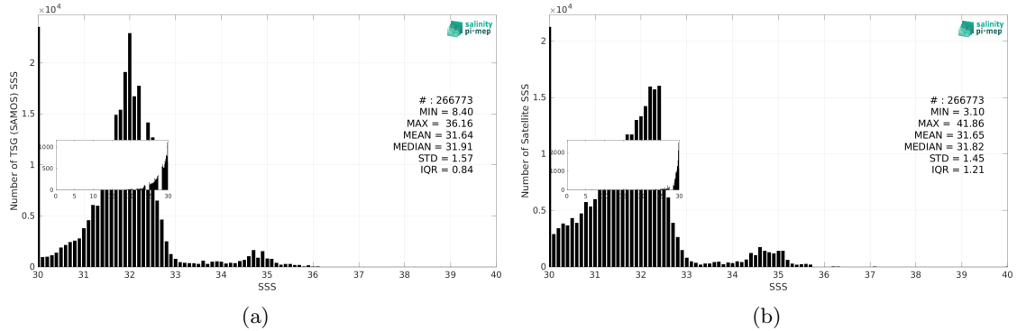
Figure 3: Histograms of SSS from TSG (SAMOS) (a) and SMOS SSS L3 Arctic v4 - 9 Days (BEC) (b) considering all match-up pairs per bins of 0.1 over the Global Ocean Pi-MEP region and for the full satellite product period.
