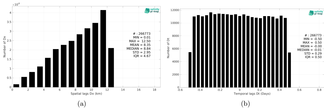
Figure 6: Histograms of the spatial (a) and temporal (b) lags between the location/time of the TSG (SAMOS) measurement and the date of the corresponding SMOS SSS L3 Arctic v4 - 9 Days (BEC) SSS pixel.
