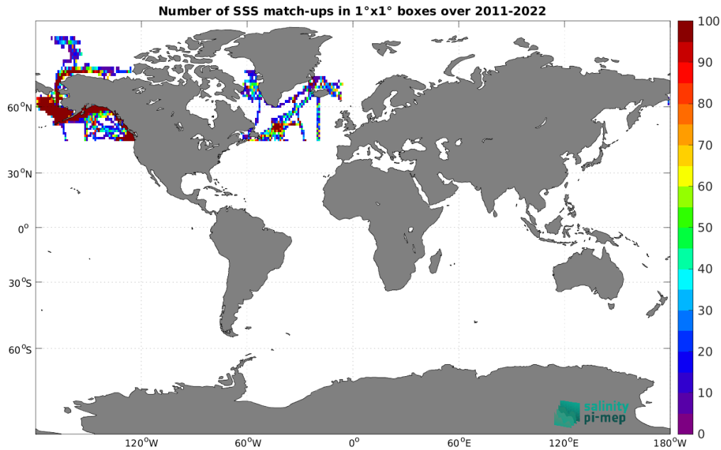
Figure 5: Number of SSS match-ups between TSG (SAMOS) SSS and the SMOS SSS L3 Arctic v4 - 9 Days (BEC) SSS product for the Global Ocean Pi-MEP region over 1^\circ \times 1^\circ boxes and for the full satellite product period.
