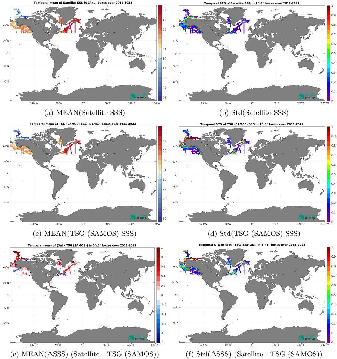
Figure 7: Temporal mean (left) and Std (right) of SSS from SMOS SSS L3 Arctic v4 - 9 Days (BEC) (top), TSG (SAMOS) (middle), and of \Delta SSS (Satellite - TSG (SAMOS)). Only match-up pairs are used to generate these maps.
