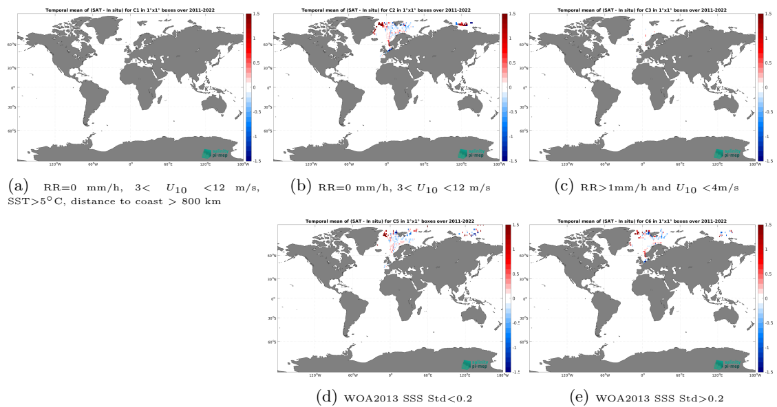
Figure 14: Temporal mean gridded over spatial boxes of size 1^\circ \times 1^\circ of \Delta SSS (SMOS SSS L3 Arctic v4 - 9 Days (BEC) - TSG (Polarstern)) for 5 different subdatasets corresponding to:RR=0 mm/h, 3 < U_{10} < 12 m/s, SST > 5°C, distance to coast > 800 km (a), RR=0 mm/h, 3 < U_{10} < 12 m/s (b), RR > 1mm/h and U_{10} < 4 m/s (c), WOA2013 SSS Std < 0.2 (d), WOA2013 SSS Std > 0.2 (e).
