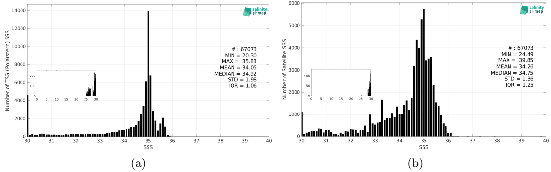
Figure 3: Histograms of SSS from TSG (Polarstern) (a) and SMOS SSS L3 Arctic v4 - 9 Days (BEC) (b) considering all match-up pairs per bins of 0.1 over the Global Ocean Pi-MEP region and for the full satellite product period.
