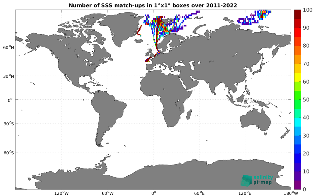
Figure 5: Number of SSS match-ups between TSG (Polarstern) SSS and the SMOS SSS L3 Arctic v4 - 9 Days (BEC) SSS product for the Global Ocean Pi-MEP region over 1°x1° boxes and for the full satellite product period.
