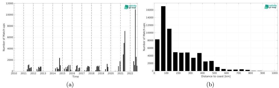
Figure 2: Number of match-ups between TSG (Polarstern) and SMOS SSS L3 Arctic v4 - 9 Days (BEC) SSS as a function of time (a) and as function of the distance to coast (b) over the Global Ocean Pi-MEP region and for the full satellite product period.
