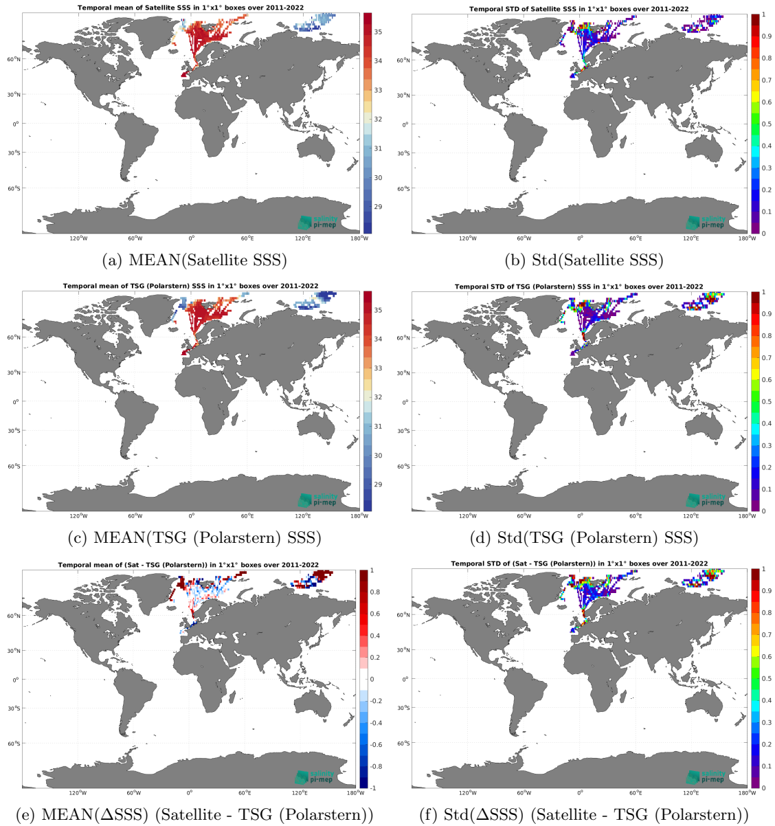
Figure 7: Temporal mean (left) and Std (right) of SSS from SMOS SSS L3 Arctic v4 - 9 Days (BEC) (top), TSG (Polarstern) (middle), and of \Delta SSS (Satellite - TSG (Polarstern)). Only match-up pairs are used to generate these maps.
