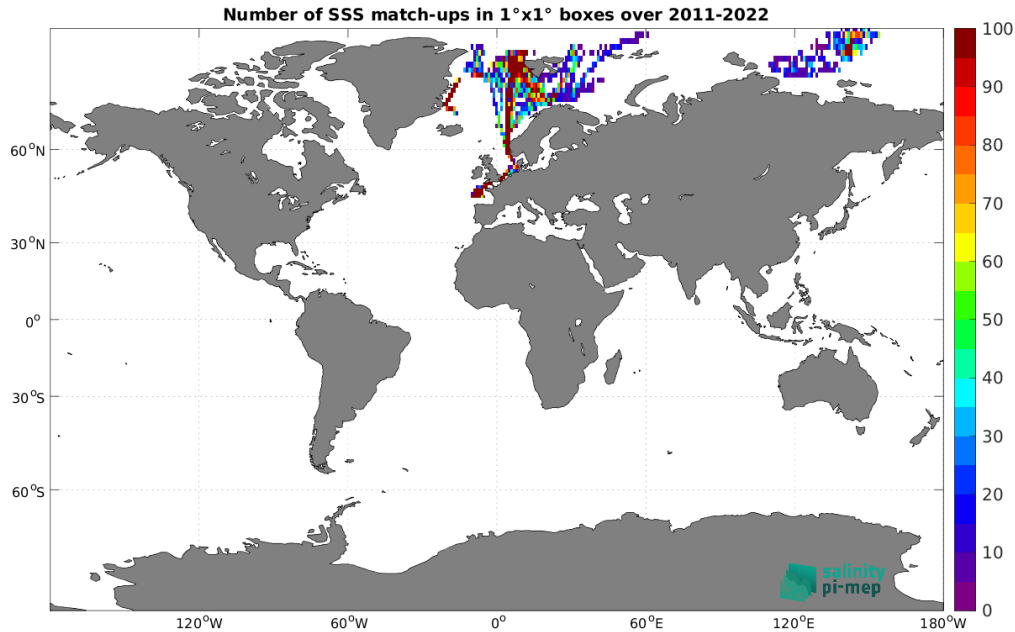
Figure 5: Number of SSS match-ups between TSG (Polarstern) SSS and the SMOS SSS L3 Arctic v4 - 9 Days (BEC) SSS product for the Global Ocean Pi-MEP region over 1^\circ \times 1^\circ boxes and for the full satellite product period.
