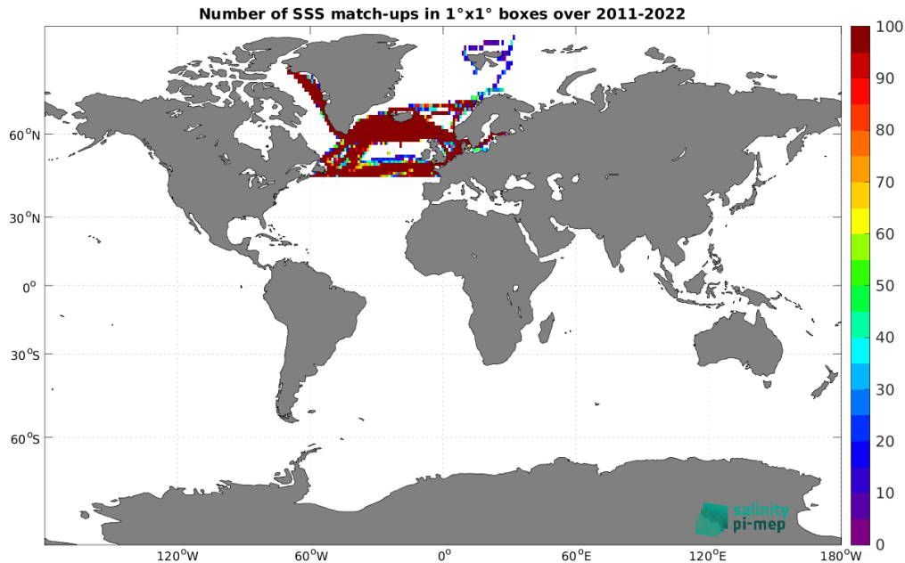
Figure 5: Number of SSS match-ups between TSG (LEGOS-DM) SSS and the SMOS SSS L3 Arctic v4 - 9 Days (BEC) SSS product for the Global Ocean Pi-MEP region over 1°x1° boxes and for the full satellite product period.
