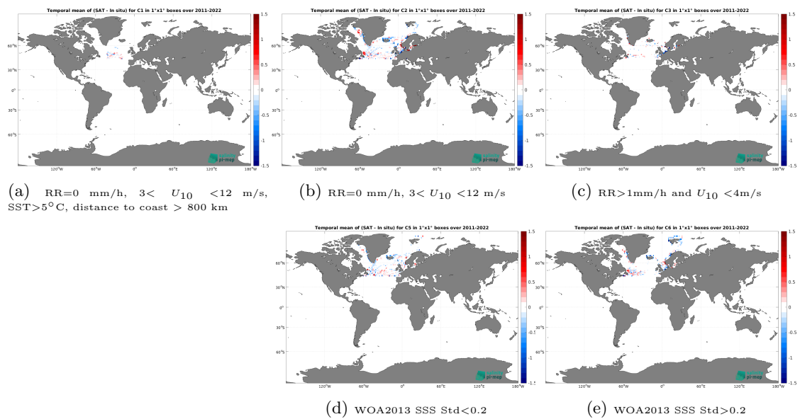
Figure 14: Temporal mean gridded over spatial boxes of size 1^\circ \times 1^\circ of \Delta SSS (SMOS SSS L3 Arctic v4 - 9 Days (BEC) - TSG (LEGOS-DM)) for 5 different subdatasets corresponding to:RR=0 mm/h, 3 < U_{10} < 12 m/s, SST > 5^\circ\text{C} , distance to coast > 800 km (a), RR=0 mm/h, 3 < U_{10} < 12 m/s (b), RR > 1 mm/h and U_{10} < 4 m/s (c), WOA2013 SSS Std < 0.2 (d), WOA2013 SSS Std > 0.2 (e).
