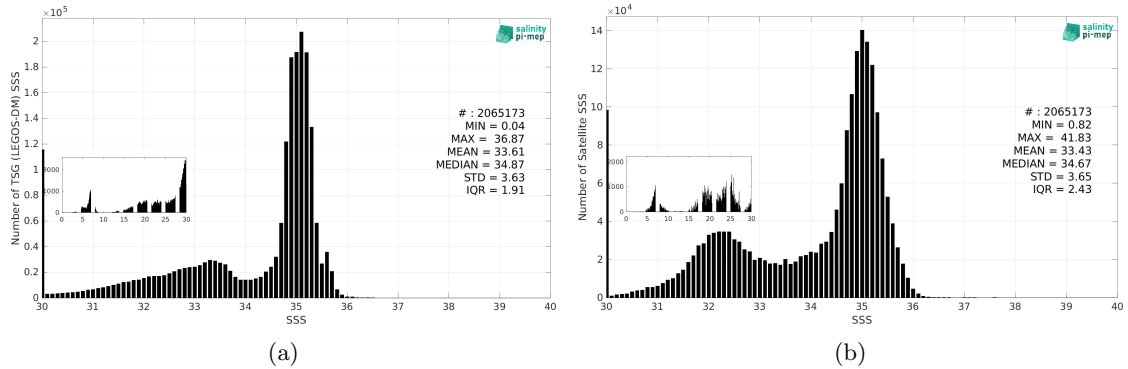
Figure 3: Histograms of SSS from TSG (LEGOS-DM) (a) and SMOS SSS L3 Arctic v4 - 9 Days (BEC) (b) considering all match-up pairs per bins of 0.1 over the Global Ocean Pi-MEP region and for the full satellite product period.
