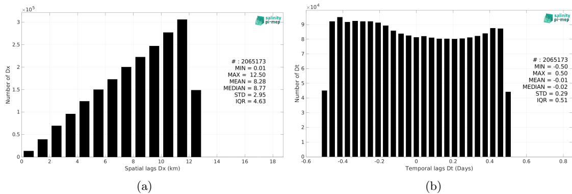
Figure 6: Histograms of the spatial (a) and temporal (b) lags between the location/time of the TSG (LEGOS-DM) measurement and the date of the corresponding SMOS SSS L3 Arctic v4 - 9 Days (BEC) SSS pixel.
