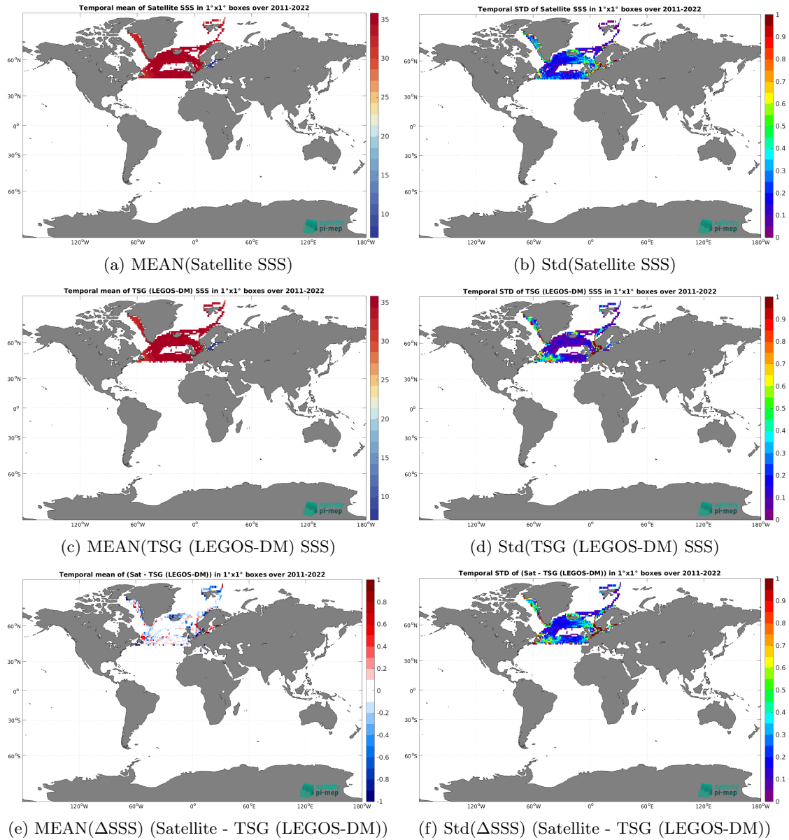
Figure 7: Temporal mean (left) and Std (right) of SSS from SMOS SSS L3 Arctic v4 - 9 Days (BEC) (top), TSG (LEGOS-DM) (middle), and of \Delta SSS (Satellite - TSG (LEGOS-DM)). Only match-up pairs are used to generate these maps.
