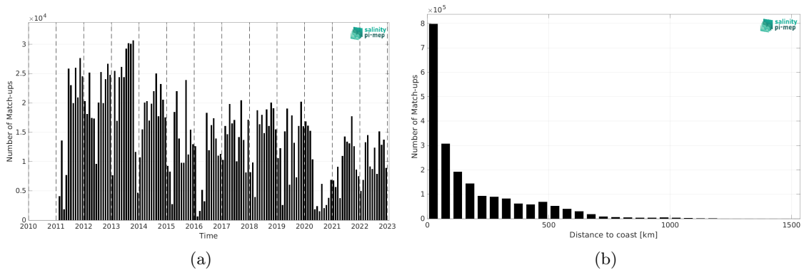
Figure 2: Number of match-ups between TSG (LEGOS-DM) and SMOS SSS L3 Arctic v4 - 9 Days (BEC) SSS as a function of time (a) and as function of the distance to coast (b) over the Global Ocean Pi-MEP region and for the full satellite product period.
