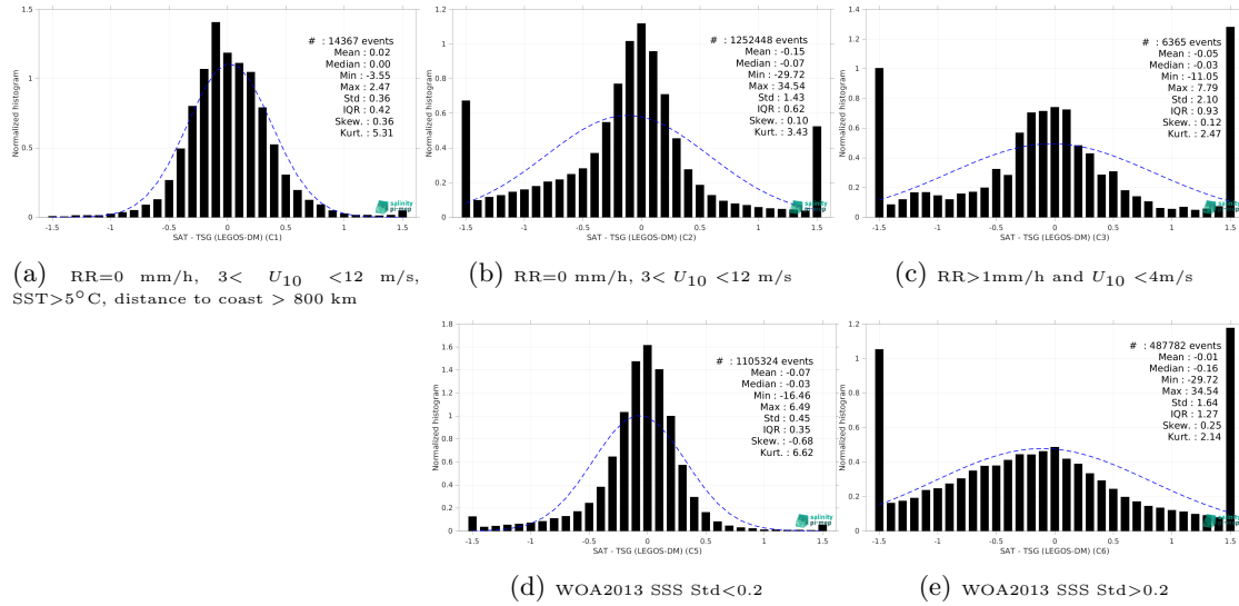
Figure 15: Normalized histogram of \Delta\text{SSS} (SMOS SSS L3 Arctic v4 - 9 Days (BEC) - TSG (LEGOS-DM)) for 5 different subdatasets corresponding to: RR=0 mm/h, 3 < U_{10} < 12 m/s, SST>5°C, distance to coast > 800 km (a), RR=0 mm/h, 3 < U_{10} < 12 m/s (b), RR>1mm/h and U_{10} < 4 m/s (c), WOA2013 SSS Std<0.2 (d), WOA2013 SSS Std>0.2 (e).
