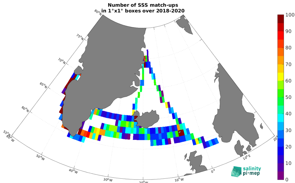
Figure 5: Number of SSS match-ups between TSG (Lauge-Koch) SSS and the SMOS SSS L3 Arctic v4 - 9 Days (BEC) SSS product for the Global Ocean Pi-MEP region over 1^\circ \times 1^\circ boxes and for the full satellite product period.
