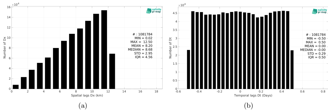
Figure 6: Histograms of the spatial (a) and temporal (b) lags between the location/time of the TSG (GOSUD-Research-vessel) measurement and the date of the corresponding SMOS SSS L3 Arctic v4 - 9 Days (BEC) SSS pixel.
