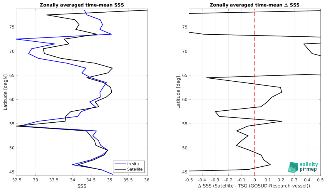
Figure 9: Left panel: Zonal mean SSS from SMOS SSS L3 Arctic v4 - 9 Days (BEC) satellite product (black) and from TSG (GOSUD-Research-vessel) (blue). Right panel: Zonal mean of \Delta SSS (Satellite - TSG (GOSUD-Research-vessel)) for all the collected Pi-MEP match-up pairs estimated over the full satellite product period.
