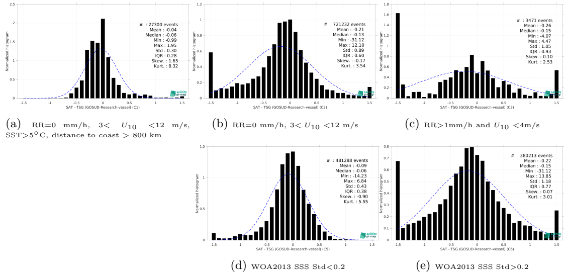
Figure 15: Normalized histogram of \Delta SSS (SMOS SSS L3 Arctic v4 - 9 Days (BEC) - TSG (GOSUD-Research-vessel)) for 5 different subdatasets corresponding to: RR=0 mm/h, 3 < U_{10} < 12 m/s, SST>5°C, distance to coast > 800 km (a), RR=0 mm/h, 3 < U_{10} < 12 m/s (b), RR>1mm/h and U_{10} < 4 m/s (c), WOA2013 SSS Std<0.2 (d), WOA2013 SSS Std>0.2 (e).
