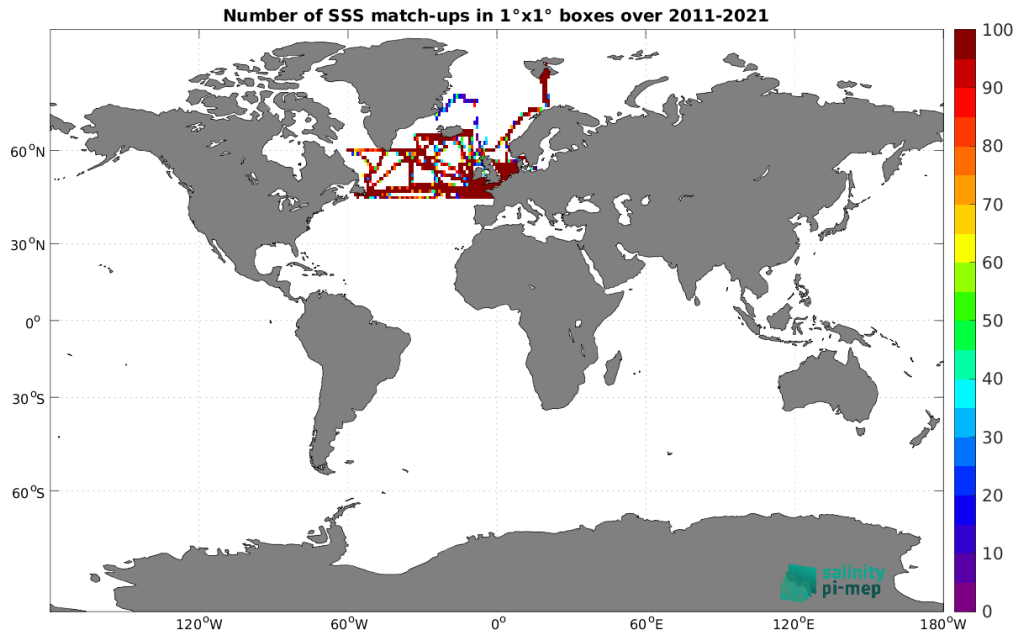
Figure 5: Number of SSS match-ups between TSG (GOSUD-Research-vessel) SSS and the SMOS SSS L3 Arctic v4 - 9 Days (BEC) SSS product for the Global Ocean Pi-MEP region over 1^\circ \times 1^\circ boxes and for the full satellite product period.
