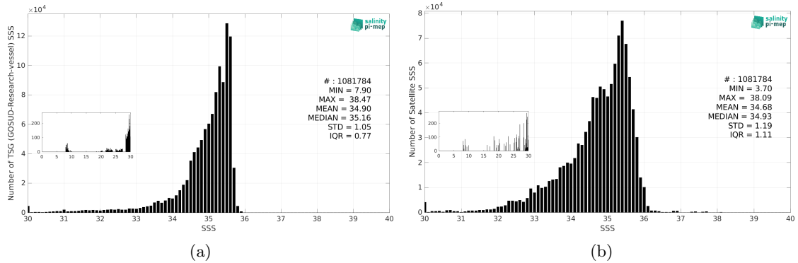
Figure 3: Histograms of SSS from TSG (GOSUD-Research-vessel) (a) and SMOS SSS L3 Arctic v4 - 9 Days (BEC) (b) considering all match-up pairs per bins of 0.1 over the Global Ocean Pi-MEP region and for the full satellite product period.
