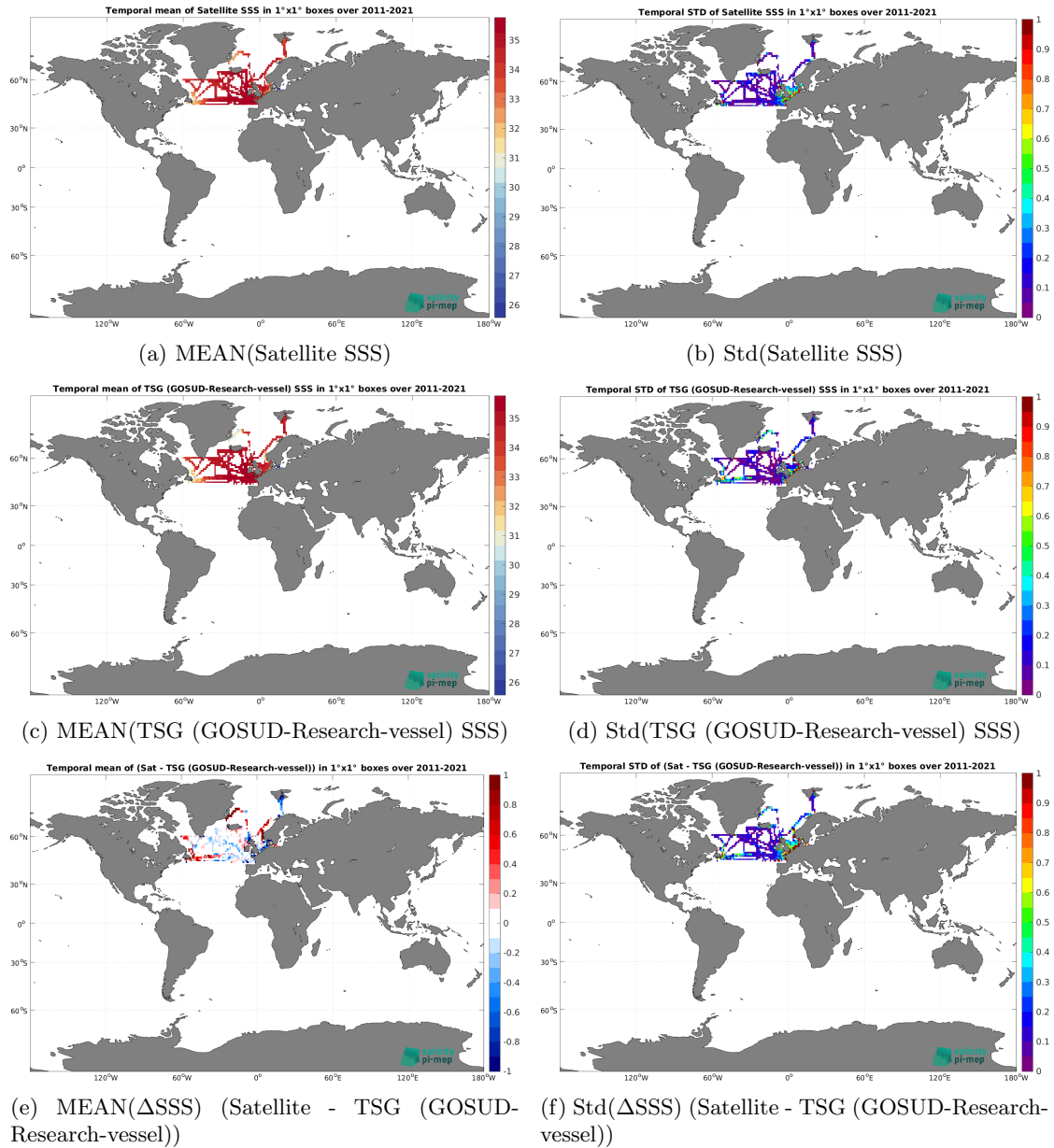
Figure 7: Temporal mean (left) and Std (right) of SSS from SMOS SSS L3 Arctic v4 - 9 Days (BEC) (top), TSG (GOSUD-Research-vessel) (middle), and of \Delta SSS (Satellite - TSG (GOSUD-Research-vessel)). Only match-up pairs are used to generate these maps.
