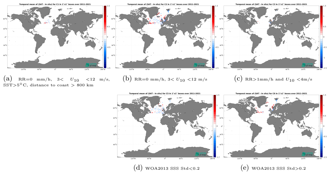
Figure 14: Temporal mean gridded over spatial boxes of size 1^\circ \times 1^\circ of \Delta SSS (SMOS SSS L3 Arctic v4 - 9 Days (BEC) - TSG (GOSUD-Research-vessel)) for 5 different subdatasets corresponding to: RR=0 mm/h, 3 < U_{10} < 12 m/s, SST > 5^\circ\text{C} , distance to coast > 800 km (a), RR=0 mm/h, 3 < U_{10} < 12 m/s (b), RR > 1 mm/h and U_{10} < 4 m/s (c), WOA2013 SSS Std < 0.2 (d), WOA2013 SSS Std > 0.2 (e).
