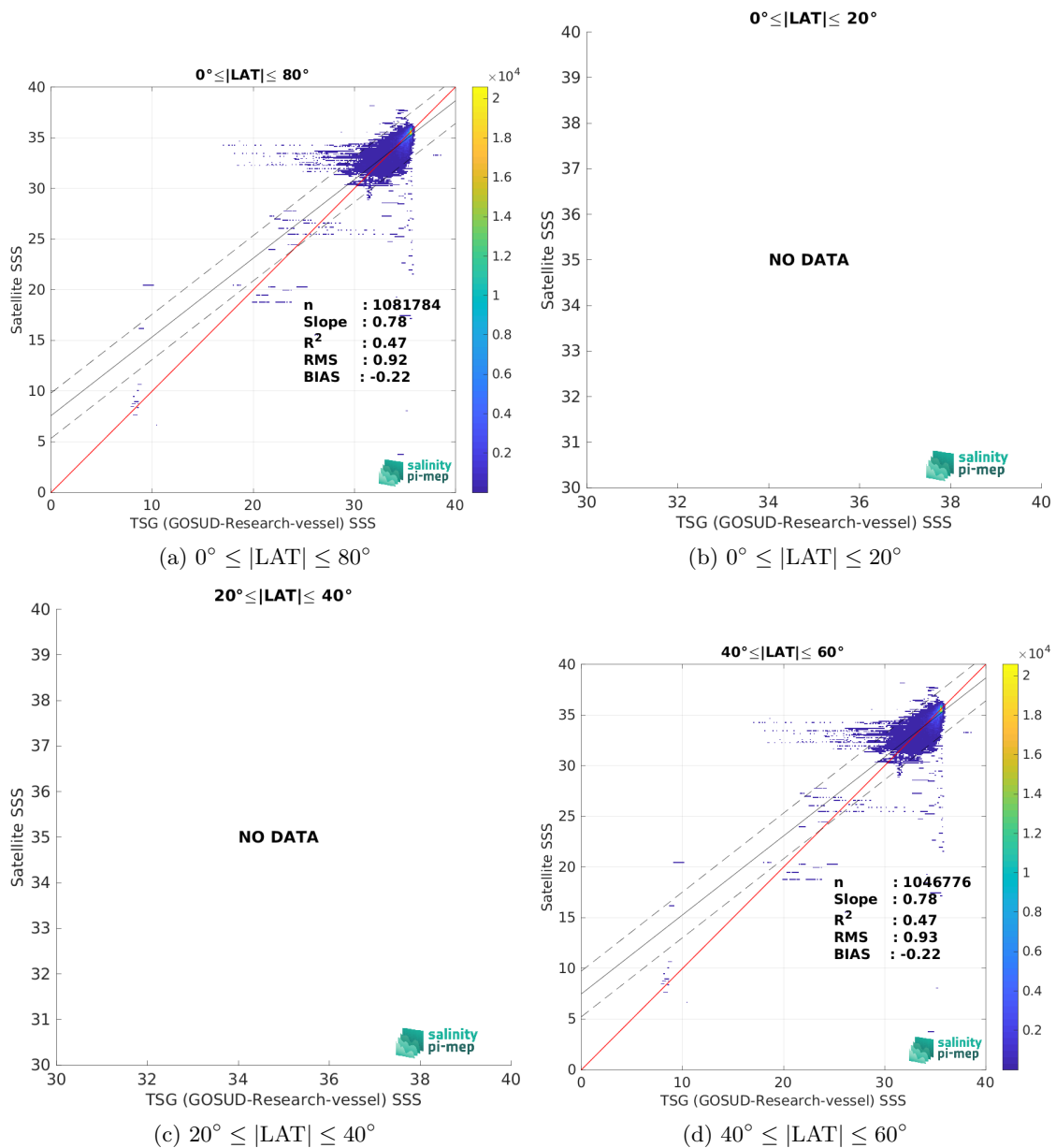
Figure 10: Contour maps of the concentration of SMOS SSS L3 Arctic v4 - 9 Days (BEC) SSS (y-axis) versus TSG (GOSUD-Research-vessel) SSS (x-axis) at match-up pairs for different latitude bands. For each plot, the red line shows x=y . The black thin and dashed lines indicate a linear fit through the data cloud and the \pm 95\% confidence levels, respectively. The number match-up pairs n , the slope and R^2 coefficient of the linear fit, the root mean square (RMS) and the mean bias between satellite and in situ data are indicated for each latitude band in each plots.
