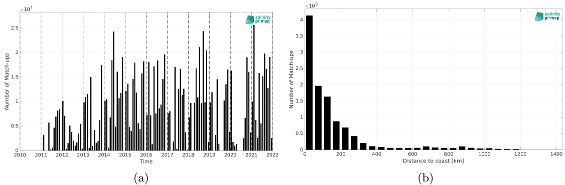
Figure 2: Number of match-ups between TSG (GOSUD-Research-vessel) and SMOS SSS L3 Arctic v4 - 9 Days (BEC) SSS as a function of time (a) and as function of the distance to coast (b) over the Global Ocean Pi-MEP region and for the full satellite product period.
