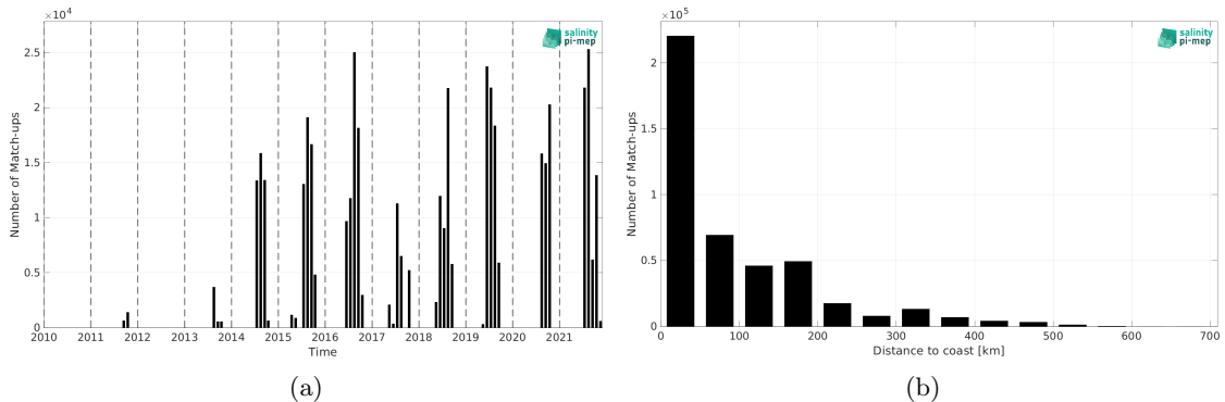
Figure 2: Number of match-ups between TSG (Amundsen) and SMOS SSS L3 Arctic v4 - 9 Days (BEC) SSS as a function of time (a) and as function of the distance to coast (b) over the Global Ocean Pi-MEP region and for the full satellite product period.
