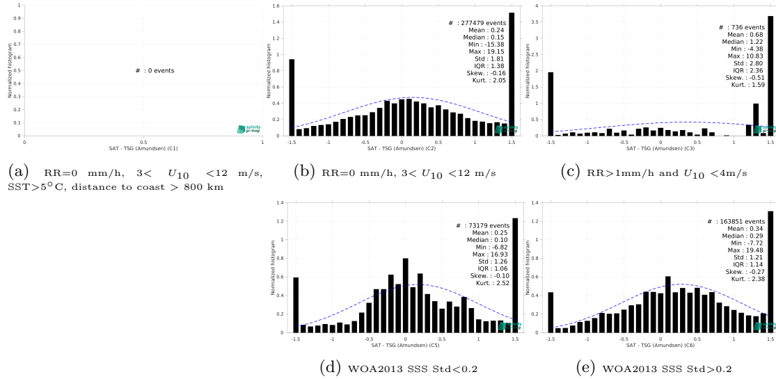
Figure 15: Normalized histogram of \Delta SSS (SMOS SSS L3 Arctic v4 - 9 Days (BEC) - TSG (Amundsen)) for 5 different subdatasets corresponding to: RR=0 mm/h, 3 < U_{10} < 12 m/s, SST > 5°C, distance to coast > 800 km (a), RR=0 mm/h, 3 < U_{10} < 12 m/s (b), RR > 1mm/h and U_{10} < 4 m/s (c), WOA2013 SSS Std < 0.2 (d), WOA2013 SSS Std > 0.2 (e).
