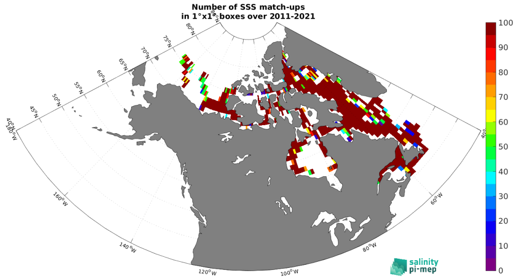
Figure 5: Number of SSS match-ups between TSG (Amundsen) SSS and the SMOS SSS L3 Arctic v4 - 9 Days (BEC) SSS product for the Global Ocean Pi-MEP region over 1^\circ \times 1^\circ boxes and for the full satellite product period.
