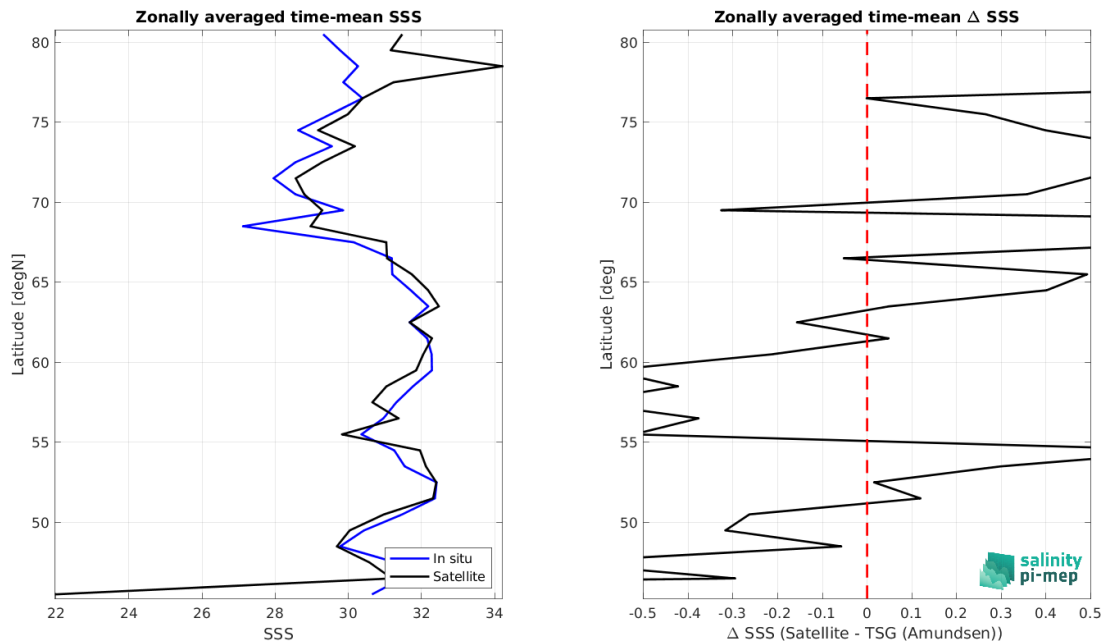
Figure 9: Left panel: Zonal mean SSS from SMOS SSS L3 Arctic v4 - 9 Days (BEC) satellite product (black) and from TSG (Amundsen) (blue). Right panel: Zonal mean of \Delta SSS (Satellite - TSG (Amundsen)) for all the collected Pi-MEP match-up pairs estimated over the full satellite product period.
