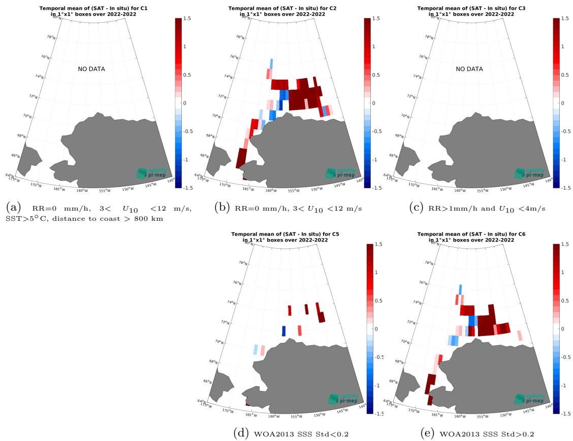
Figure 14: Temporal mean gridded over spatial boxes of size 1^\circ \times 1^\circ of \Delta SSS (SMOS SSS L3 Arctic v4 - 9 Days (BEC) - SASSIE) for 5 different subdatasets corresponding to:RR=0 mm/h, 3 < U_{10} < 12 m/s, SST>5°C, distance to coast > 800 km (a), RR=0 mm/h, 3 < U_{10} < 12 m/s (b), RR>1mm/h and U_{10} < 4 m/s (c), WOA2013 SSS Std<0.2 (d), WOA2013 SSS Std>0.2 (e).
