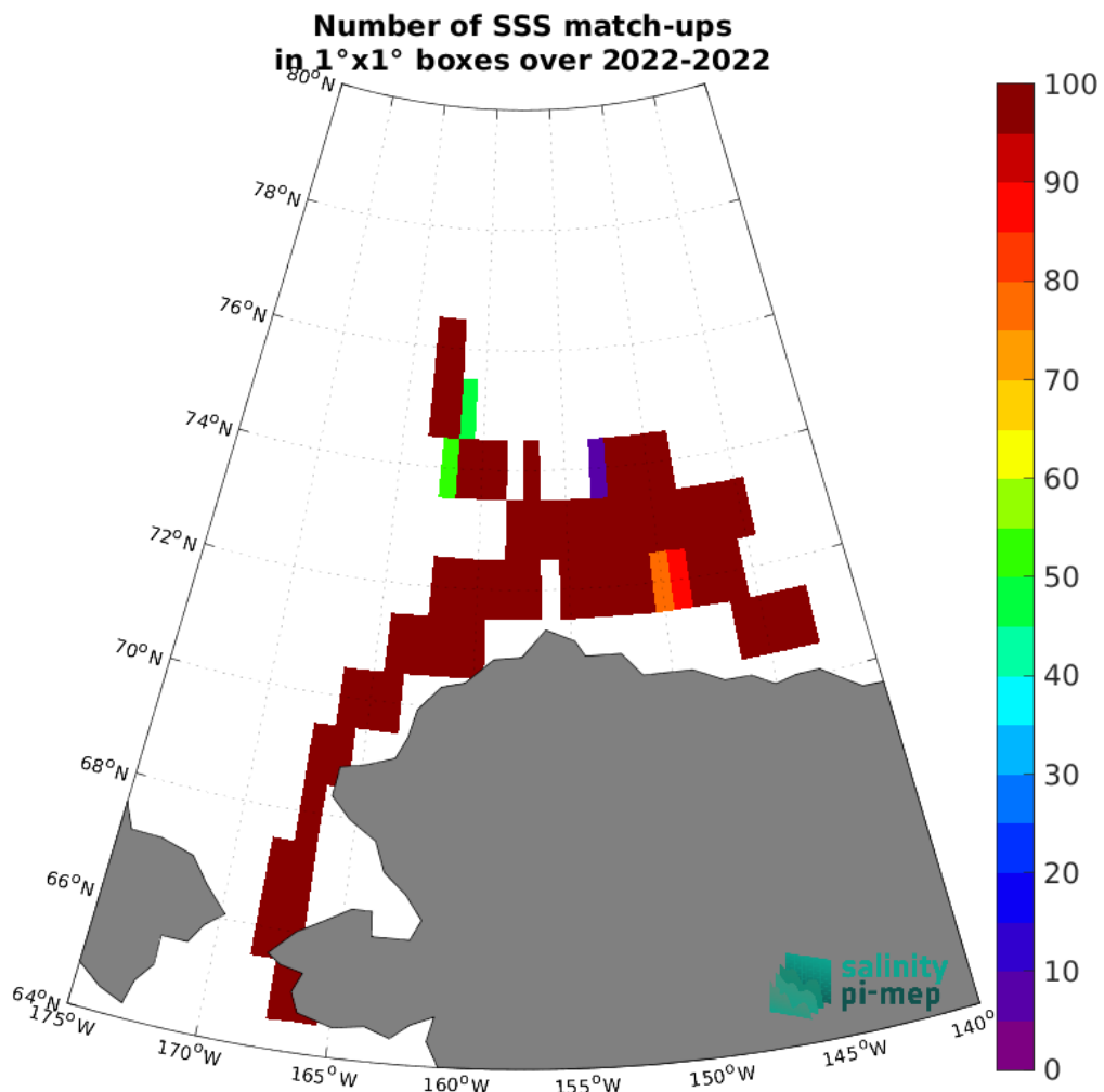
Figure 5: Number of SSS match-ups between SASSIE SSS and the SMOS SSS L3 Arctic v4 - 9 Days (BEC) SSS product for the Global Ocean Pi-MEP region over 1°x1° boxes and for the full satellite product period.
