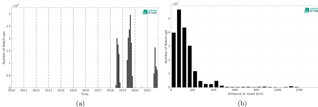
Figure 2: Number of match-ups between Saildrone and SMOS SSS L3 Arctic v4 - 9 Days (BEC) SSS as a function of time (a) and as function of the distance to coast (b) over the Global Ocean Pi-MEP region and for the full satellite product period.
