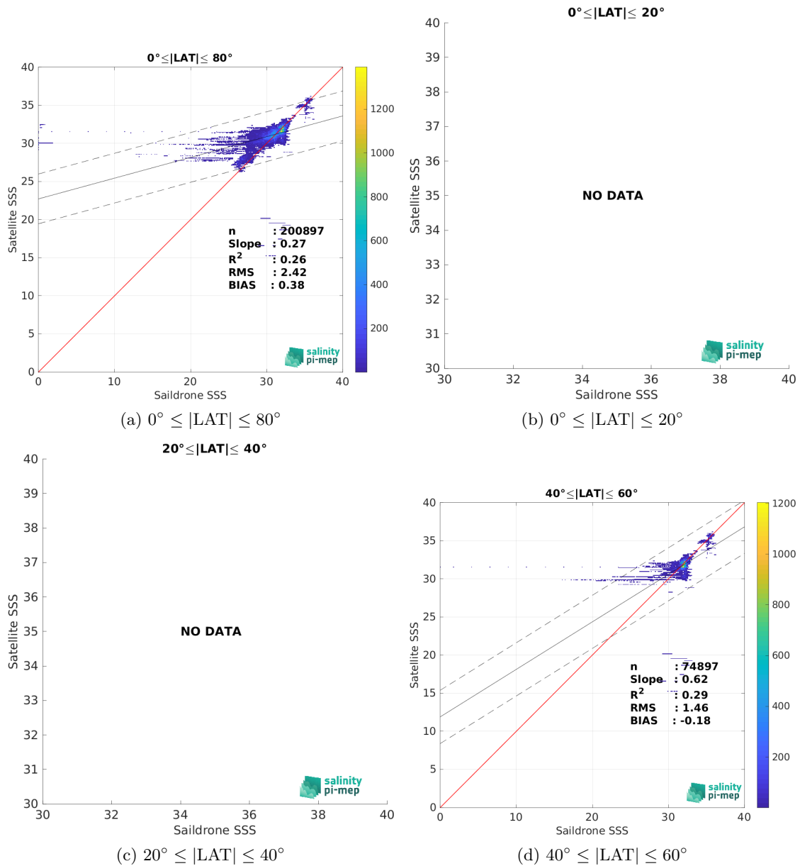
Figure 10: Contour maps of the concentration of SMOS SSS L3 Arctic v4 - 9 Days (BEC) SSS (y-axis) versus Saildrone SSS (x-axis) at match-up pairs for different latitude bands. For each plot, the red line shows x=y . The black thin and dashed lines indicate a linear fit through the data cloud and the \pm 95\% confidence levels, respectively. The number match-up pairs n , the slope and R^2 coefficient of the linear fit, the root mean square (RMS) and the mean bias between satellite and in situ data are indicated for each latitude band in each plots.
