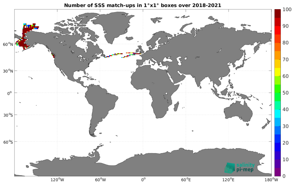
Figure 5: Number of SSS match-ups between Saildrone SSS and the SMOS SSS L3 Arctic v4 - 9 Days (BEC) SSS product for the Global Ocean Pi-MEP region over 1^\circ \times 1^\circ boxes and for the full satellite product period.
