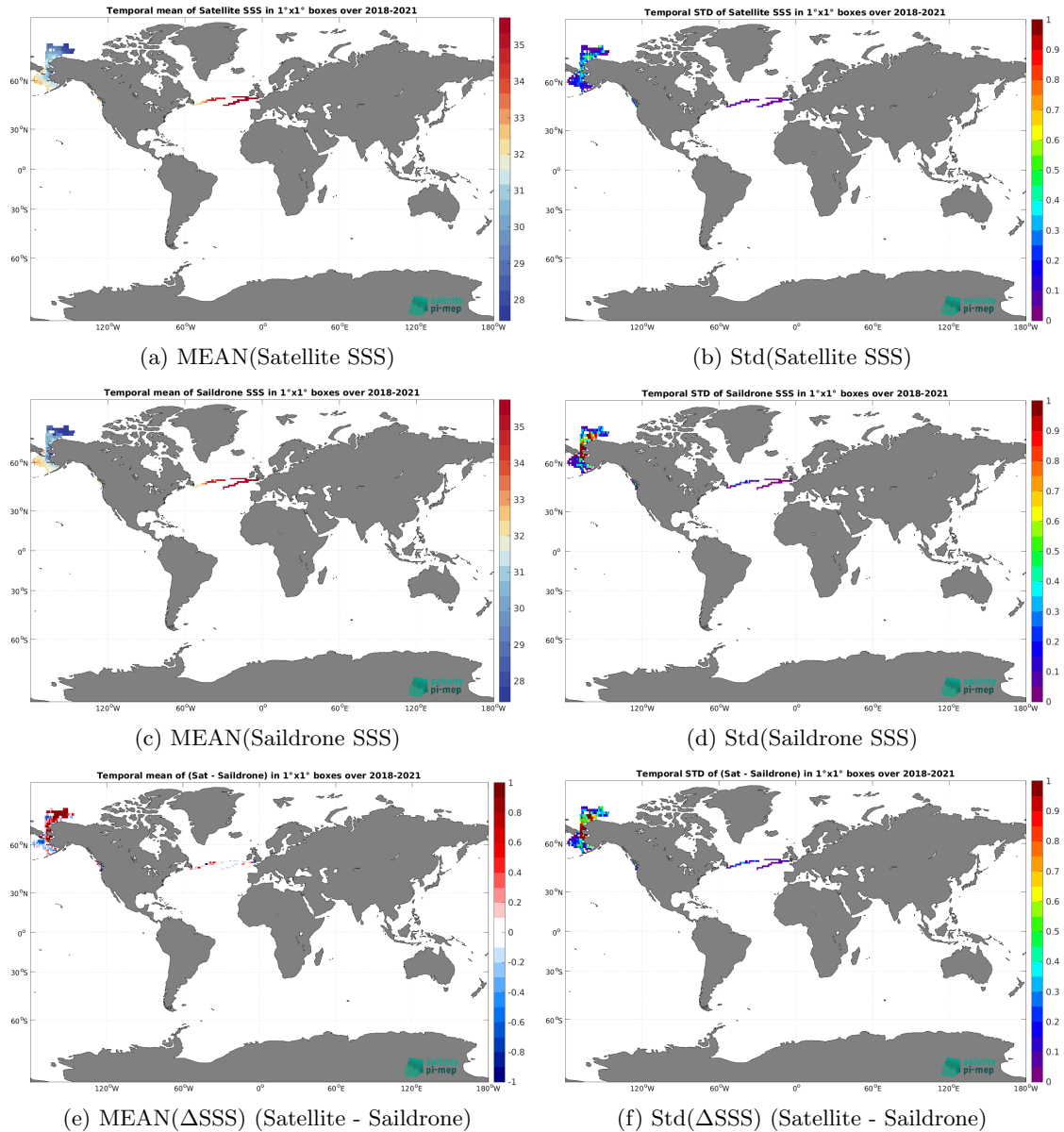
Figure 7: Temporal mean (left) and Std (right) of SSS from SMOS SSS L3 Arctic v4 - 9 Days (BEC) (top), Saildrone (middle), and of \Delta SSS (Satellite - Saildrone). Only match-up pairs are used to generate these maps.
