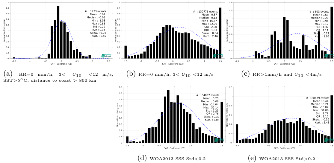
Figure 15: Normalized histogram of \Delta SSS (SMOS SSS L3 Arctic v4 - 9 Days (BEC) - Sairdrone) for 5 different subdatasets corresponding to: RR=0 mm/h, 3 < U_{10} < 12 m/s, SST > 5°C, distance to coast > 800 km (a), RR=0 mm/h, 3 < U_{10} < 12 m/s (b), RR > 1mm/h and U_{10} < 4 m/s (c), WOA2013 SSS Std < 0.2 (d), WOA2013 SSS Std > 0.2 (e).
