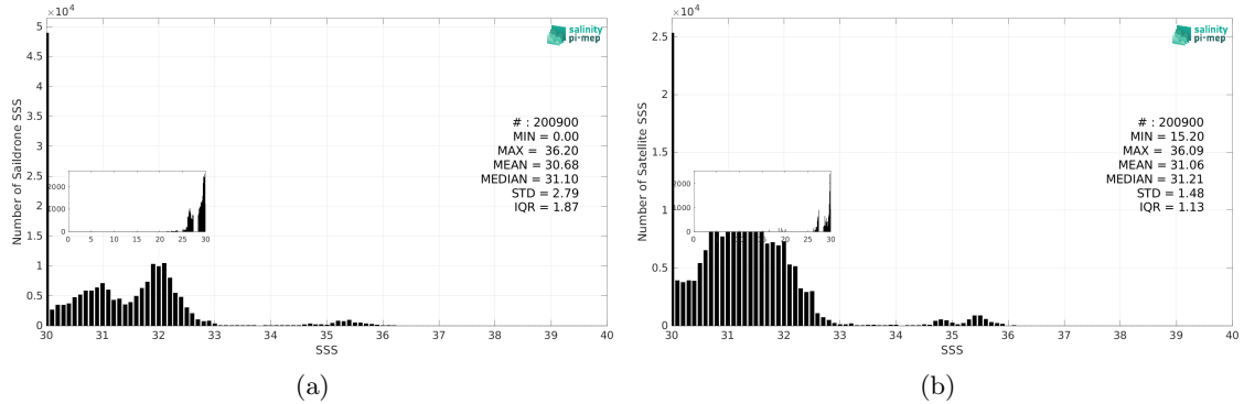
Figure 3: Histograms of SSS from Saildrone (a) and SMOS SSS L3 Arctic v4 - 9 Days (BEC) (b) considering all match-up pairs per bins of 0.1 over the Global Ocean Pi-MEP region and for the full satellite product period.
