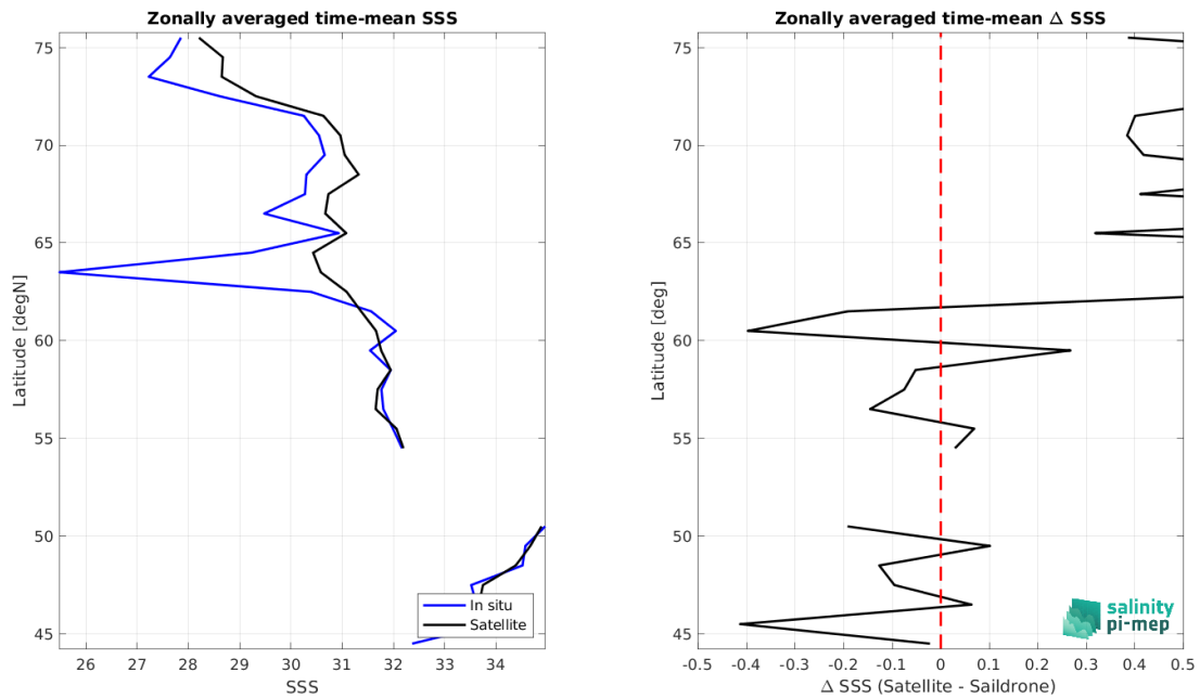
Figure 9: Left panel: Zonal mean SSS from SMOS SSS L3 Arctic v4 - 9 Days (BEC) satellite product (black) and from Sairdron (blue). Right panel: Zonal mean of \Delta SSS (Satellite - Sairdron) for all the collected Pi-MEP match-up pairs estimated over the full satellite product period.
