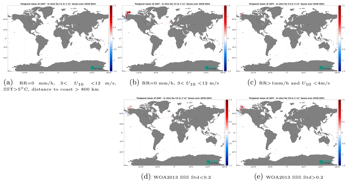
Figure 14: Temporal mean gridded over spatial boxes of size 1^\circ \times 1^\circ of \Delta SSS (SMOS SSS L3 Arctic v4 - 9 Days (BEC) - Saildrone) for 5 different subdatasets corresponding to:RR=0 mm/h, 3 < U_{10} < 12 m/s, SST > 5^\circ\text{C} , distance to coast > 800 km (a), RR=0 mm/h, 3 < U_{10} < 12 m/s (b), RR > 1 mm/h and U_{10} < 4 m/s (c), WOA2013 SSS Std < 0.2 (d), WOA2013 SSS Std > 0.2 (e).
