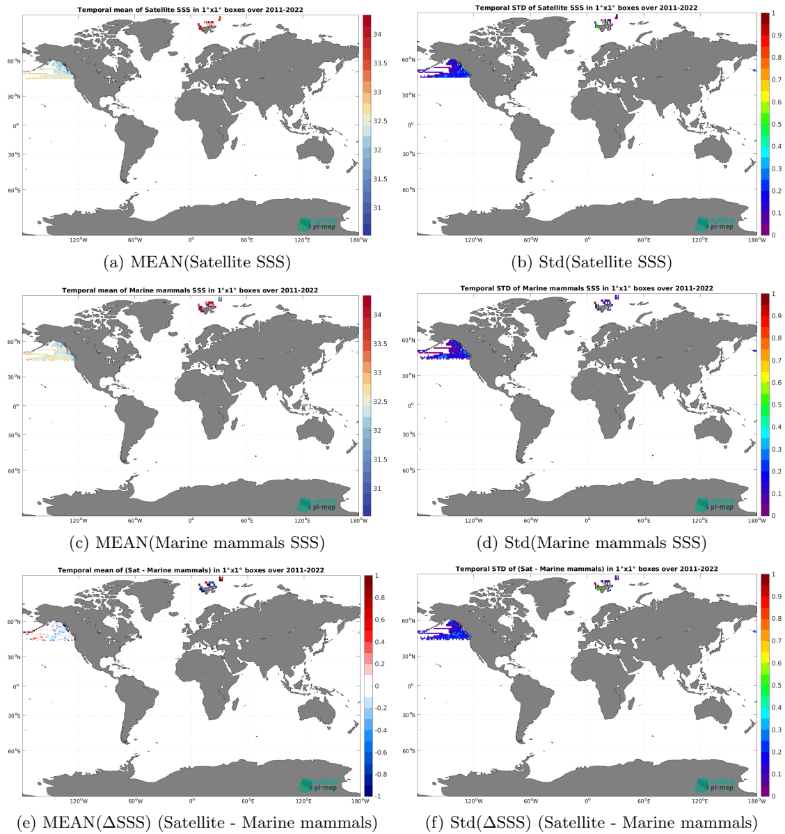
Figure 7: Temporal mean (left) and Std (right) of SSS from SMOS SSS L3 Arctic v4 - 9 Days (BEC) (top), Marine mammals (middle), and of \Delta SSS (Satellite - Marine mammals). Only match-up pairs are used to generate these maps.
