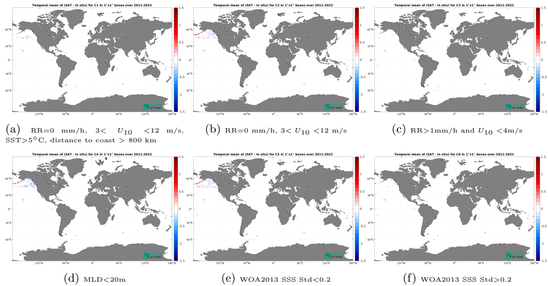
Figure 14: Temporal mean gridded over spatial boxes of size 1^\circ \times 1^\circ of \Delta SSS (SMOS SSS L3 Arctic v4 - 9 Days (BEC) - Marine mammals) for 6 different subdatasets corresponding to:RR=0 mm/h, 3 < U_{10} < 12 m/s, SST >5^\circ C, distance to coast > 800 km (a), RR=0 mm/h, 3 < U_{10} < 12 m/s (b), RR >1 mm/h and U_{10} < 4 m/s (c),MLD <20 m (d),WOA2013 SSS Std <0.2 (e),WOA2013 SSS Std >0.2 (f).
