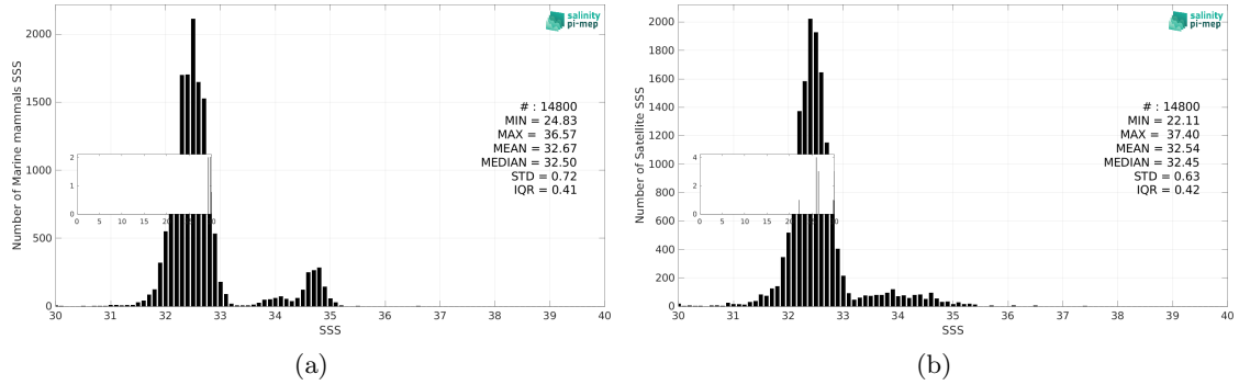
Figure 3: Histograms of SSS from Marine mammals (a) and SMOS SSS L3 Arctic v4 - 9 Days (BEC) (b) considering all match-up pairs per bins of 0.1 over the Global Ocean Pi-MEP region and for the full satellite product period.
