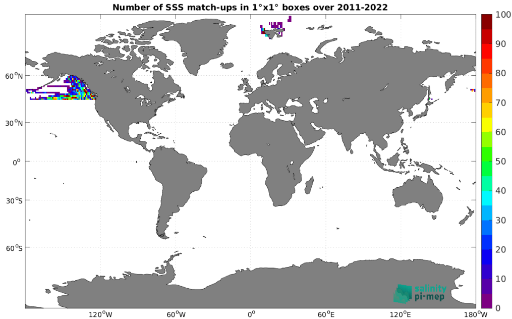
Figure 5: Number of SSS match-ups between Marine mammals SSS and the SMOS SSS L3 Arctic v4 - 9 Days (BEC) SSS product for the Global Ocean Pi-MEP region over 1°x1° boxes and for the full satellite product period.
