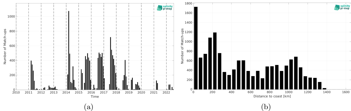
Figure 2: Number of match-ups between Marine mammals and SMOS SSS L3 Arctic v4 - 9 Days (BEC) SSS as a function of time (a) and as function of the distance to coast (b) over the Global Ocean Pi-MEP region and for the full satellite product period.
