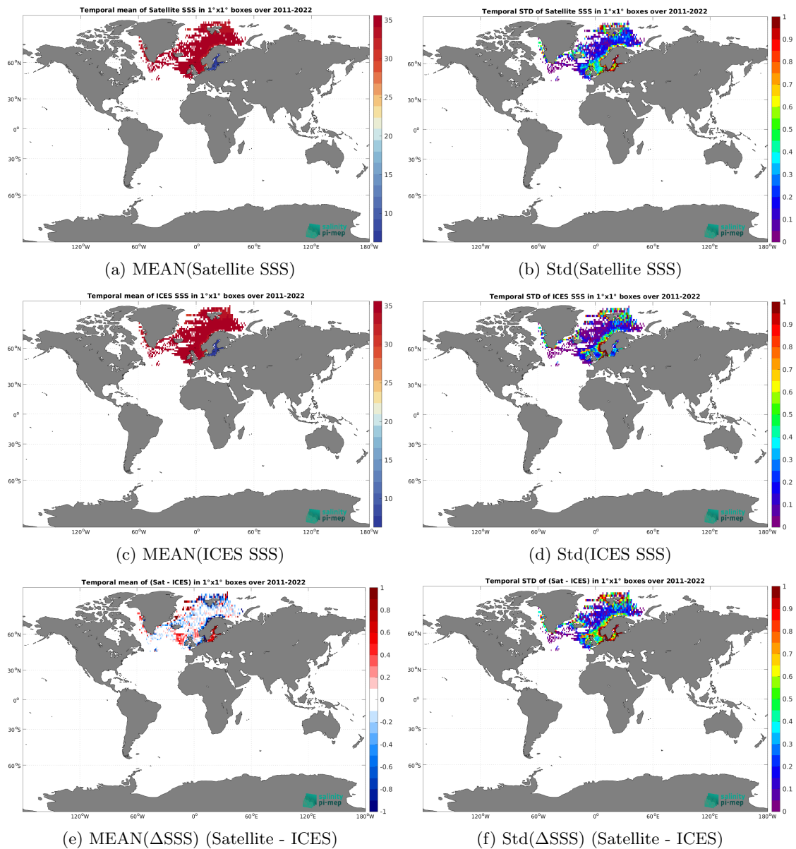
Figure 7: Temporal mean (left) and Std (right) of SSS from SMOS SSS L3 Arctic v4 - 9 Days (BEC) (top), ICES (middle), and of \Delta SSS (Satellite - ICES). Only match-up pairs are used to generate these maps.
