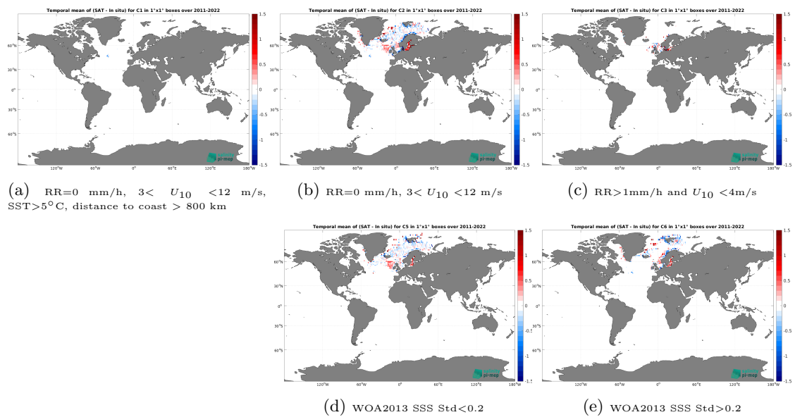
Figure 14: Temporal mean gridded over spatial boxes of size 1^\circ \times 1^\circ of \Delta SSS (SMOS SSS L3 Arctic v4 - 9 Days (BEC) - ICES) for 5 different subdatasets corresponding to:RR=0 mm/h, 3 < U_{10} < 12 m/s, SST > 5^\circ\text{C} , distance to coast > 800 km (a), RR=0 mm/h, 3 < U_{10} < 12 m/s (b), RR > 1 mm/h and U_{10} < 4 m/s (c), WOA2013 SSS Std < 0.2 (d), WOA2013 SSS Std > 0.2 (e).
