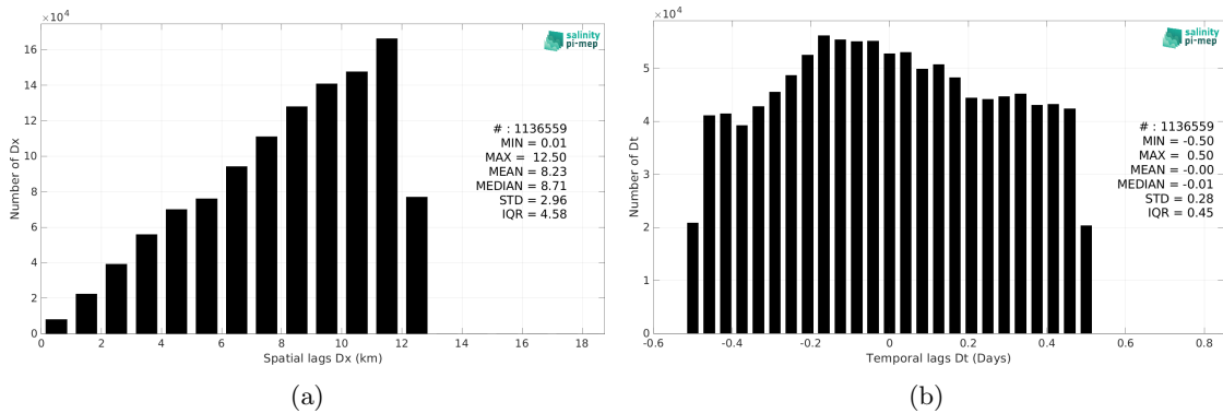
Figure 6: Histograms of the spatial (a) and temporal (b) lags between the location/time of the ICES measurement and the date of the corresponding SMOS SSS L3 Arctic v4 - 9 Days (BEC) SSS pixel.
