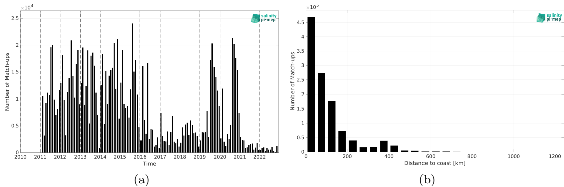
Figure 2: Number of match-ups between ICES and SMOS SSS L3 Arctic v4 - 9 Days (BEC) SSS as a function of time (a) and as function of the distance to coast (b) over the Global Ocean Pi-MEP region and for the full satellite product period.
