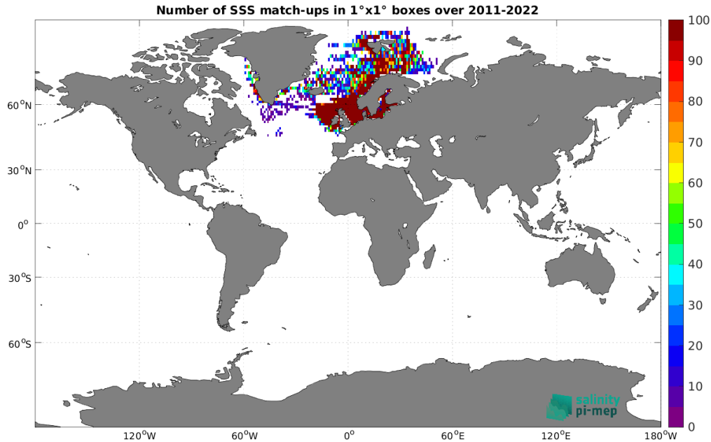
Figure 5: Number of SSS match-ups between ICES SSS and the SMOS SSS L3 Arctic v4 - 9 Days (BEC) SSS product for the Global Ocean Pi-MEP region over 1^\circ \times 1^\circ boxes and for the full satellite product period.
