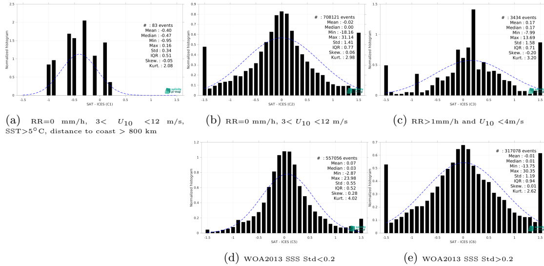
Figure 15: Normalized histogram of \Delta SSS (SMOS SSS L3 Arctic v4 - 9 Days (BEC) - ICES) for 5 different subdatasets corresponding to: RR=0 mm/h, 3 < U_{10} < 12 m/s, SST>5°C, distance to coast > 800 km (a), RR=0 mm/h, 3 < U_{10} < 12 m/s (b), RR>1mm/h and U_{10} < 4 m/s (c), WOA2013 SSS Std<0.2 (d), WOA2013 SSS Std>0.2 (e).
