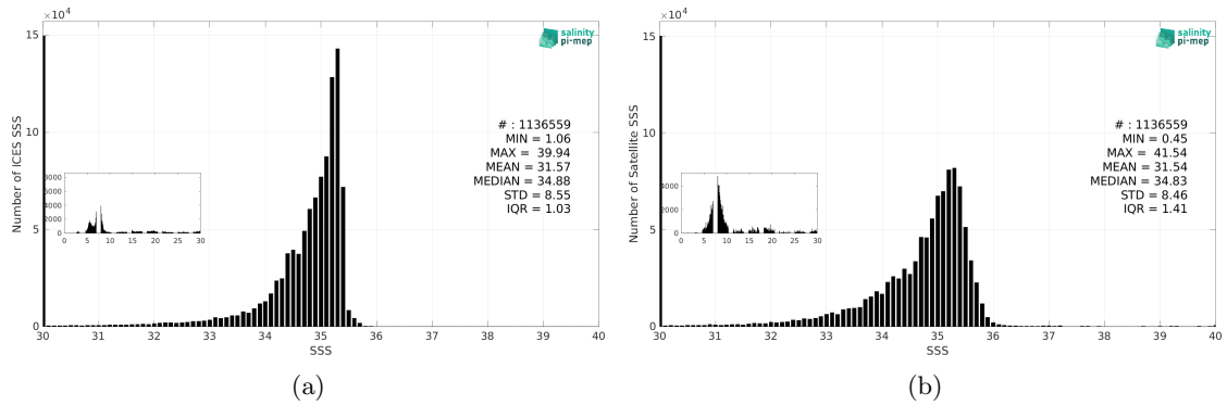
Figure 3: Histograms of SSS from ICES (a) and SMOS SSS L3 Arctic v4 - 9 Days (BEC) (b) considering all match-up pairs per bins of 0.1 over the Global Ocean Pi-MEP region and for the full satellite product period.
