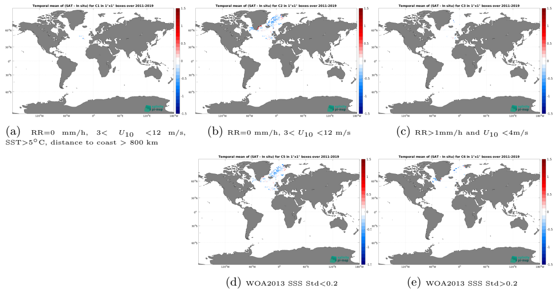
Figure 13: Temporal mean gridded over spatial boxes of size 1^\circ \times 1^\circ of \Delta SSS (SMOS SSS L3 Arctic v4 - 9 Days (BEC) - Surface drifters) for 5 different subdatasets corresponding to:RR=0 mm/h, 3 < U_{10} < 12 m/s, SST > 5^\circ\text{C} , distance to coast > 800 km (a), RR=0 mm/h, 3 < U_{10} < 12 m/s (b), RR > 1 mm/h and U_{10} < 4 m/s (c), WOA2013 SSS Std < 0.2 (d), WOA2013 SSS Std > 0.2 (e).
