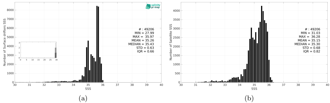
Figure 3: Histograms of SSS from Surface drifters (a) and SMOS SSS L3 Arctic v4 - 9 Days (BEC) (b) considering all match-up pairs per bins of 0.1 over the Global Ocean Pi-MEP region and for the full satellite product period.
