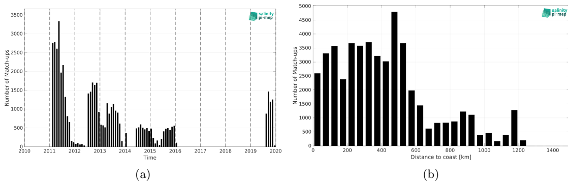
Figure 2: Number of match-ups between Surface drifters and SMOS SSS L3 Arctic v4 - 9 Days (BEC) SSS as a function of time (a) and as function of the distance to coast (b) over the Global Ocean Pi-MEP region and for the full satellite product period.
