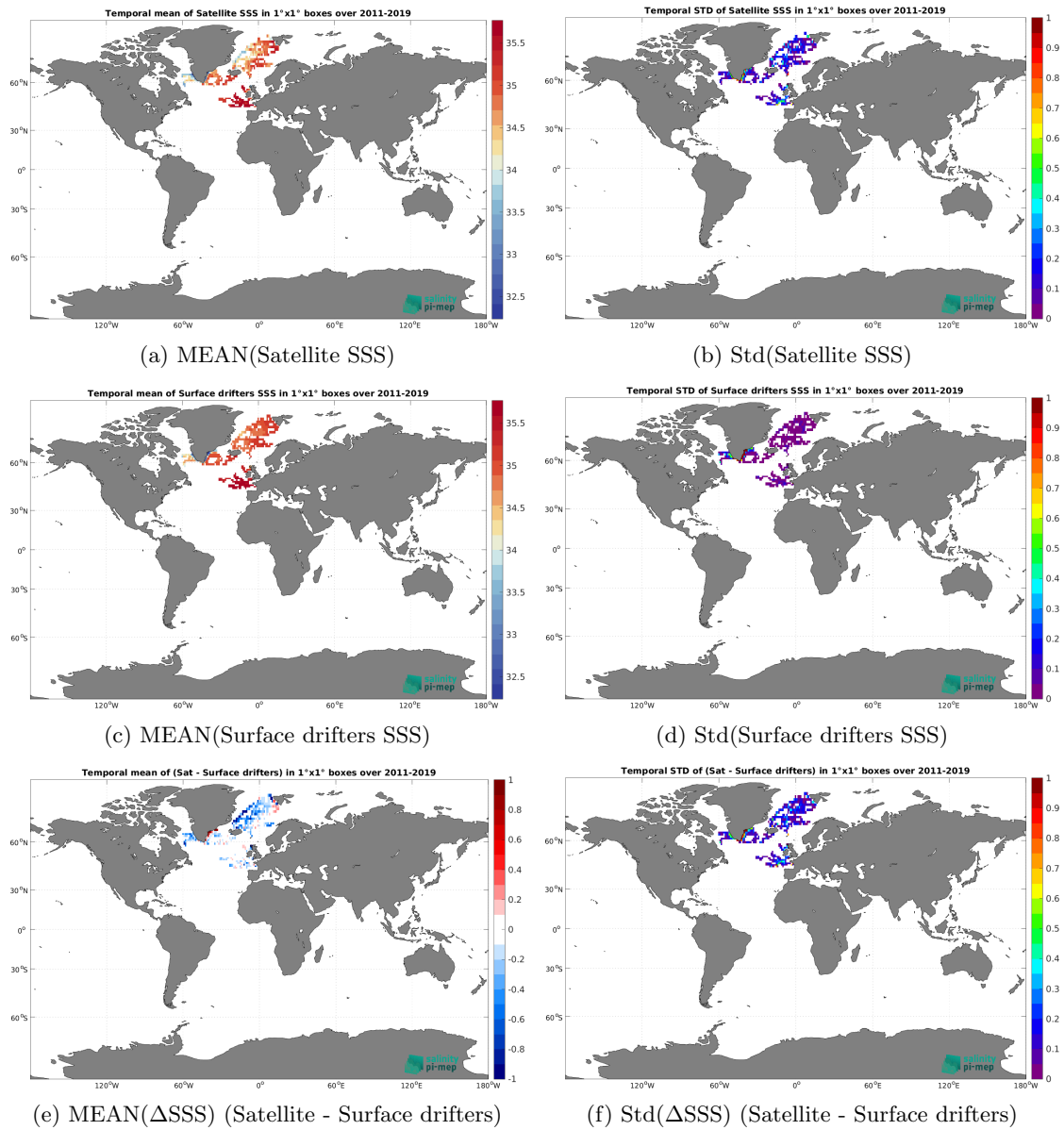
Figure 6: Temporal mean (left) and Std (right) of SSS from SMOS SSS L3 Arctic v4 - 9 Days (BEC) (top), Surface drifters (middle), and of \Delta SSS (Satellite - Surface drifters). Only match-up pairs are used to generate these maps.
