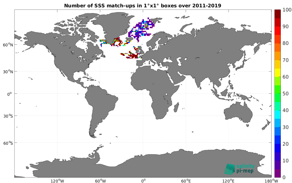
Figure 4: Number of SSS match-ups between Surface drifters SSS and the SMOS SSS L3 Arctic v4 - 9 Days (BEC) SSS product for the Global Ocean Pi-MEP region over 1^\circ \times 1^\circ boxes and for the full satellite product period.
