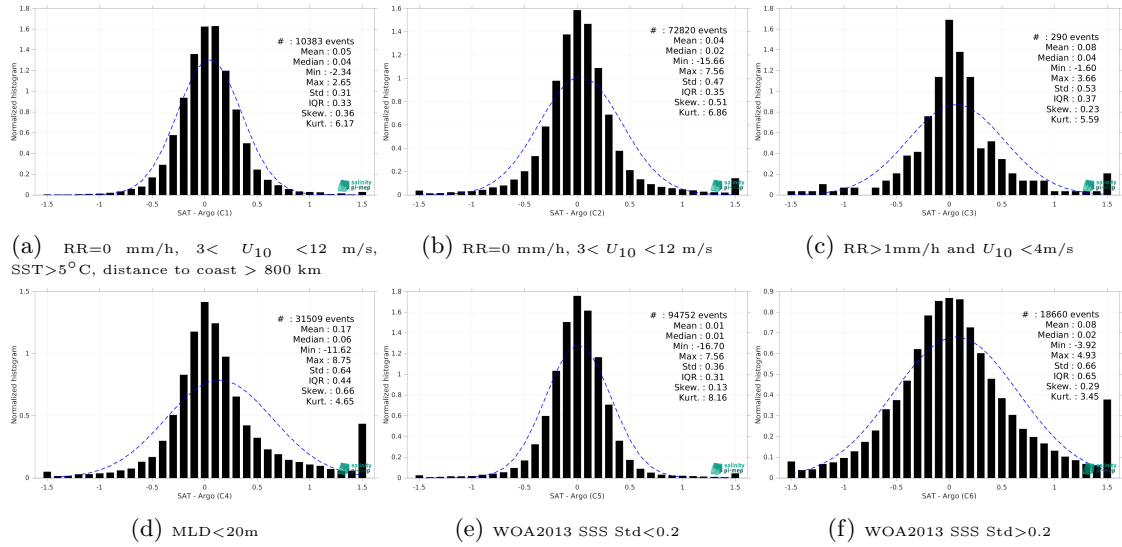
Figure 15: Normalized histogram of \Delta SSS (SMOS SSS L3 Arctic v4 - 9 Days (BEC) - Argo) for 6 different subdatasets corresponding to: RR=0 mm/h, 3 < U_{10} < 12 m/s, SST > 5°C, distance to coast > 800 km (a), RR=0 mm/h, 3 < U_{10} < 12 m/s (b), RR > 1mm/h and U_{10} < 4 m/s (c), MLD < 20m (d), WOA2013 SSS Std < 0.2 (e), WOA2013 SSS Std > 0.2 (f).
